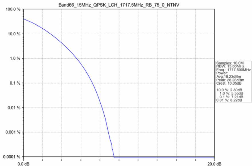
Band66_15MHz_QPSK_LCH_1717.5MHz_RB_75_0_NTNV
