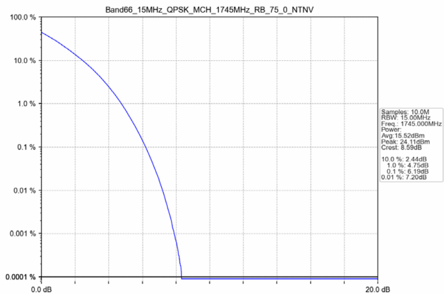
Band66_15MHz_QPSK_MCH_1745MHz_RB_75_0_NTNV
