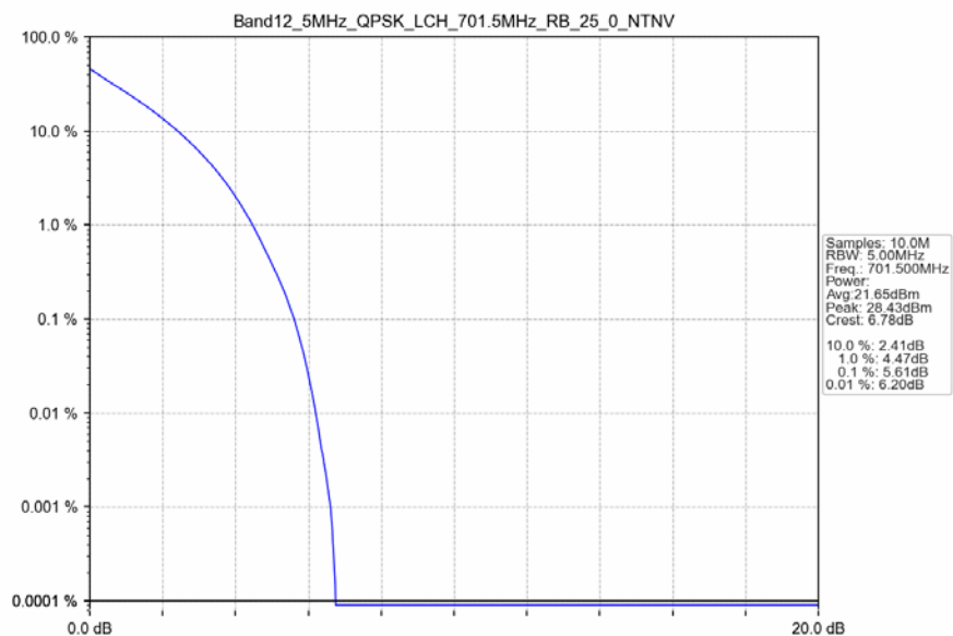
Band12_5MHz_QPSK_LCH_701.5MHz_RB_25_0_NTNV
