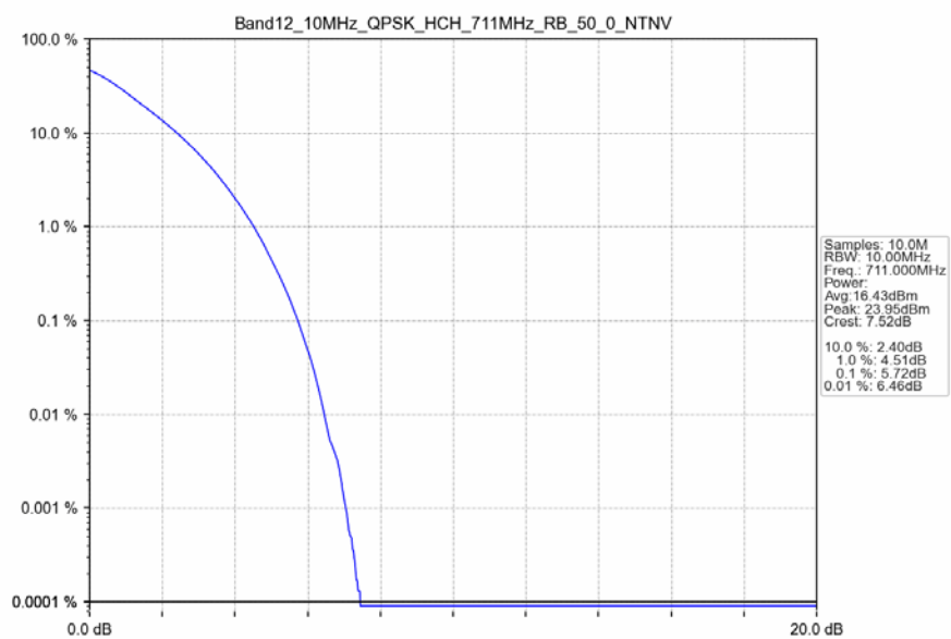
Band12_10MHz_QPSK_HCH_711MHz_RB_50_0_NTNV
