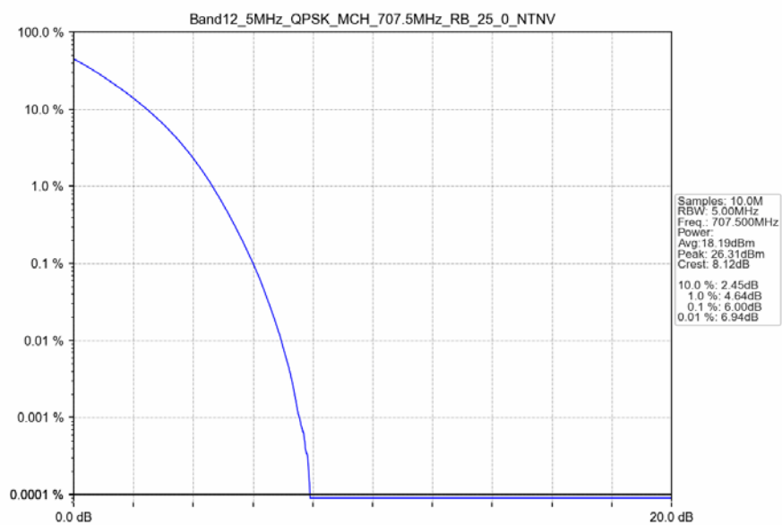
Band12_5MHz_QPSK_MCH_707.5MHz_RB_25_0_NTNV
