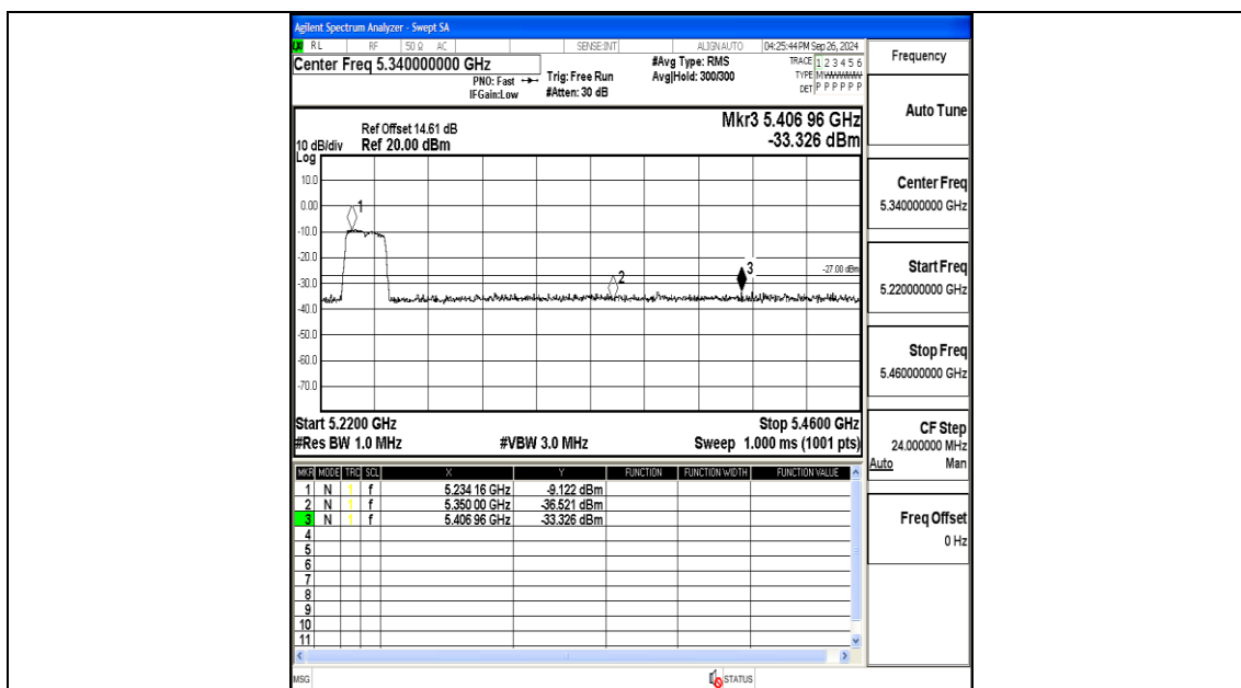
11AC20MIMO-Ant1-5240-PASS
