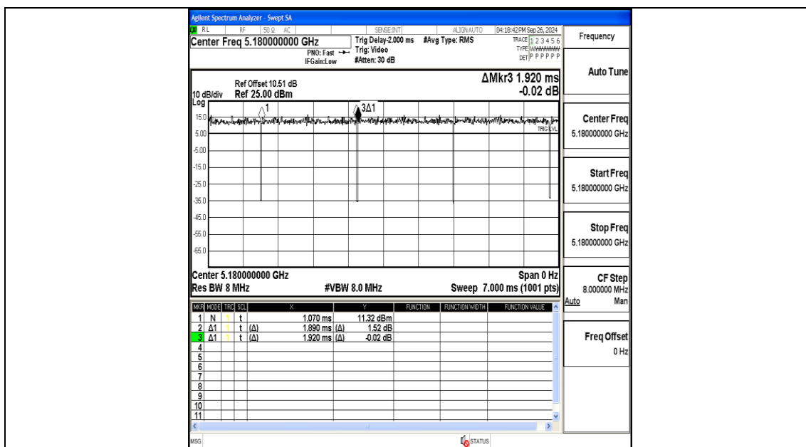
NTNV-11AC20MIMO-Ant2-5180
