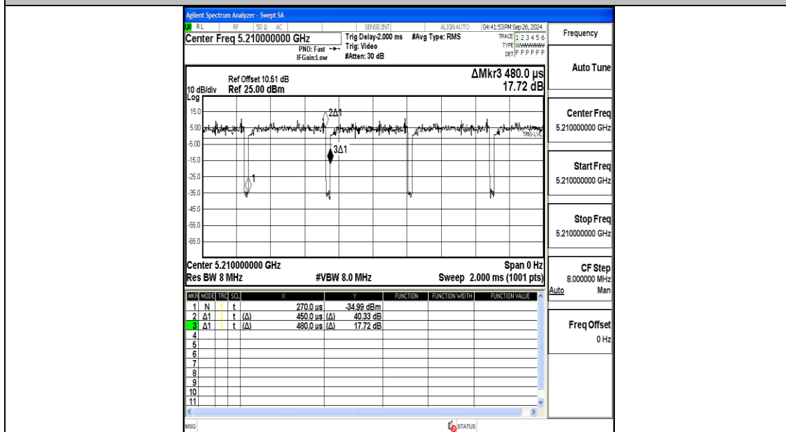
NTNV-11AC80MIMO-Ant2-5210
