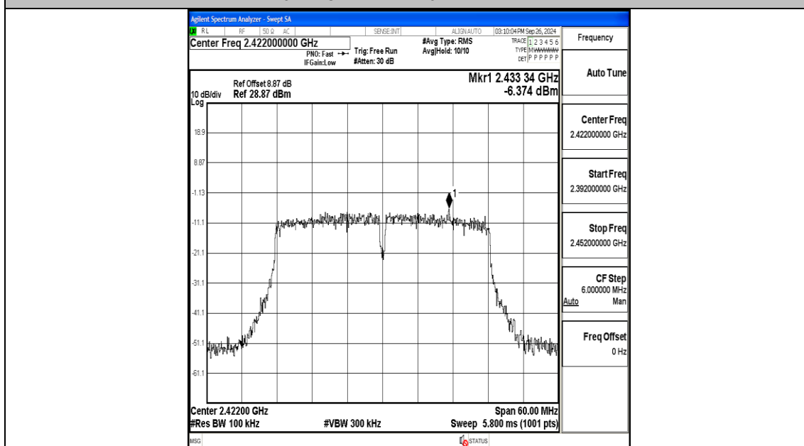
11N40MIMO-Ant2-2422-0~Reference-PASS
