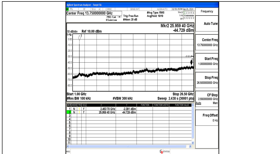
11G-Ant2-2462-1000~26500-PASS
