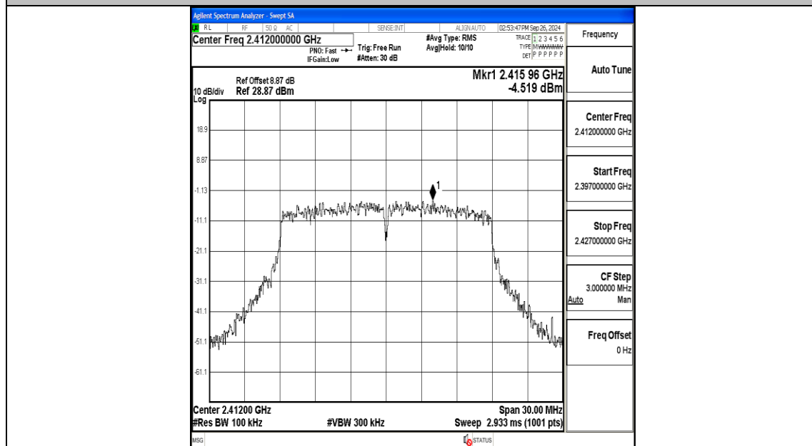
11N20MIMO-Ant2-2412-0~Reference-PASS
