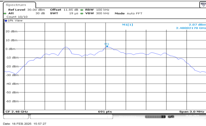
SRD 2.4G_Ant1_2480_0-Reference
