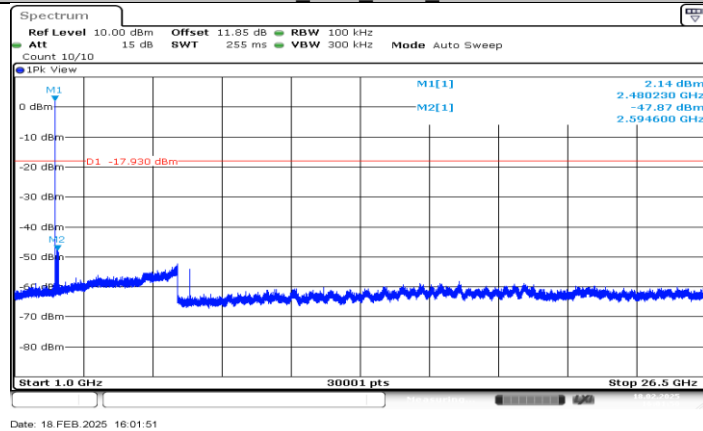
SRD 2.4G_Ant1_2480_1000-26500
