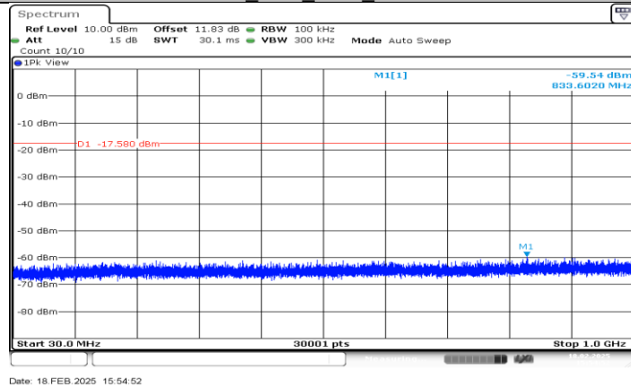
SRD 2.4G_Ant1_2441_30-1000
