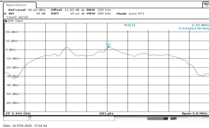
SRD 2.4G_Ant1_2441_0-Reference
