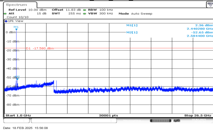
SRD 2.4G_Ant1_2441_1000-26500
