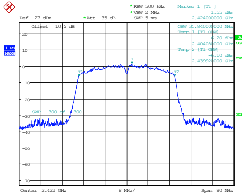
802.11n40_2422MHz 35.840MHz
