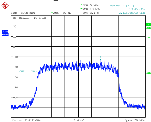
802.11n20_2412MHz -13.45dBm/3kHz
