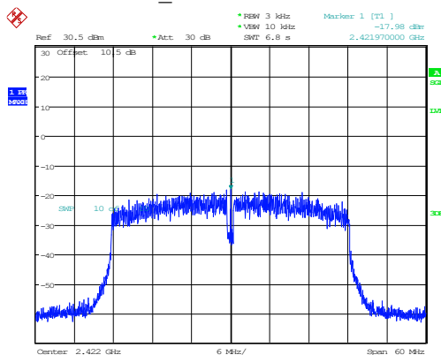
802.11n40_2422MHz -17.98dBm/3kHz
