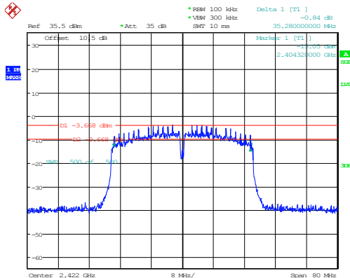
802.11n40_2422MHz 35.280MHz
