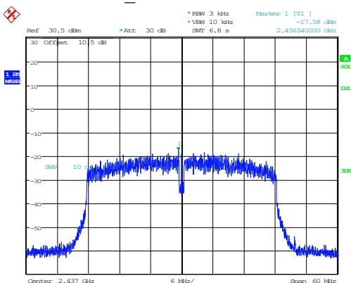
802.11n40_2437MHz -17.58dBm/3kHz
