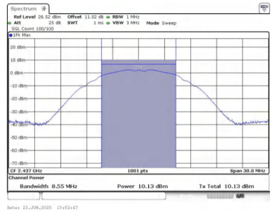
Conducted Output Power IEEE 802.11b_Channel 6_Antenna 0
