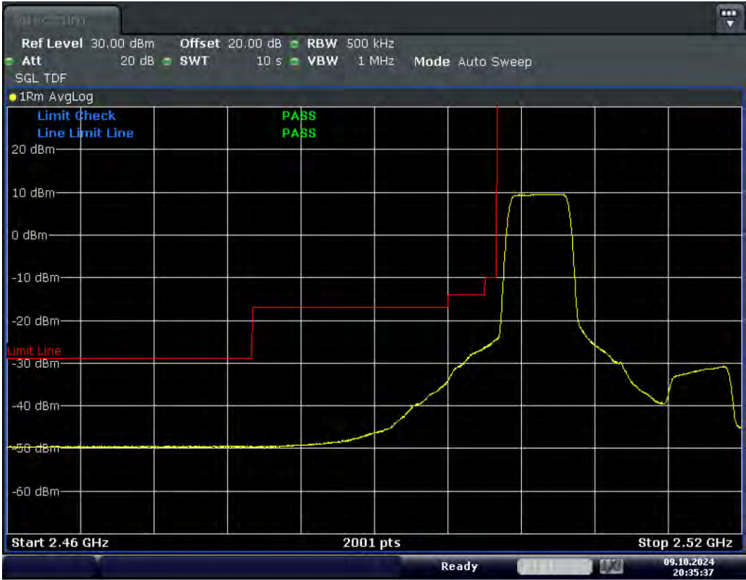
Band7-20-2510-16QAM-27#LOW
