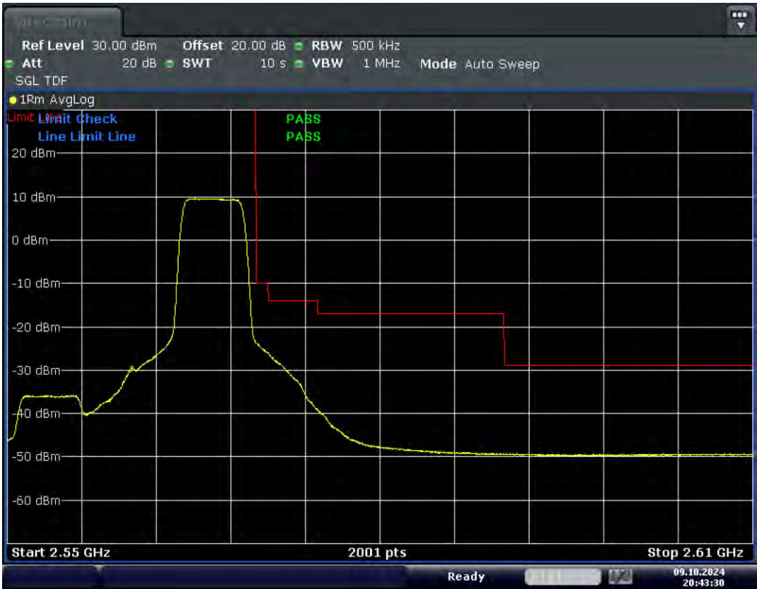
Band7-20-2560-16QAM-27#HIGH
