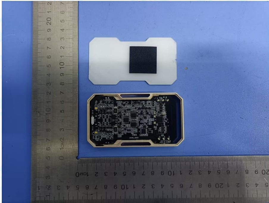
Photo 10 Internal of PCB & Battery
