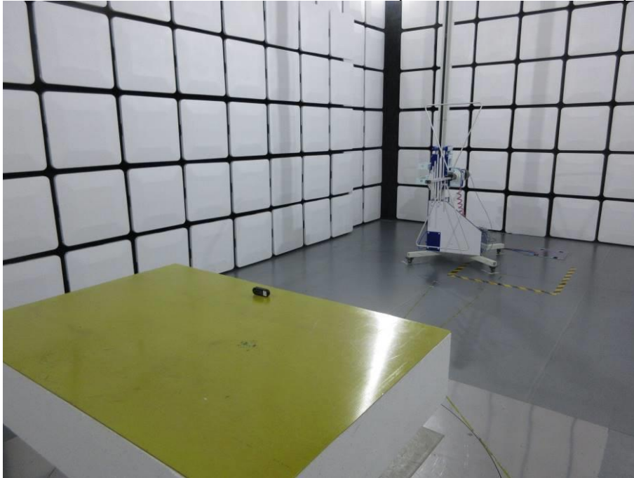
RADIATED RF MEASUREMENT SETUP (30MHz ~ 1 GHz - Y axis)
