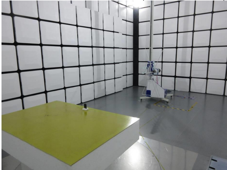
RADIATED RF MEASUREMENT SETUP (30MHz ~ 1 GHz - Z axis)
