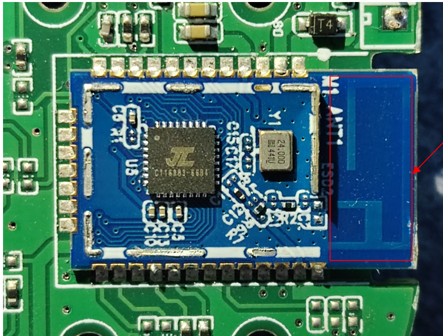
BT/BLE Antenna
