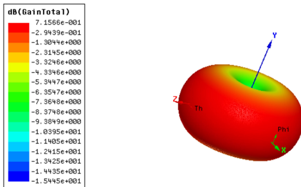
Figure 4 antenna gain
