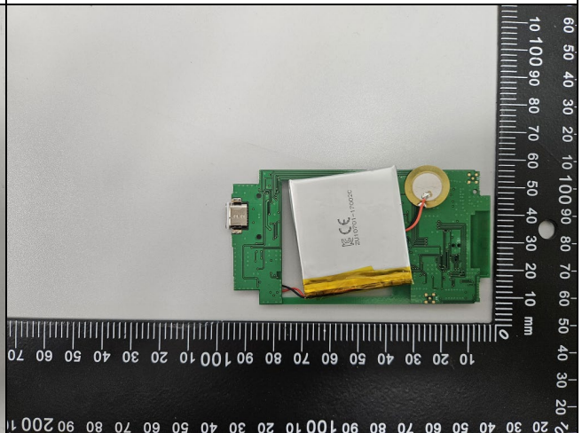
Chip Antenna for LE 1 Mbps, ANT+
