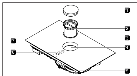
Fig. 6.1 Structure
