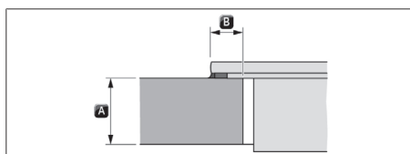
Fig. 11.11 Overlay dimensions for surface mounting
