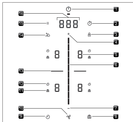
Fig. 6.3 Operating panel
