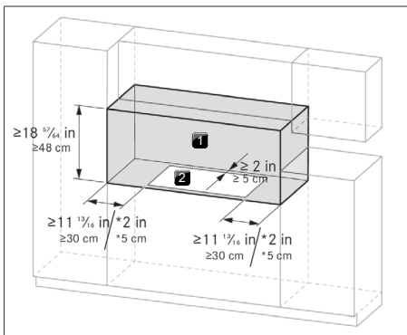
Fig. 11.3 Distance requise
