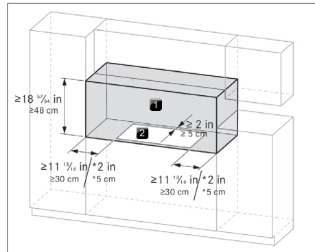
Fig. 11.3 Required clearance
