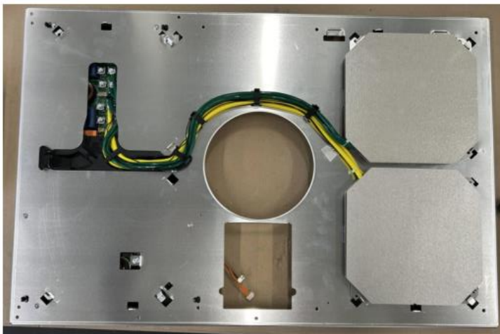
Induction coil support with all coils
