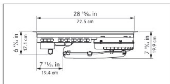
Fig. 5.2 Appliance dimensions front view
