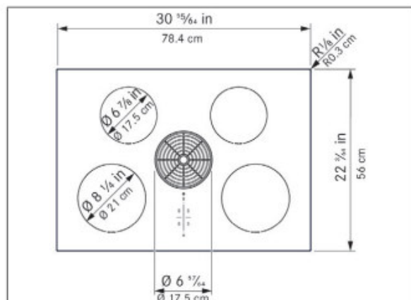
Fig. 5.1 Appliance dimensions top view
