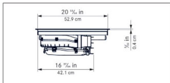
Fig. 5.3 Appliance dimensions side view
