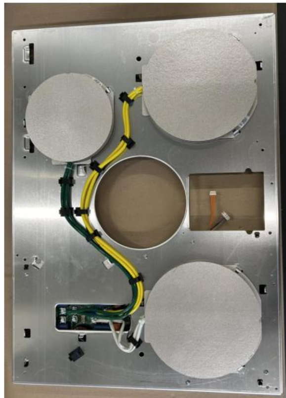
Induction coil support with all coils
