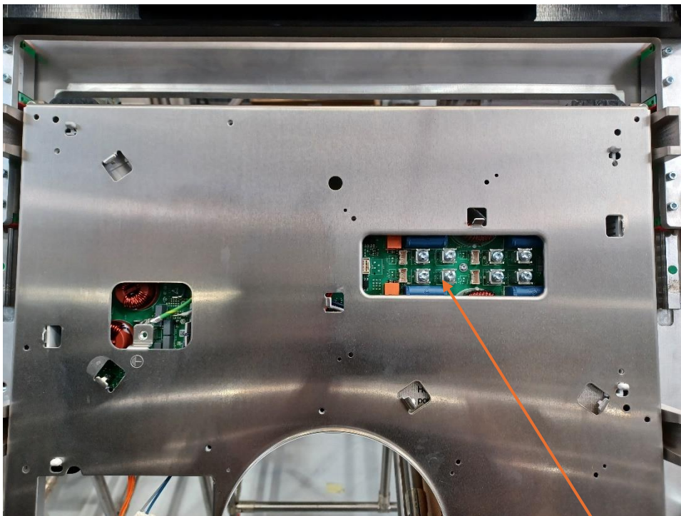
Grounding at the induction coil support
