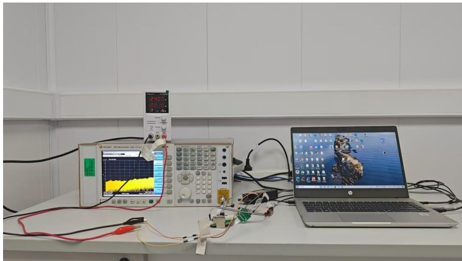
Conducted Test-BT
