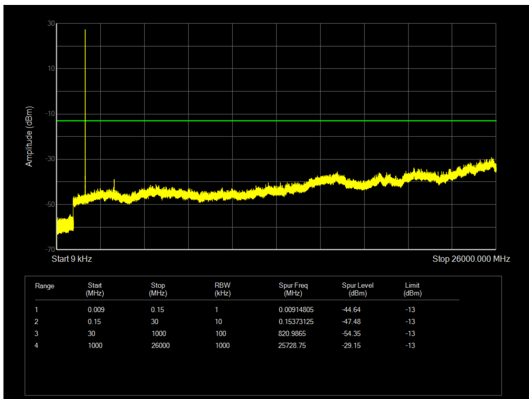
Band66 QAM16 BW=1.4MHz Channel=131979 RB Size=6 Position=#0
