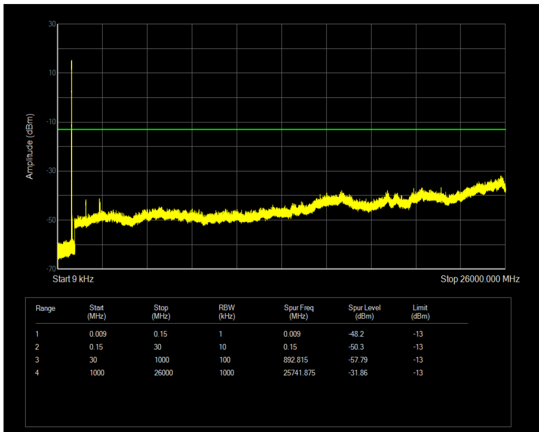
Band18(824-830) QPSK BW=5MHz Channel=23975 RB Size=25 Position=#0
