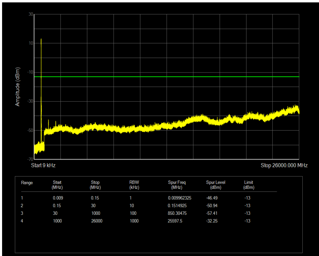
Band18(824-830) QPSK BW=5MHz Channel=23965 RB Size=25 Position=#0
