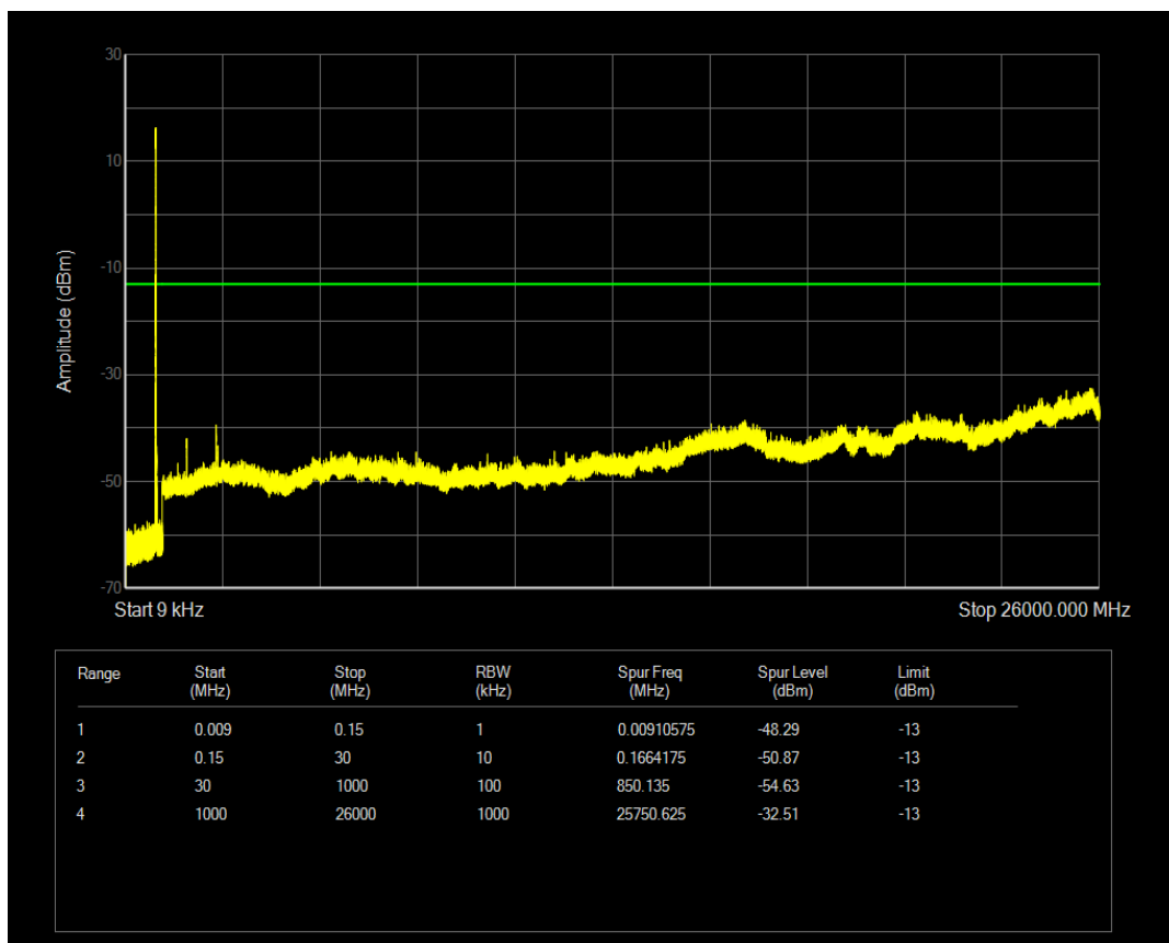
Band18(824-830) QAM16 BW=5MHz Channel=23975 RB Size=25 Position=#0
