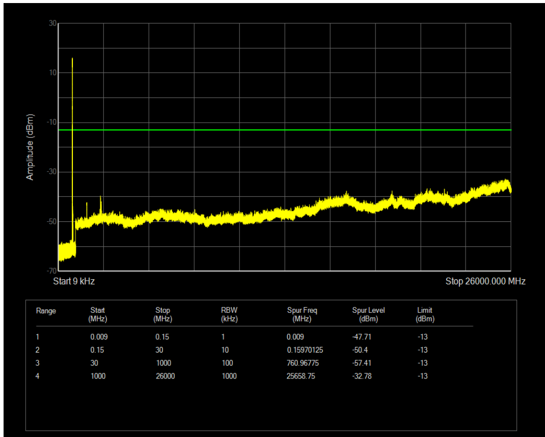
Band18(824-830) QAM16 BW=5MHz Channel=23965 RB Size=25 Position=#0
