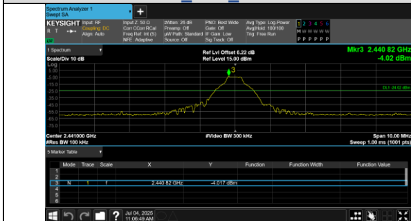
Out Of Band Emission GFSK_DH5_Channel 39
