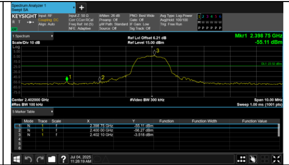
Out Of Band Emission \pi/4 DQPSK_2-DH5_Channel 0
