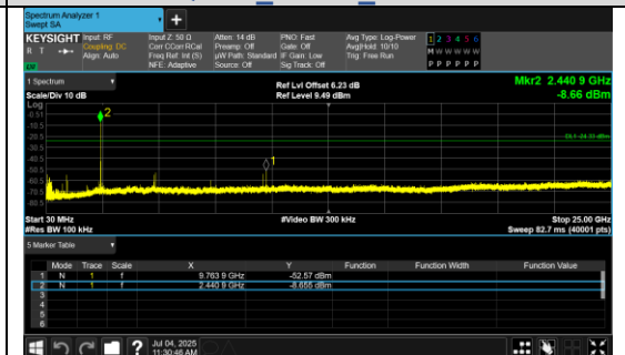
30.0 MHz - 25000.0 MHz \pi/4 DQPSK_2-DH5_Channel 39
