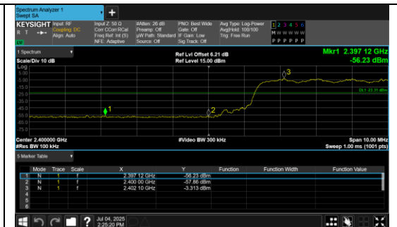
Out Of Band Emission(Left) pi/4DQPSK_2-DH5_Channel Hopping
