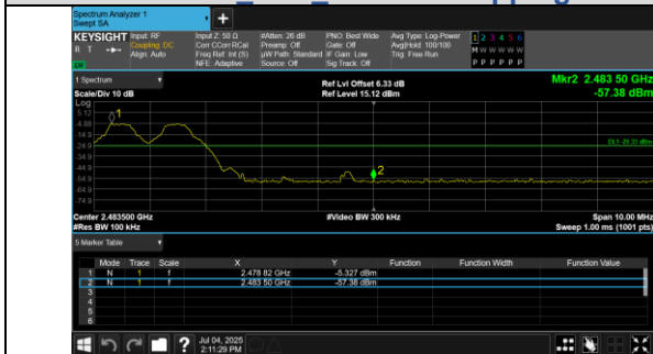
Out Of Band Emission(Right) GFSK_DH5_Channel Hopping
