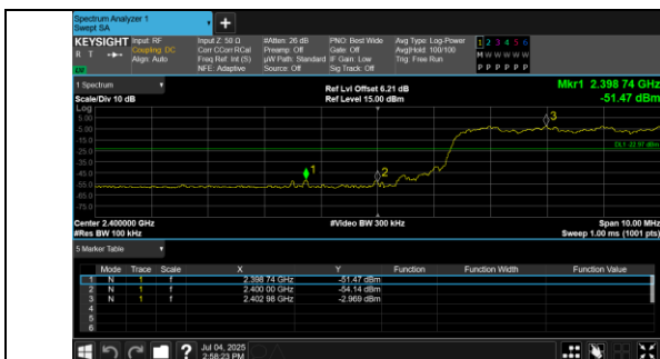
Out Of Band Emission(Left) 8DPSK_3-DH5_Channel Hopping
