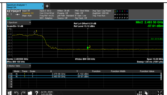
Out Of Band Emission(Right) 8DPSK_3-DH5_Channel Hopping
