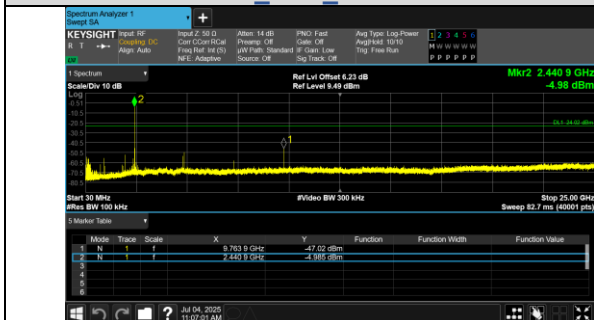
30.0 MHz - 25000.0 MHz GFSK_DH5_Channel 39
