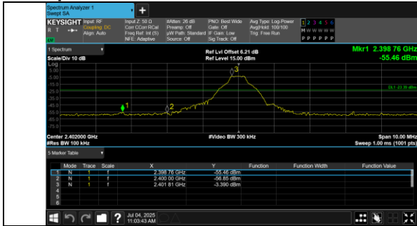
Out Of Band Emission GFSK_DH5_Channel 0
