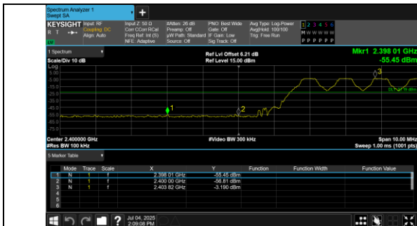
Out Of Band Emission(Left) GFSK_DH5_Channel Hopping
