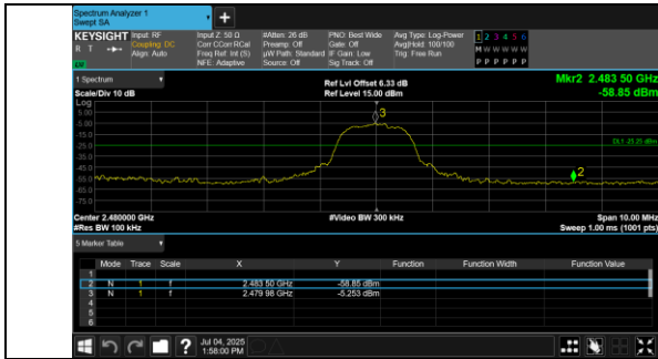
Out Of Band Emission 8DPSK_3-DH5_Channel 78
