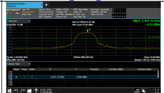
Out Of Band Emission \pi/4 DQPSK_2-DH5_Channel 39
