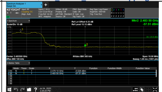
Out Of Band Emission(Right) pi/4DQPSK_2-DH5_Channel Hopping
