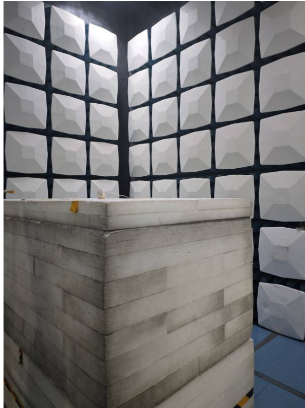
Radiated Emission Above 140-220GHz View
