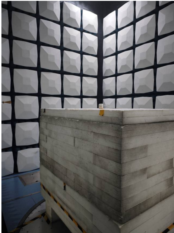
Radiated Emission Above 60-90GHz View
