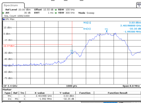
BLE_2M_Low_Channel
