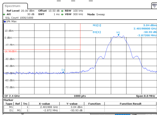
BLE_1M_Low_Channel
