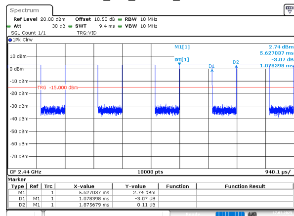
BLE_2M_Middle_Channel
