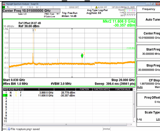
12A_n77(3700-3980MHz) (30MHz-20GHz) 60M DFT-s-OFDM QPSK Inner_1RB_Right Mid
