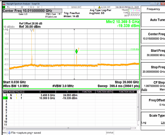
12A_n77(3450-3550MHz) (30MHz-20GHz) 90M DFT-s-OFDM QPSK Inner_1RB_Left Mid
