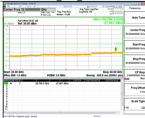
12A_n77(3700-3980MHz) (20GHz-40GHz) 40M DFT-s-OFDM QPSK Inner_1RB_Right Mid
