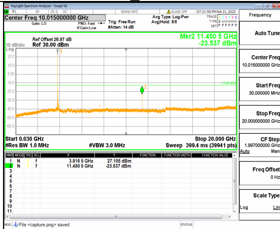
12A_n77(3700-3980MHz) (30MHz-20GHz) 50M DFT-s-OFDM QPSK Inner_1RB_Left_Mid
