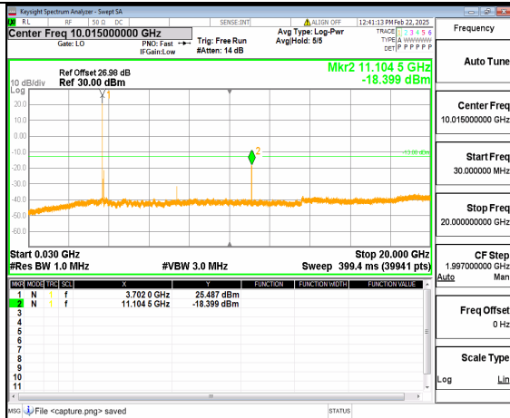
12A_n77(3700-3980MHz) (30MHz-20GHz) 70M DFT-s-OFDM QPSK Inner_1RB_Left Low
