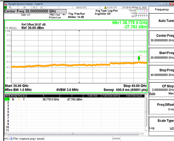
12A_n77(3700-3980MHz) (20GHz-40GHz) 30M DFT-s-OFDM QPSK Outer_Full_Mid
