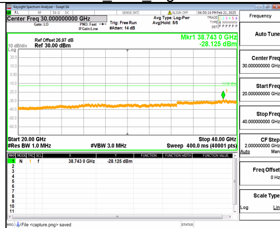
12A_n77(3700-3980MHz) (20GHz-40GHz) 20M DFT-s-OFDM QPSK Outer_Full Mid
