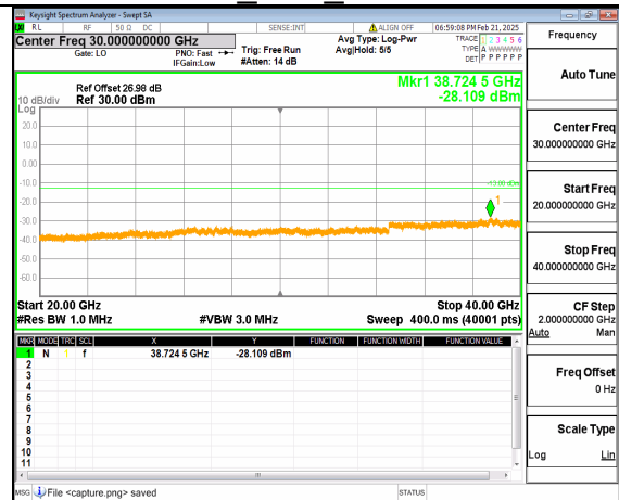
12A_n77(3700-3980MHz) (20GHz-40GHz) 30M DFT-s-OFDM QPSK Inner_1RB_Right Low
