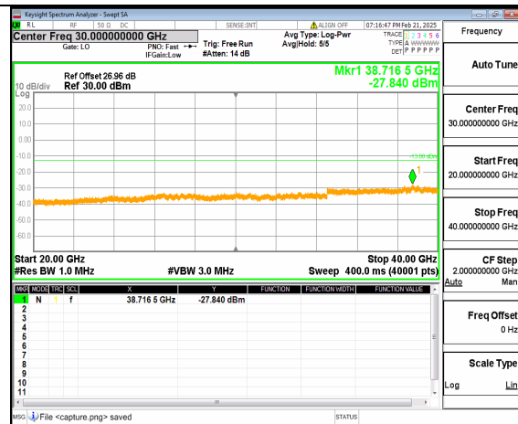
12A_n77(3700-3980MHz) (20GHz-40GHz) 40M DFT-s-OFDM QPSK Inner_1RB_Right High
