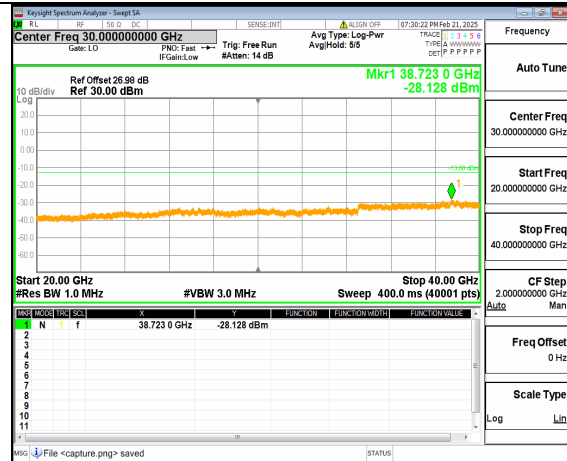
12A_n77(3700-3980MHz) (20GHz-40GHz) 60M DFT-s-OFDM QPSK Inner_1RB_Right Low
