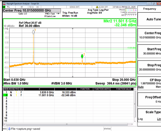
12A_n77(3700-3980MHz) (30MHz-20GHz) 30M DFT-s-OFDM QPSK Outer_Full_Mid
