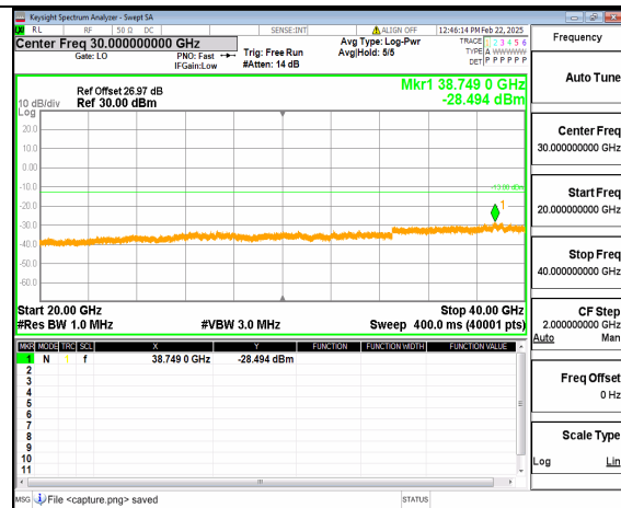
12A_n77(3700-3980MHz) (20GHz-40GHz) 70M DFT-s-OFDM QPSK Inner_1RB_Right Mid
