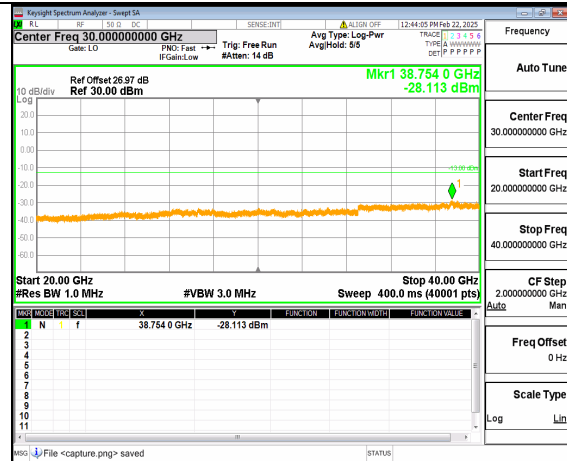
12A_n77(3700-3980MHz) (20GHz-40GHz) 70M DFT-s-OFDM QPSK Outer_Full_Mid
