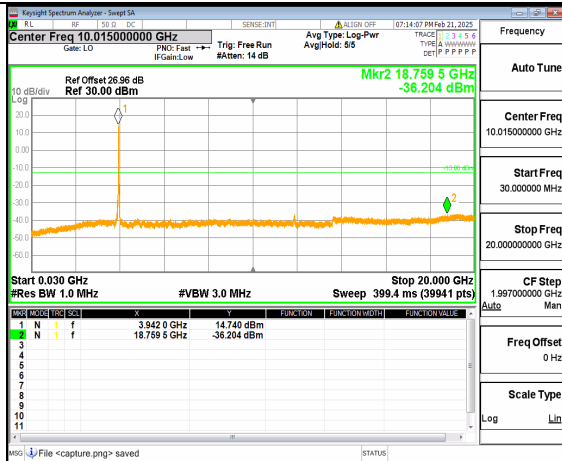
12A_n77(3700-3980MHz) (30MHz-20GHz) 40M DFT-s-OFDM QPSK Outer_Full_High
