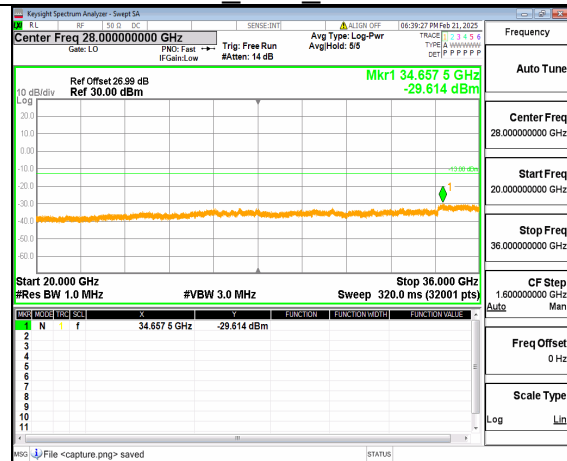
12A_n77(3450-3550MHz) (20GHz-36GHz) 90M DFT-s-OFDM QPSK Inner_1RB_Right Mid
