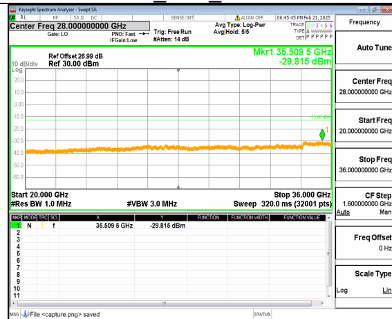
12A_n77(3450-3550MHz) (20GHz-36GHz) 100M DFT-s-OFDM QPSK Inner_1RB_Right Mid
