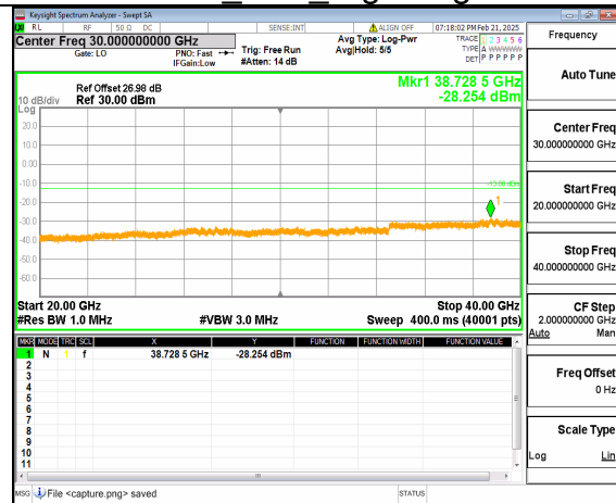
12A_n77(3700-3980MHz) (20GHz-40GHz) 50M DFT-s-OFDM QPSK Outer_Full Low
