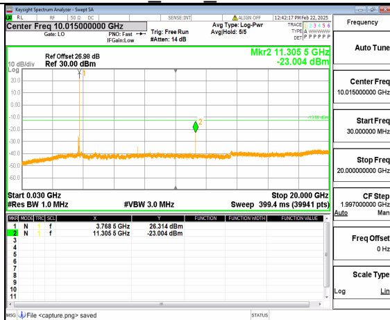
12A_n77(3700-3980MHz) (30MHz-20GHz) 70M DFT-s-OFDM QPSK Inner_1RB_Right Low
