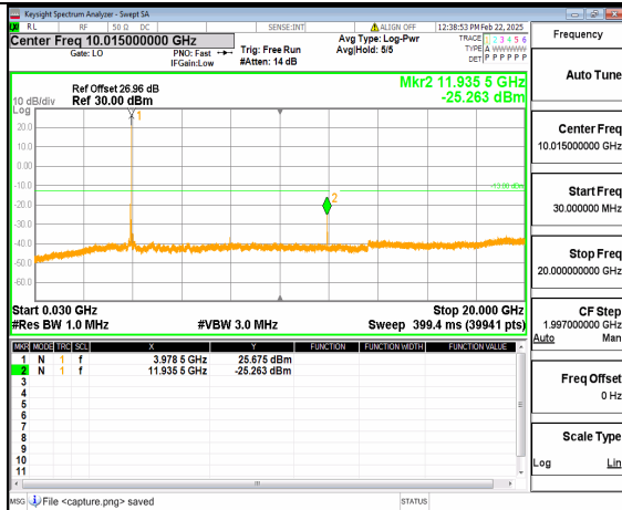
12A_n77(3700-3980MHz) (30MHz-20GHz) 60M DFT-s-OFDM QPSK Inner_1RB_Right_High
