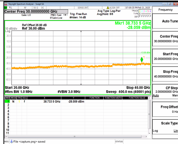
12A_n77(3700-3980MHz) (20GHz-40GHz) 40M DFT-s-OFDM QPSK Inner_1RB_Right Low
