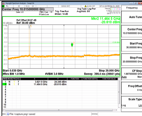
12A_n77(3700-3980MHz) (30MHz-20GHz) 40M DFT-s-OFDM QPSK Inner_1RB_Left Mid
