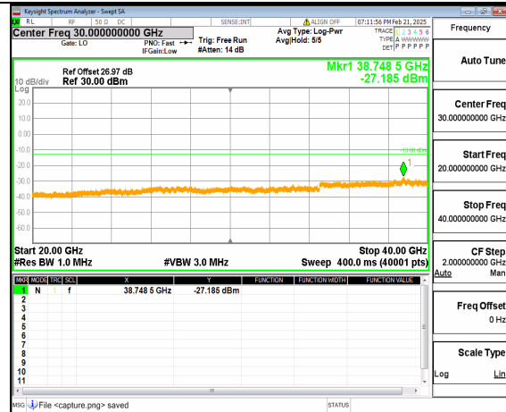
12A_n77(3700-3980MHz) (20GHz-40GHz) 40M DFT-s-OFDM QPSK Inner_1RB_Left Mid
