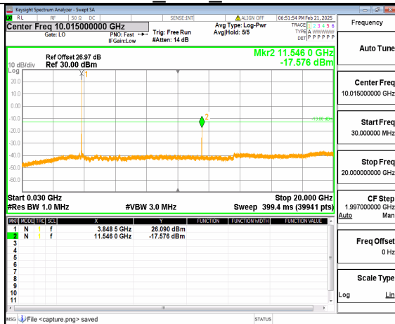
12A_n77(3700-3980MHz) (30MHz-20GHz) 20M DFT-s-OFDM QPSK Inner_1RB_Right Mid
