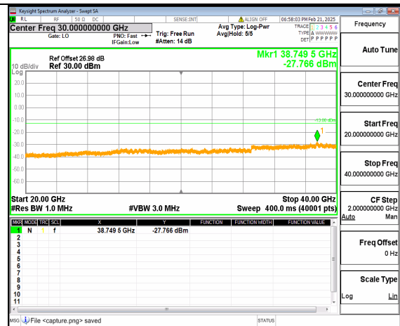
12A_n77(3700-3980MHz) (20GHz-40GHz) 30M DFT-s-OFDM QPSK Inner_1RB_Left Low
