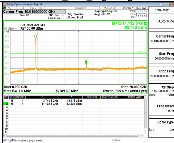
12A_n77(3700-3980MHz) (30MHz-20GHz) 50M DFT-s-OFDM QPSK Outer_Full Low
