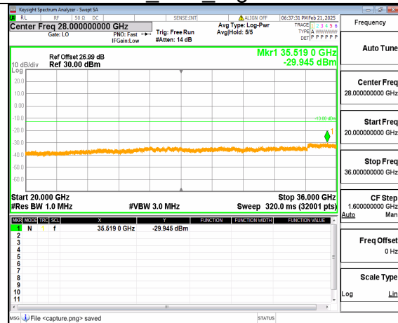
12A_n77(3450-3550MHz) (20GHz-36GHz) 90M DFT-s-OFDM QPSK Outer_Full Mid
