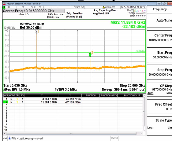
12A_n77(3700-3980MHz) (30MHz-20GHz) 20M DFT-s-OFDM QPSK Inner_1RB_Left_High
