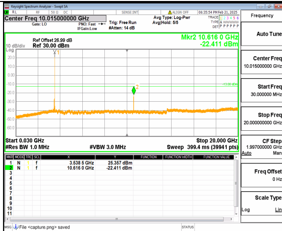
12A_n77(3450-3550MHz) (30MHz-20GHz) 90M DFT-s-OFDM QPSK Inner_1RB_Right Low
