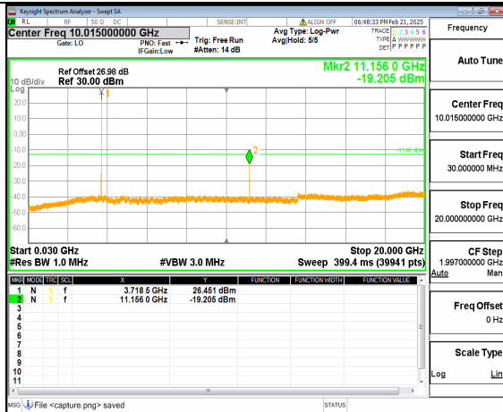
12A_n77(3700-3980MHz) (30MHz-20GHz) 20M DFT-s-OFDM QPSK Inner_1RB_Right Low
