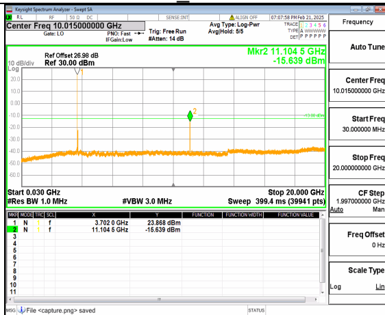
12A_n77(3700-3980MHz) (30MHz-20GHz) 40M DFT-s-OFDM QPSK Inner_1RB_Left Low
