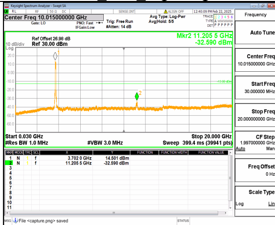
12A_n77(3700-3980MHz) (30MHz-20GHz) 70M DFT-s-OFDM QPSK Outer_Full_Low
