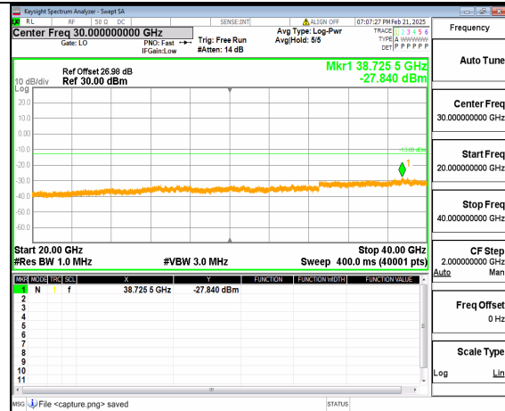
12A_n77(3700-3980MHz) (20GHz-40GHz) 40M DFT-s-OFDM QPSK Outer_Full Low
