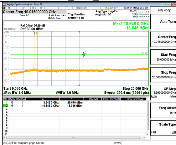
12A_n77(3450-3550MHz) (30MHz-20GHz) 100M DFT-s-OFDM QPSK Inner_1RB_Right Mid
