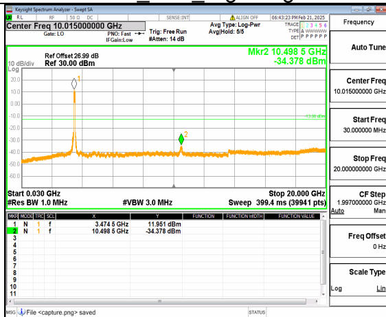
12A_n77(3450-3550MHz) (30MHz-20GHz) 100M DFT-s-OFDM QPSK Outer_Full Mid
