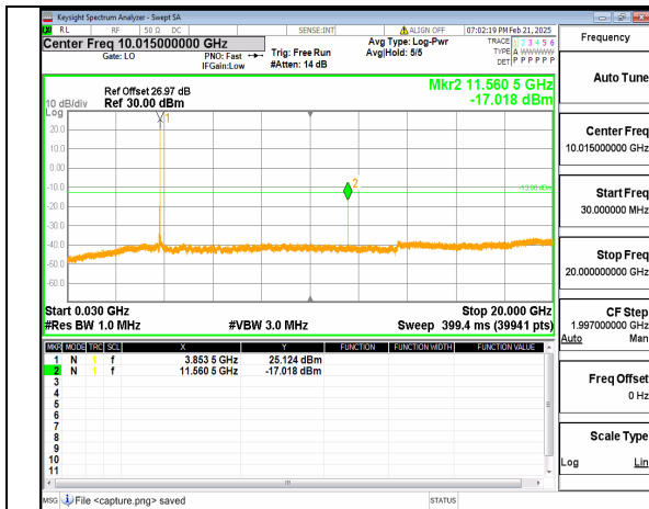
12A_n77(3700-3980MHz) (30MHz-20GHz) 30M DFT-s-OFDM QPSK Inner_1RB_Right Mid
