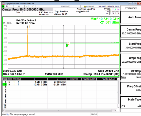
12A_n77(3450-3550MHz) (30MHz-20GHz) 90M DFT-s-OFDM QPSK Inner_1RB_Right Mid
