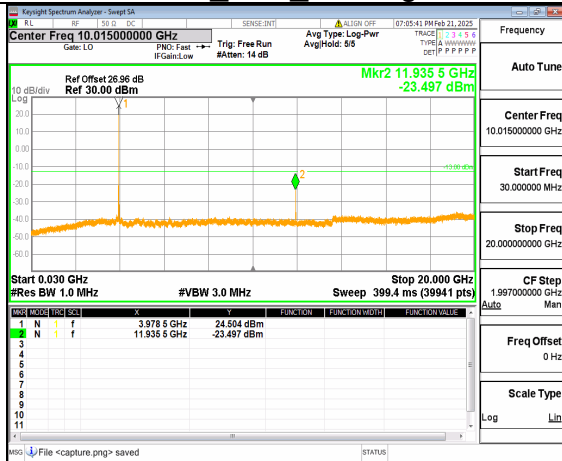
12A_n77(3700-3980MHz) (30MHz-20GHz) 30M DFT-s-OFDM QPSK Inner_1RB_Right High
