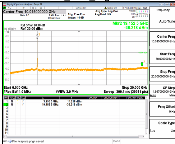
12A_n77(3700-3980MHz) (30MHz-20GHz) 30M DFT-s-OFDM QPSK Outer_Full High
