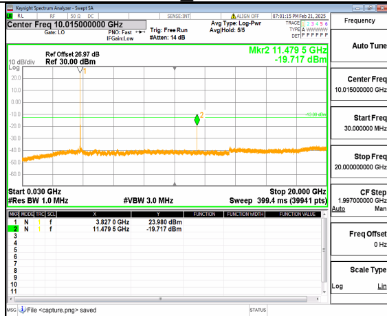
12A_n77(3700-3980MHz) (30MHz-20GHz) 30M DFT-s-OFDM QPSK Inner_1RB_Left_Mid
