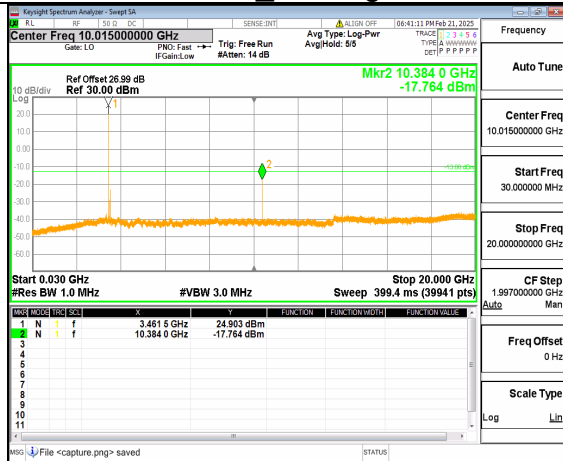
12A_n77(3450-3550MHz) (30MHz-20GHz) 90M DFT-s-OFDM QPSK Inner_1RB_Left_High
