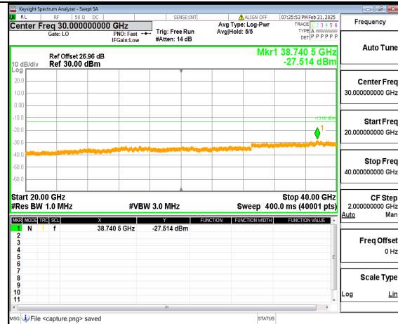
12A_n77(3700-3980MHz) (20GHz-40GHz) 50M DFT-s-OFDM QPSK Inner_1RB_Left High
