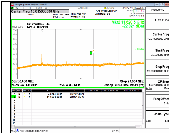
12A_n77(3700-3980MHz) (30MHz-20GHz) 70M DFT-s-OFDM QPSK Inner_1RB_Right Mid
