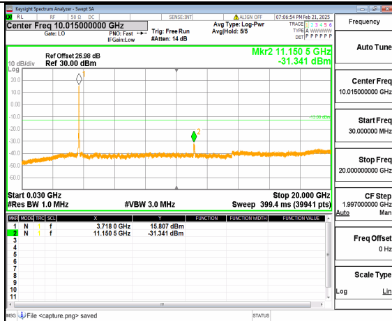
12A_n77(3700-3980MHz) (30MHz-20GHz) 40M DFT-s-OFDM QPSK Outer_Full Low
