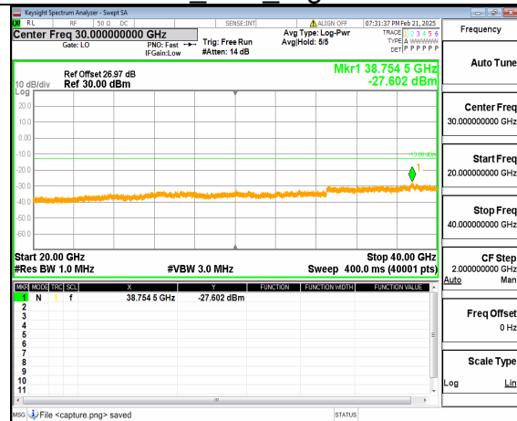
12A_n77(3700-3980MHz) (20GHz-40GHz) 60M DFT-s-OFDM QPSK Outer_Full Mid
