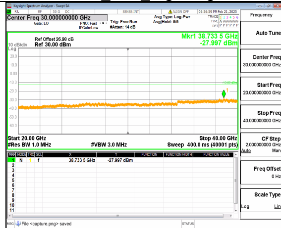
12A_n77(3700-3980MHz) (20GHz-40GHz) 30M DFT-s-OFDM QPSK Outer_Full_Low
