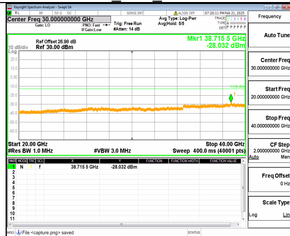
12A_n77(3700-3980MHz) (20GHz-40GHz) 50M DFT-s-OFDM QPSK Inner_1RB_Right Low
