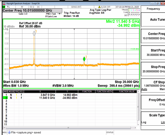
12A_n77(3700-3980MHz) (30MHz-20GHz) 40M DFT-s-OFDM QPSK Outer_Full Mid
