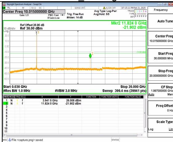
12A_n77(3700-3980MHz) (30MHz-20GHz) 40M DFT-s-OFDM QPSK Inner_1RB_Left_High
