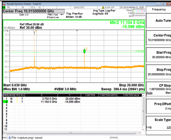
12A_n77(3700-3980MHz) (30MHz-20GHz) 50M DFT-s-OFDM QPSK Inner_1RB_Left Low
