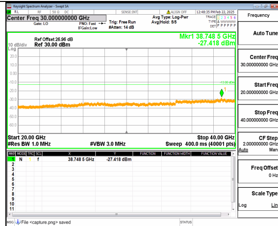
12A_n77(3700-3980MHz) (20GHz-40GHz) 70M DFT-s-OFDM QPSK Inner_1RB_Left_High
