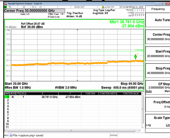
12A_n77(3700-3980MHz) (20GHz-40GHz) 40M DFT-s-OFDM QPSK Outer_Full Mid
