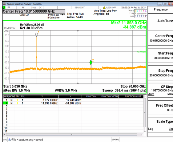
12A_n77(3700-3980MHz) (30MHz-20GHz) 20M DFT-s-OFDM QPSK Outer_Full_High
