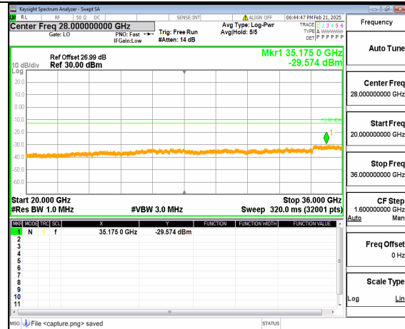
12A_n77(3450-3550MHz) (20GHz-36GHz) 100M DFT-s-OFDM QPSK Inner_1RB_Left Mid
