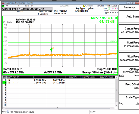
12A_n77(3700-3980MHz) (30MHz-20GHz) 50M DFT-s-OFDM QPSK Inner_1RB_Right High
