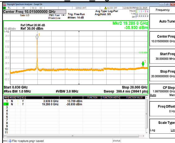
12A_n77(3700-3980MHz) (30MHz-20GHz) 70M DFT-s-OFDM QPSK Outer_Full High
