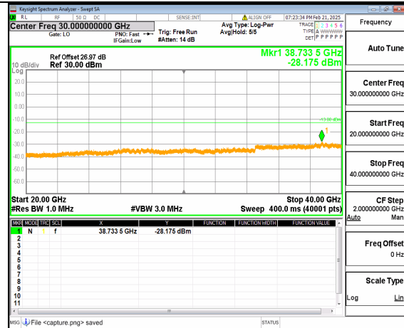
12A_n77(3700-3980MHz) (20GHz-40GHz) 50M DFT-s-OFDM QPSK Inner_1RB_Right Mid
