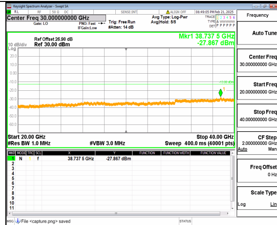
12A_n77(3700-3980MHz) (20GHz-40GHz) 20M DFT-s-OFDM QPSK Inner_1RB_Right Low
