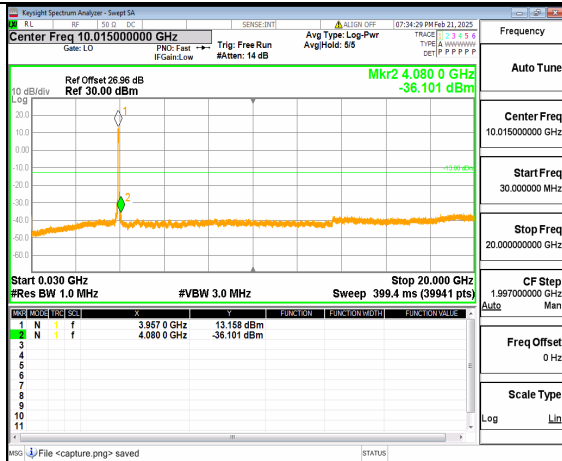
12A_n77(3700-3980MHz) (30MHz-20GHz) 60M DFT-s-OFDM QPSK Outer_Full_High
