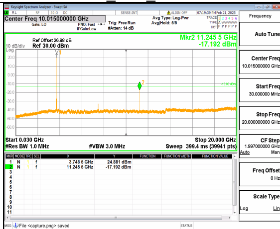
12A_n77(3700-3980MHz) (30MHz-20GHz) 50M DFT-s-OFDM QPSK Inner_1RB_Right Low
