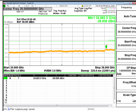
12A_n77(3450-3550MHz) (20GHz-36GHz) 90M DFT-s-OFDM QPSK Inner_1RB_Right Low
