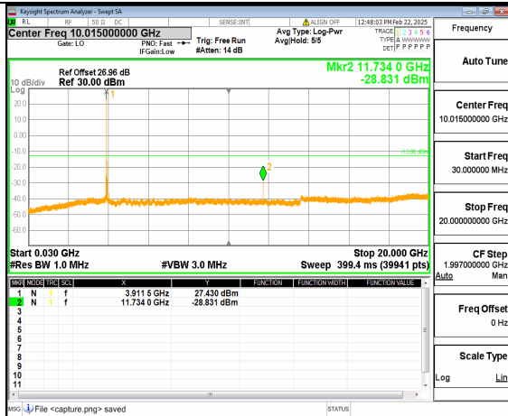
12A_n77(3700-3980MHz) (30MHz-20GHz) 70M DFT-s-OFDM QPSK Inner_1RB_Left_High
