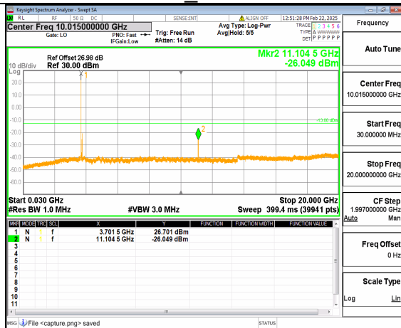
12A_n77(3700-3980MHz) (30MHz-20GHz) 80M DFT-s-OFDM QPSK Inner_1RB_Left Low
