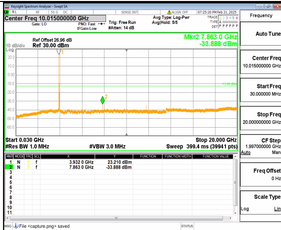
12A_n77(3700-3980MHz) (30MHz-20GHz) 50M DFT-s-OFDM QPSK Inner_1RB_Left High
