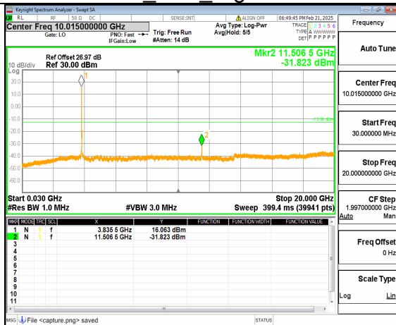
12A_n77(3700-3980MHz) (30MHz-20GHz) 20M DFT-s-OFDM QPSK Outer_Full Mid
