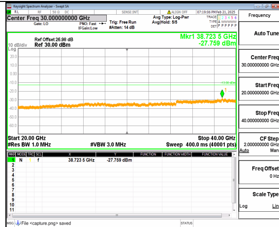
12A_n77(3700-3980MHz) (20GHz-40GHz) 50M DFT-s-OFDM QPSK Inner_1RB_Left Low
