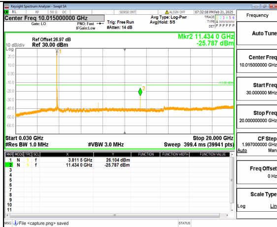
12A_n77(3700-3980MHz) (30MHz-20GHz) 60M DFT-s-OFDM QPSK Inner_1RB_Left Mid
