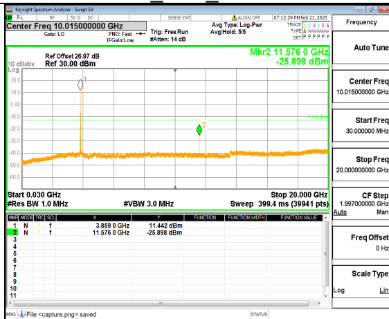
12A_n77(3700-3980MHz) (30MHz-20GHz) 40M DFT-s-OFDM QPSK Inner_1RB_Right Mid
