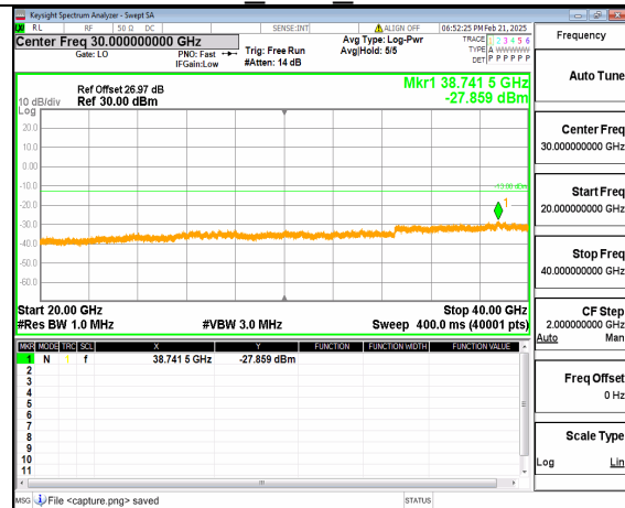
12A_n77(3700-3980MHz) (20GHz-40GHz) 20M DFT-s-OFDM QPSK Inner_1RB_Right Mid
