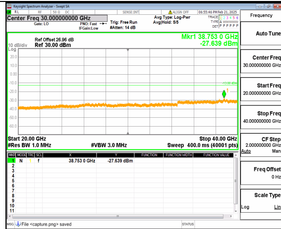
12A_n77(3700-3980MHz) (20GHz-40GHz) 20M DFT-s-OFDM QPSK Inner_1RB_Right_High
