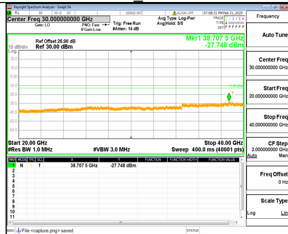
12A_n77(3700-3980MHz) (20GHz-40GHz) 40M DFT-s-OFDM QPSK Inner_1RB_Left Low
