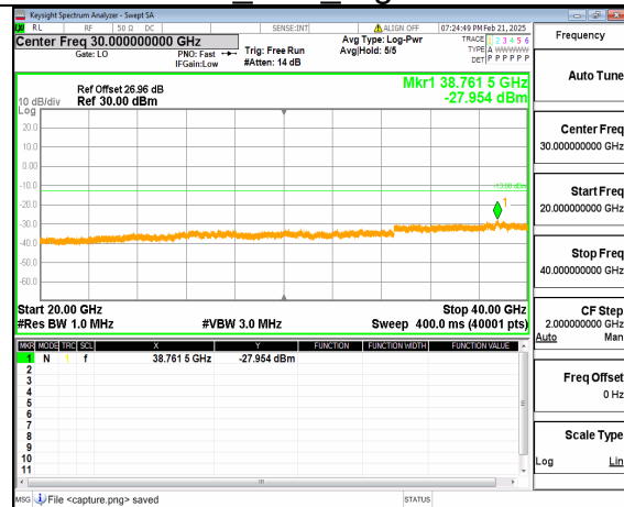
12A_n77(3700-3980MHz) (20GHz-40GHz) 50M DFT-s-OFDM QPSK Outer_Full High
