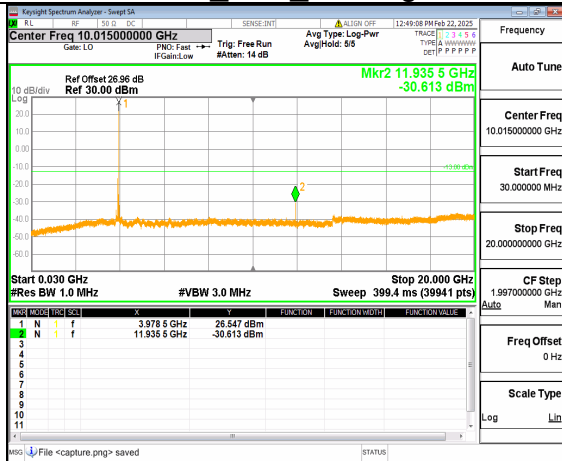
12A_n77(3700-3980MHz) (30MHz-20GHz) 70M DFT-s-OFDM QPSK Inner_1RB_Right_High
