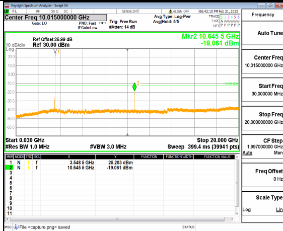
12A_n77(3450-3550MHz) (30MHz-20GHz) 90M DFT-s-OFDM QPSK Inner_1RB_Right High
