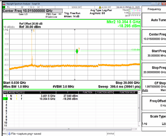
12A_n77(3450-3550MHz) (30MHz-20GHz) 100M DFT-s-OFDM QPSK Inner_1RB_Left Mid
