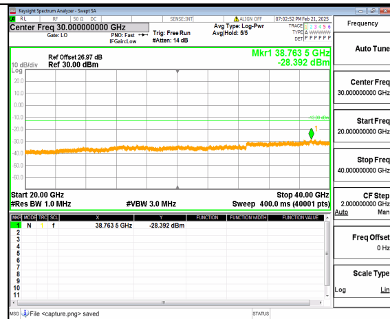
12A_n77(3700-3980MHz) (20GHz-40GHz) 30M DFT-s-OFDM QPSK Inner_1RB_Right Mid
