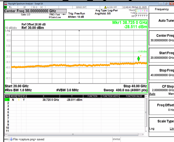
12A_n77(3700-3980MHz) (20GHz-40GHz) 70M DFT-s-OFDM QPSK Outer_Full_Low
