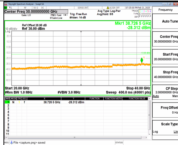
12A_n77(3700-3980MHz) (20GHz-40GHz) 60M DFT-s-OFDM QPSK Outer_Full_High
