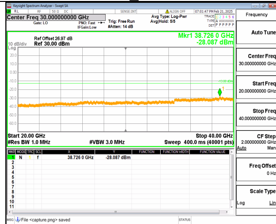
12A_n77(3700-3980MHz) (20GHz-40GHz) 30M DFT-s-OFDM QPSK Inner_1RB_Left_Mid
