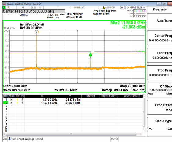
12A_n77(3700-3980MHz) (30MHz-20GHz) 20M DFT-s-OFDM QPSK Inner_1RB_Right_High
