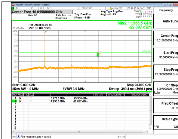
12A_n77(3700-3980MHz) (30MHz-20GHz) 40M DFT-s-OFDM QPSK Inner_1RB_Right High
