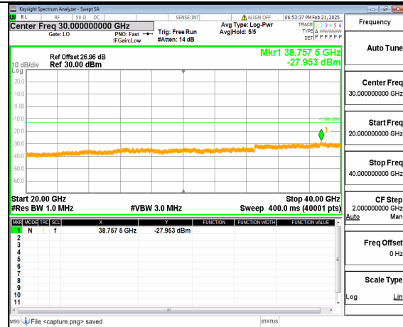
12A_n77(3700-3980MHz) (20GHz-40GHz) 20M DFT-s-OFDM QPSK Outer_Full_High
