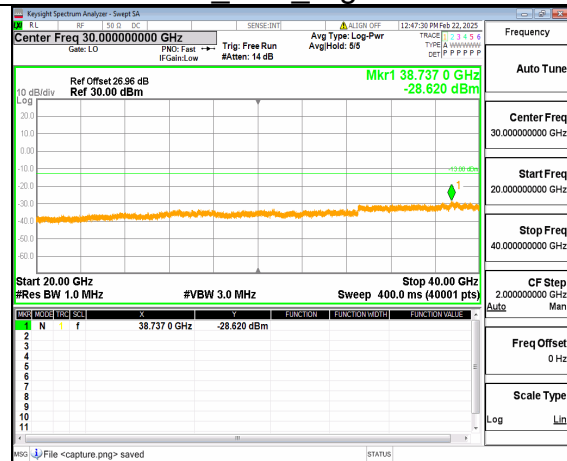
12A_n77(3700-3980MHz) (20GHz-40GHz) 70M DFT-s-OFDM QPSK Outer_Full High
