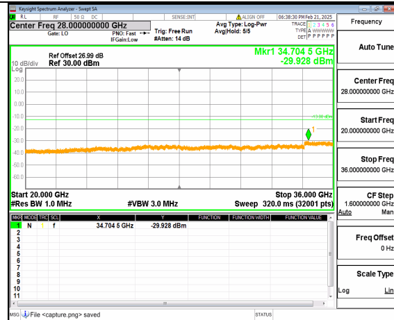
12A_n77(3450-3550MHz) (20GHz-36GHz) 90M DFT-s-OFDM QPSK Inner_1RB_Left Mid
