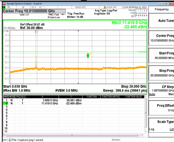
12A_n77(3700-3980MHz) (30MHz-20GHz) 70M DFT-s-OFDM QPSK Inner_1RB_Left_Mid
