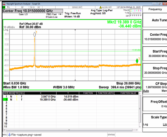
12A_n77(3700-3980MHz) (30MHz-20GHz) 50M DFT-s-OFDM QPSK Outer_Full_Mid
