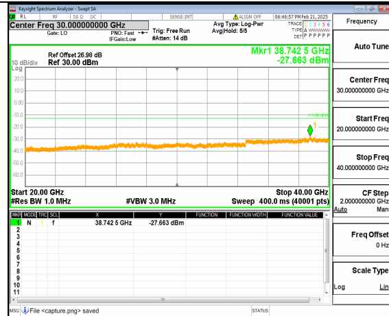
12A_n77(3700-3980MHz) (20GHz-40GHz) 20M DFT-s-OFDM QPSK Outer_Full Low
