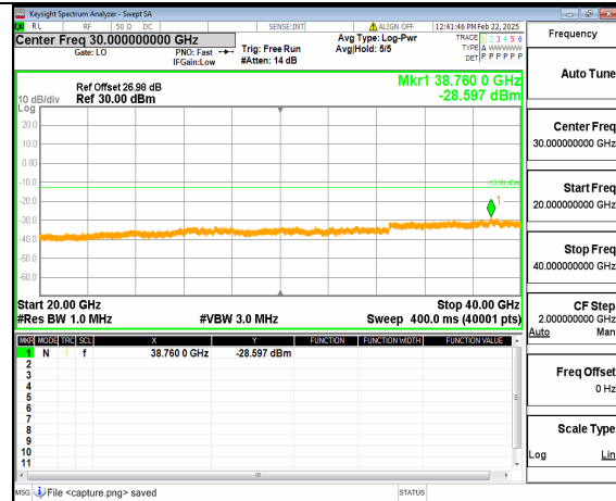
12A_n77(3700-3980MHz) (20GHz-40GHz) 70M DFT-s-OFDM QPSK Inner_1RB_Left Low
