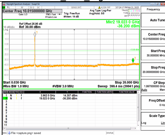
12A_n77(3700-3980MHz) (30MHz-20GHz) 50M DFT-s-OFDM QPSK Outer_Full High
