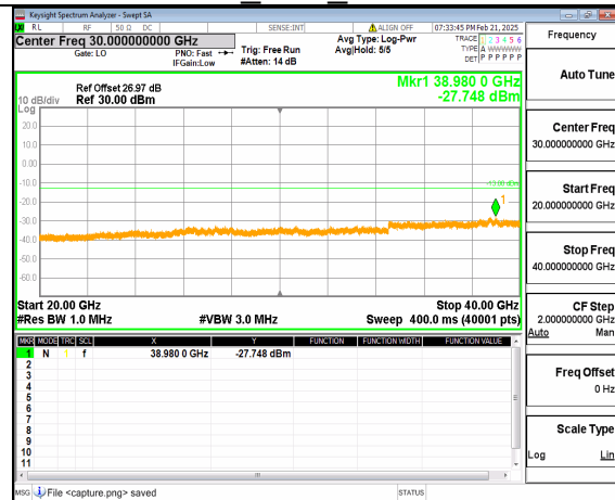
12A_n77(3700-3980MHz) (20GHz-40GHz) 60M DFT-s-OFDM QPSK Inner_1RB_Right Mid
