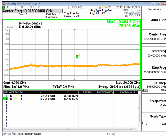
12A_n77(3450-3550MHz) (30MHz-20GHz) 40M DFT-s-OFDM QPSK Inner_1RB_Left Low
