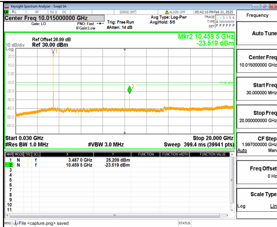
12A_n77(3450-3550MHz) (30MHz-20GHz) 30M DFT-s-OFDM QPSK Inner_1RB_Left Mid
