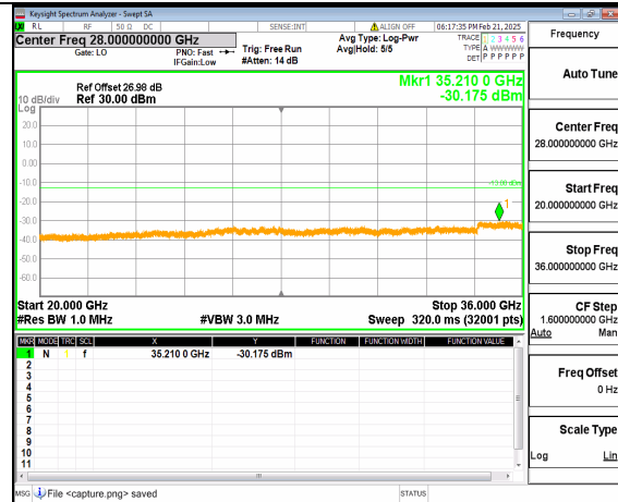
12A_n77(3450-3550MHz) (20GHz-36GHz) 70M DFT-s-OFDM QPSK Inner 1RB Right Low
