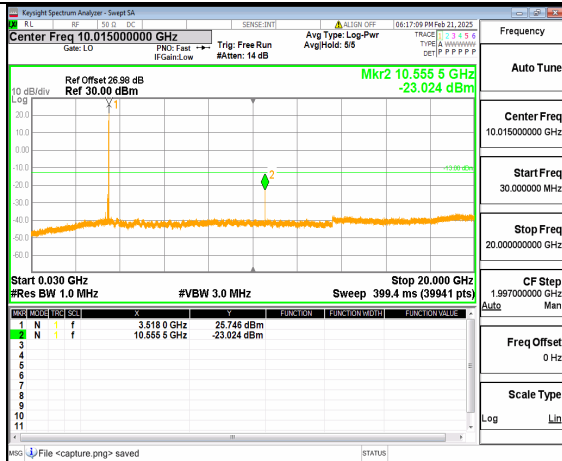
12A_n77(3450-3550MHz) (30MHz-20GHz) 70M DFT-s-OFDM QPSK Inner 1RB Right Low
