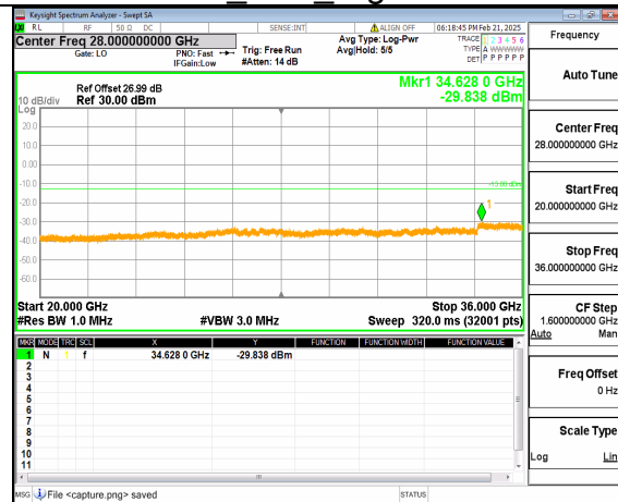
12A_n77(3450-3550MHz) (20GHz-36GHz) 70M DFT-s-OFDM QPSK Outer Full Mid
