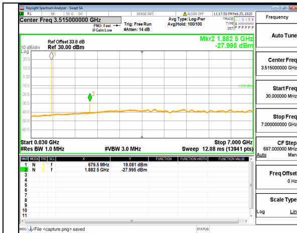
2A_n71 (30MHz-7GHz) 20M DFT-s-OFDM QPSK Inner_1RB_Left High
