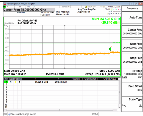
12A_n77(3450-3550MHz) (20GHz-36GHz) 20M DFT-s-OFDM QPSK Outer_Full Low
