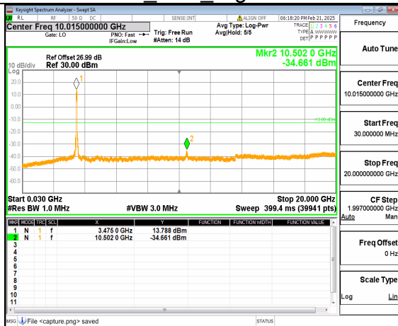
12A_n77(3450-3550MHz) (30MHz-20GHz) 70M DFT-s-OFDM QPSK Outer Full Mid
