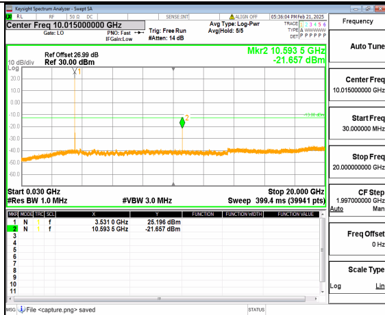
12A_n77(3450-3550MHz) (30MHz-20GHz) 20M DFT-s-OFDM QPSK Inner_1RB_Left High
