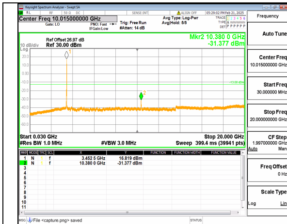
12A_n77(3450-3550MHz) (30MHz-20GHz) 20M DFT-s-OFDM QPSK Outer_Full Low
