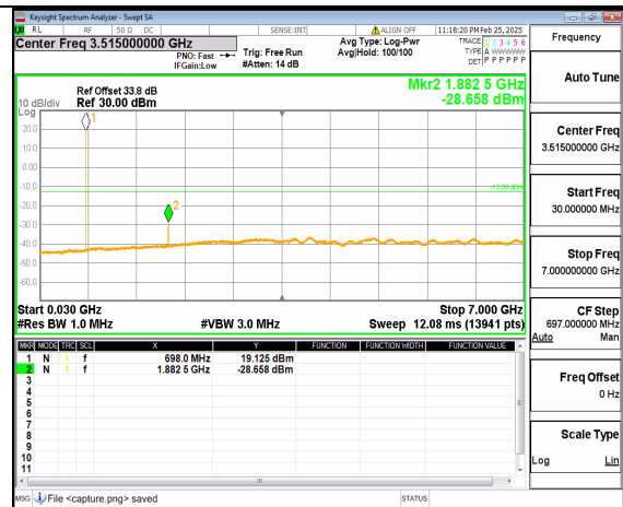
2A_n71 (30MHz-7GHz) 20M DFT-s-OFDM QPSK Inner_1RB_Right High
