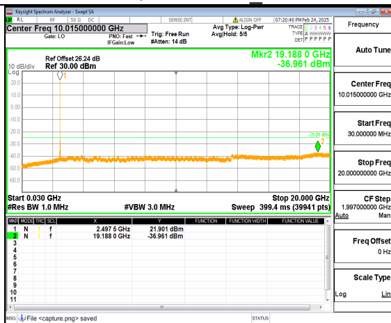
66A_n41 (30MHz-20GHz) 30M DFT-s-OFDM QPSK Inner_1RB_Left_Low
