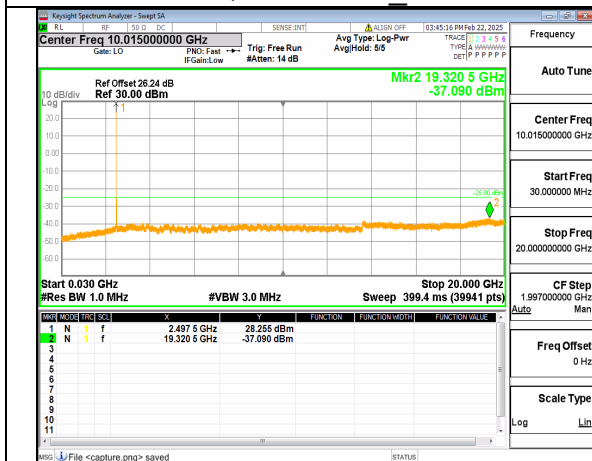
66A_n41 (30MHz-20GHz) 20M DFT-s-OFDM QPSK Inner_1RB_Left_Low
