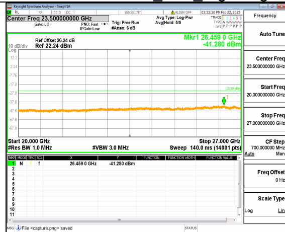
66A_n41 (20GHz-27GHz) 30M DFT-s-OFDM QPSK Outer_Full_Low
