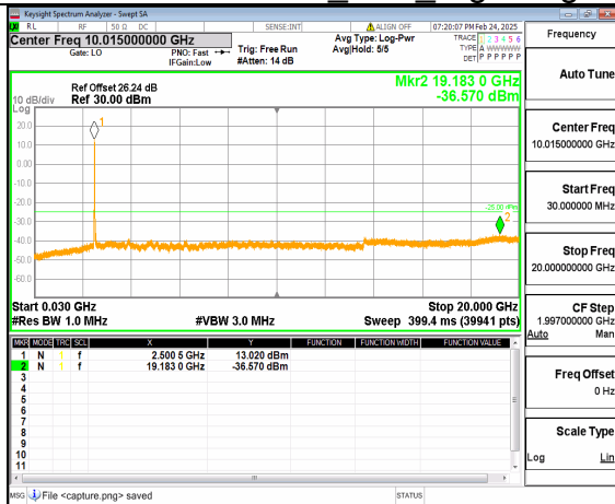
66A_n41 (30MHz-20GHz) 30M DFT-s-OFDM QPSK Outer_Full_Low
