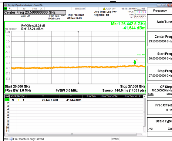
66A_n41 (20GHz-27GHz) 30M DFT-s-OFDM QPSK Inner_1RB_Left_Low
