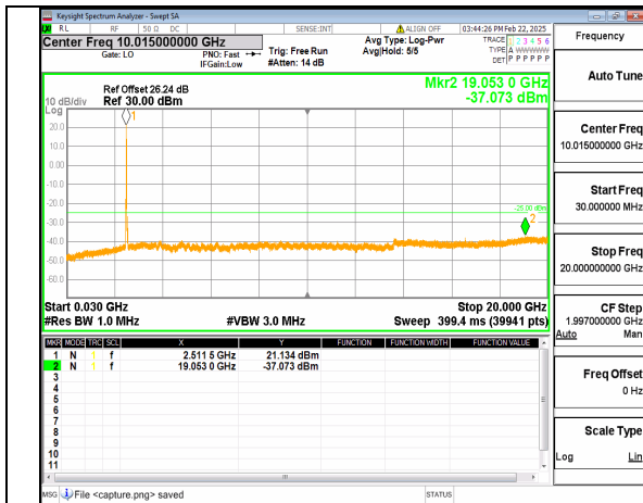
66A_n41 (30MHz-20GHz) 20M DFT-s-OFDM QPSK Outer_Full_Low
