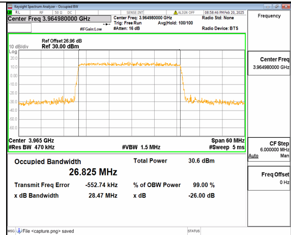
12A_n77(3700-3980MHz) 30M DFT-s-OFDM 64QAM Outer_Full High
