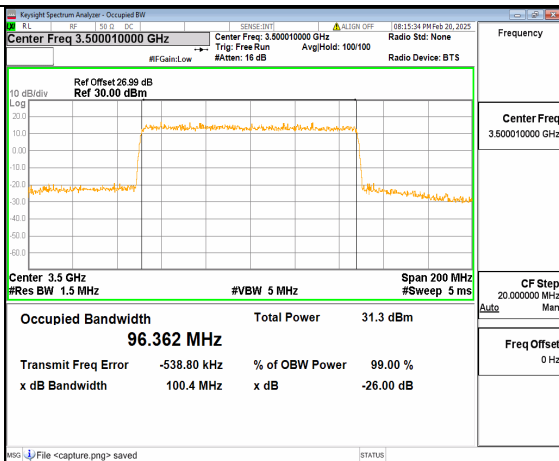
12A_n77(3450-3550MHz) 100M DFT-s-OFDM 16QAM Outer_Full Mid
