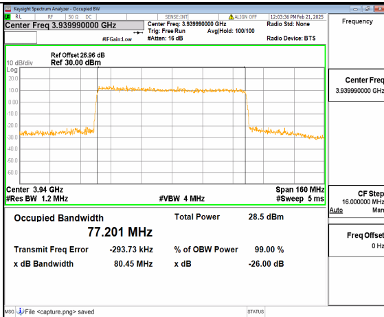
12A_n77(3700-3980MHz) 80M DFT-s-OFDM 16QAM Outer_Full High
