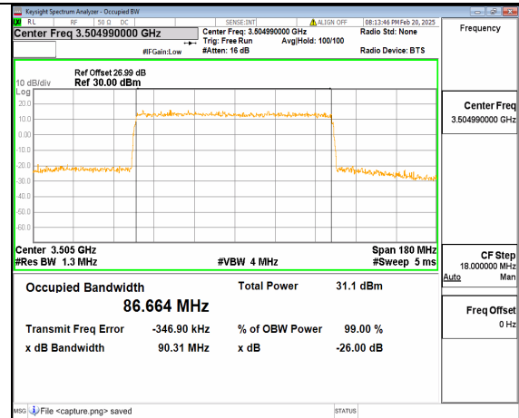
12A_n77(3450-3550MHz) 90M DFT-s-OFDM 64QAM Outer_Full High
