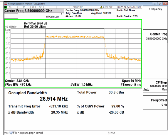
12A_n77(3700-3980MHz) 30M DFT-s-OFDM 64QAM Outer_Full Mid
