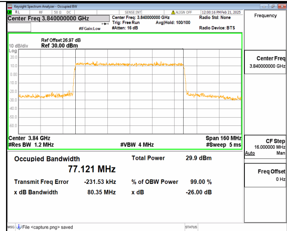
12A_n77(3700-3980MHz) 80M DFT-s-OFDM QPSK Outer_Full Mid
