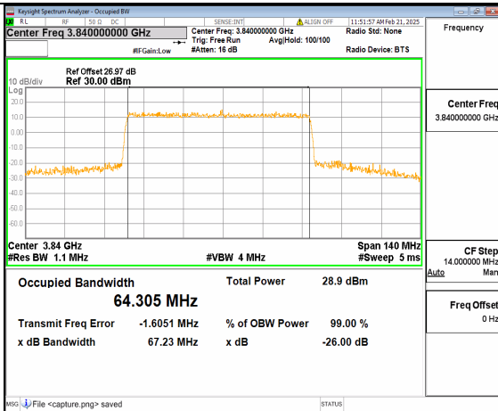
12A_n77(3700-3980MHz) 70M DFT-s-OFDM 16QAM Outer_Full Mid
