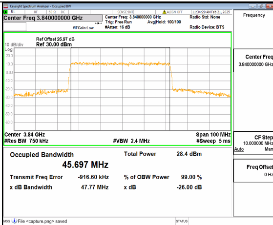
12A_n77(3700-3980MHz) 50M DFT-s-OFDM 16QAM Outer_Full Mid
