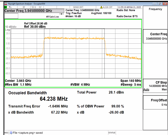
12A_n77(3700-3980MHz) 70M DFT-s-OFDM 64QAM Outer_Full High
