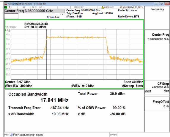
12A_n77(3700-3980MHz) 20M DFT-s-OFDM 64QAM Outer_Full High
