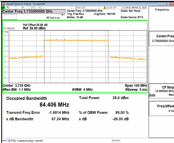
12A_n77(3700-3980MHz) 70M DFT-s-OFDM 16QAM Outer_Full Low
