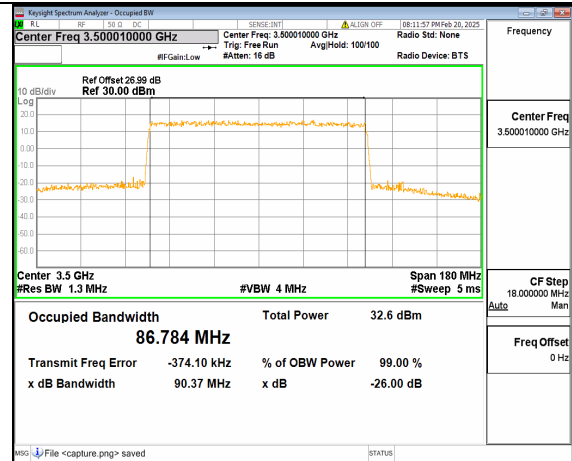
12A_n77(3450-3550MHz) 90M DFT-s-OFDM QPSK Outer_Full Mid
