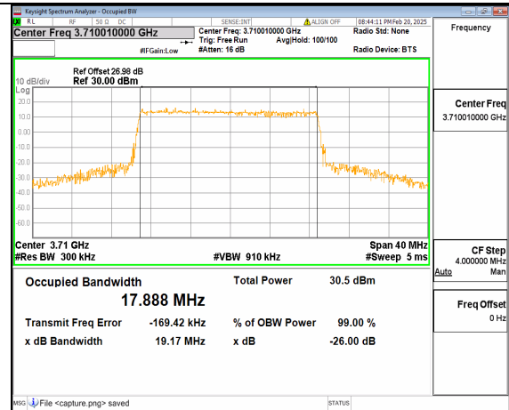
12A_n77(3700-3980MHz) 20M DFT-s-OFDM 64QAM Outer_Full Low
