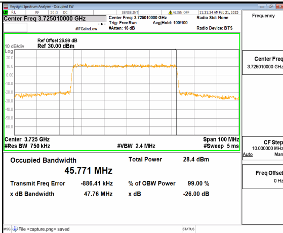
12A_n77(3700-3980MHz) 50M DFT-s-OFDM 16QAM Outer_Full Low
