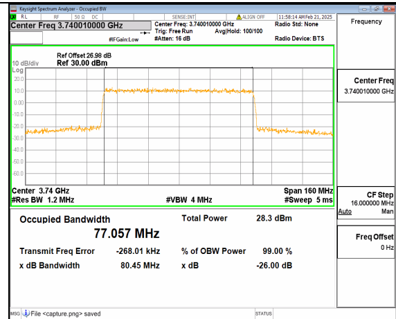
12A_n77(3700-3980MHz) 80M DFT-s-OFDM 64QAM Outer_Full Low
