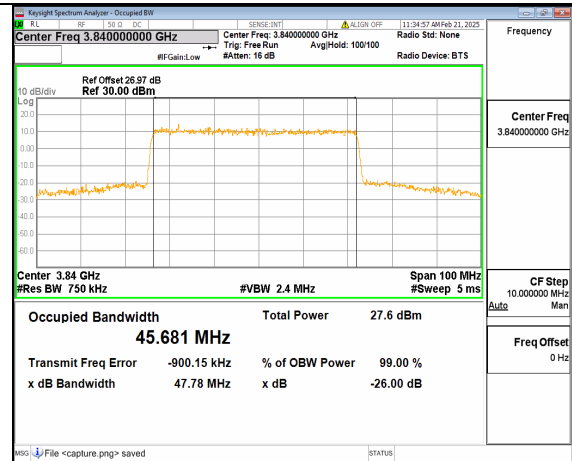
12A_n77(3700-3980MHz) 50M DFT-s-OFDM 64QAM Outer_Full Mid
