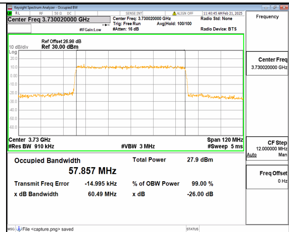
12A_n77(3700-3980MHz) 60M DFT-s-OFDM 64QAM Outer_Full Low
