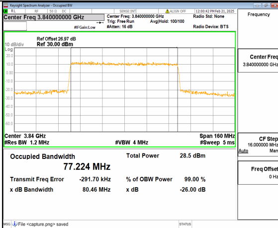
12A_n77(3700-3980MHz) 80M DFT-s-OFDM 16QAM Outer_Full Mid
