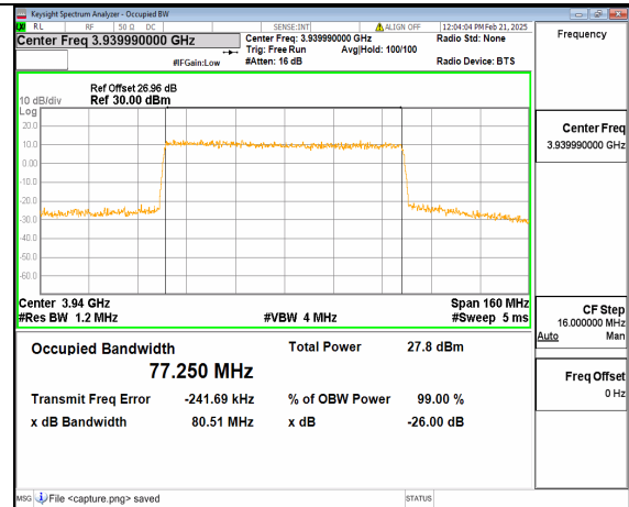
12A_n77(3700-3980MHz) 80M DFT-s-OFDM 64QAM Outer_Full High
