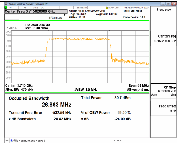
12A_n77(3700-3980MHz) 30M DFT-s-OFDM 64QAM Outer_Full Low
