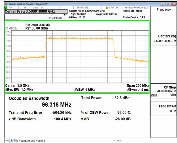
12A_n77(3450-3550MHz) 100M DFT-s-OFDM QPSK Outer_Full Mid
