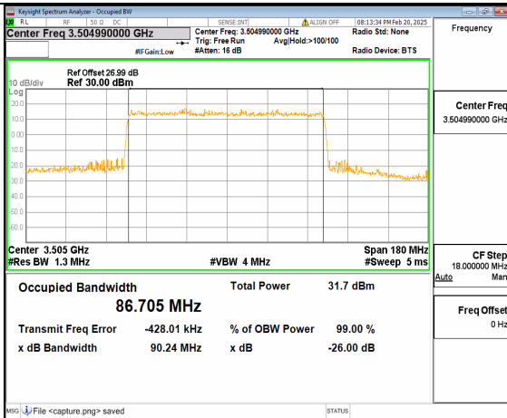
12A_n77(3450-3550MHz) 90M DFT-s-OFDM 16QAM Outer_Full High
