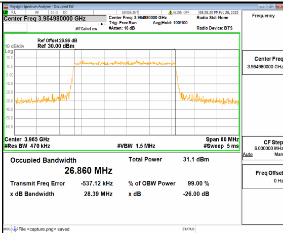
12A_n77(3700-3980MHz) 30M DFT-s-OFDM 16QAM Outer_Full High
