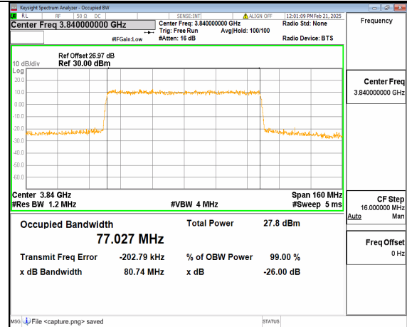
12A_n77(3700-3980MHz) 80M DFT-s-OFDM 64QAM Outer_Full Mid
