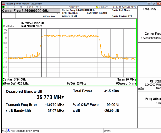
12A_n77(3700-3980MHz) 40M DFT-s-OFDM 16QAM Outer_Full Mid
