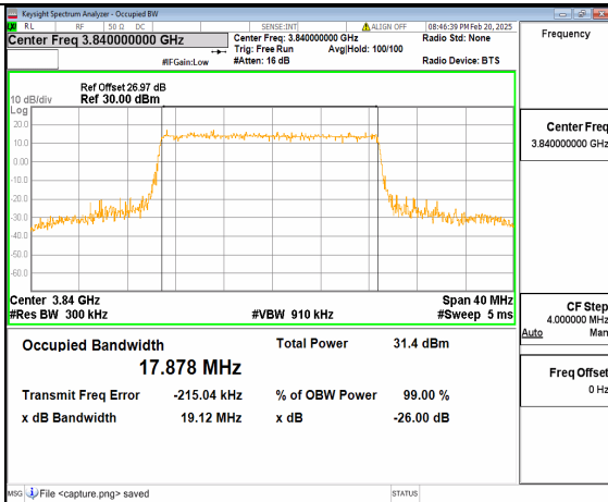
12A_n77(3700-3980MHz) 20M DFT-s-OFDM 16QAM Outer_Full Mid
