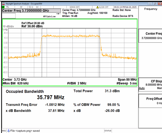
12A_n77(3700-3980MHz) 40M DFT-s-OFDM 16QAM Outer_Full Low
