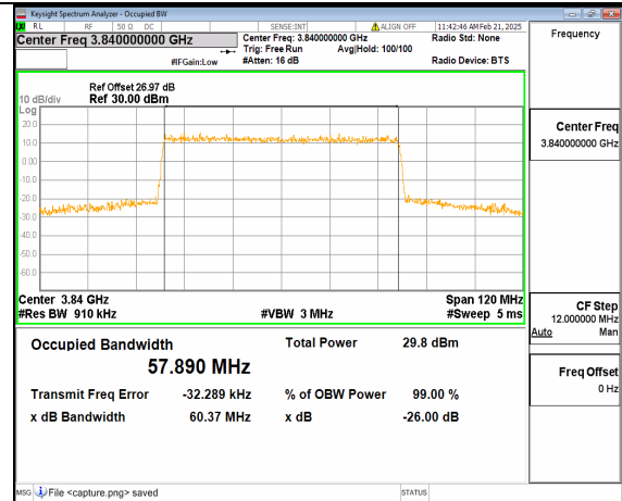
12A_n77(3700-3980MHz) 60M DFT-s-OFDM QPSK Outer_Full Mid
