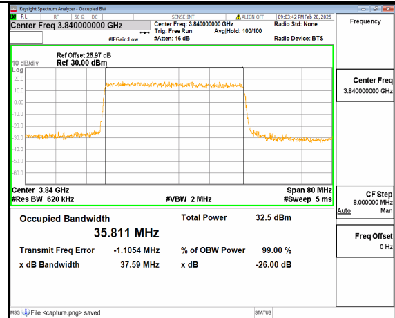
12A_n77(3700-3980MHz) 40M DFT-s-OFDM QPSK Outer_Full Mid
