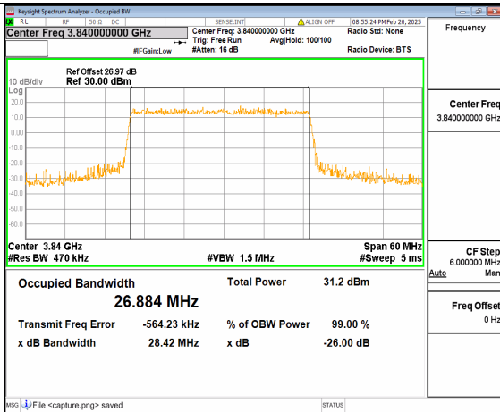
12A_n77(3700-3980MHz) 30M DFT-s-OFDM 16QAM Outer_Full Mid
