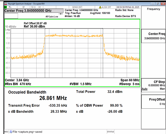
12A_n77(3700-3980MHz) 30M DFT-s-OFDM QPSK Outer_Full Mid
