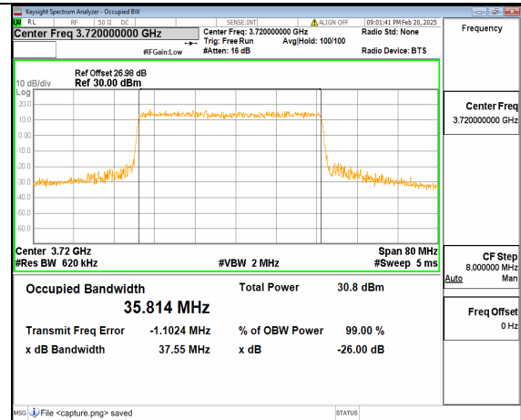
12A_n77(3700-3980MHz) 40M DFT-s-OFDM 64QAM Outer_Full Low
