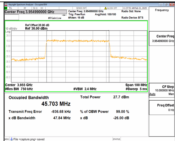
12A_n77(3700-3980MHz) 50M DFT-s-OFDM 64QAM Outer_Full High
