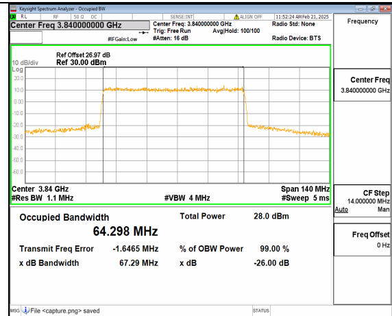
12A_n77(3700-3980MHz) 70M DFT-s-OFDM 64QAM Outer_Full Mid
