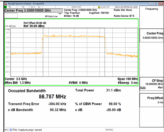
12A_n77(3450-3550MHz) 90M DFT-s-OFDM 64QAM Outer_Full Mid
