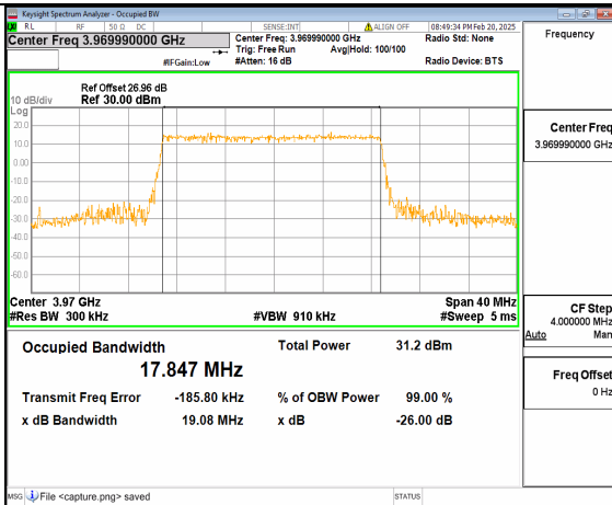
12A_n77(3700-3980MHz) 20M DFT-s-OFDM 16QAM Outer_Full High
