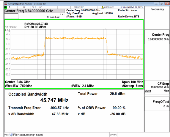
12A_n77(3700-3980MHz) 50M DFT-s-OFDM QPSK Outer_Full Mid
