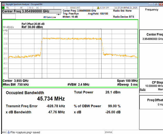
12A_n77(3700-3980MHz) 50M DFT-s-OFDM 16QAM Outer_Full High
