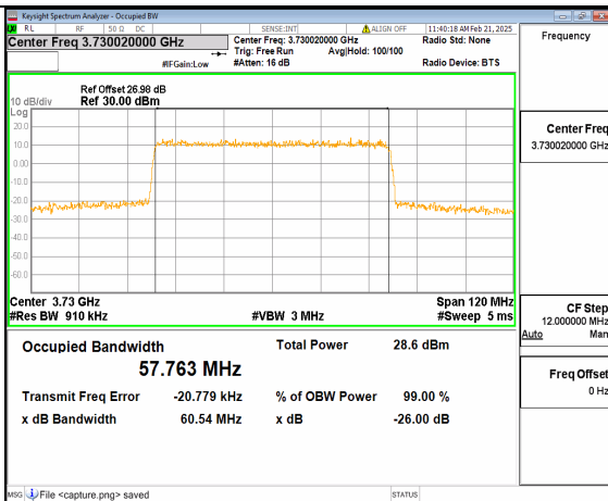
12A_n77(3700-3980MHz) 60M DFT-s-OFDM 16QAM Outer_Full Low
