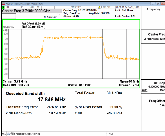
12A_n77(3700-3980MHz) 20M DFT-s-OFDM 16QAM Outer_Full Low
