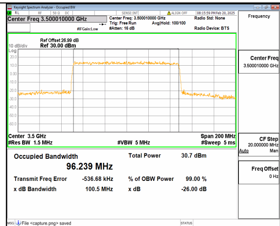
12A_n77(3450-3550MHz) 100M DFT-s-OFDM 64QAM Outer_Full Mid
