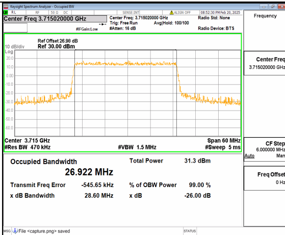
12A_n77(3700-3980MHz) 30M DFT-s-OFDM 16QAM Outer_Full Low
