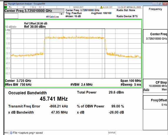
12A_n77(3700-3980MHz) 50M DFT-s-OFDM QPSK Outer_Full Low
