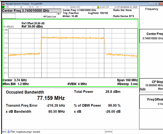
12A_n77(3700-3980MHz) 80M DFT-s-OFDM 16QAM Outer_Full Low
