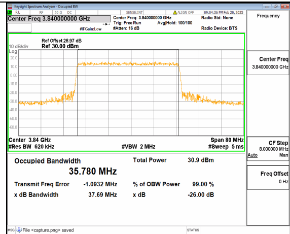
12A_n77(3700-3980MHz) 40M DFT-s-OFDM 64QAM Outer_Full Mid
