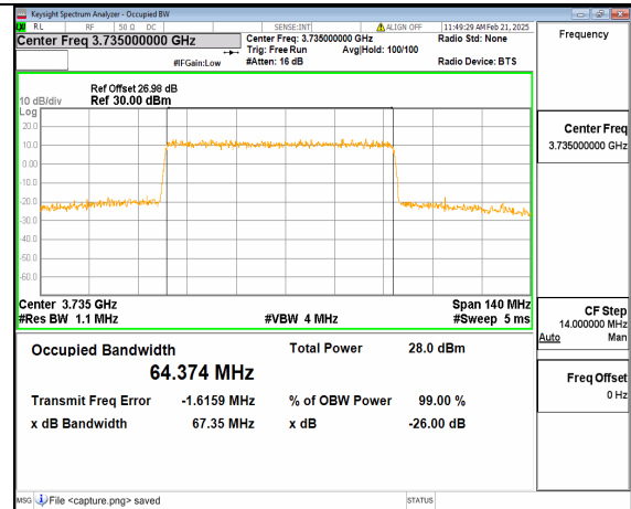
12A_n77(3700-3980MHz) 70M DFT-s-OFDM 64QAM Outer_Full Low
