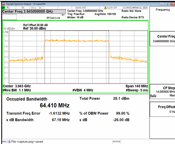
12A_n77(3700-3980MHz) 70M DFT-s-OFDM 16QAM Outer_Full High
