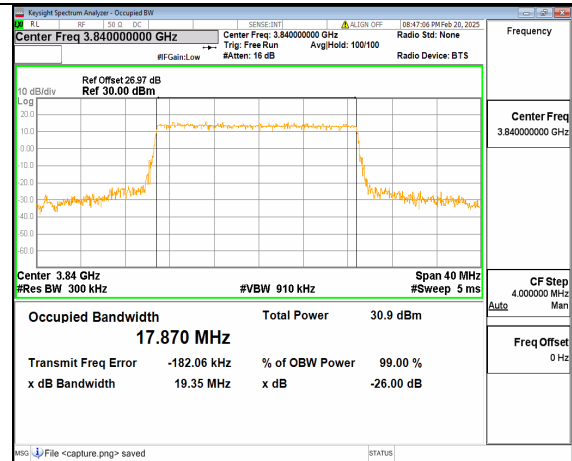
12A_n77(3700-3980MHz) 20M DFT-s-OFDM 64QAM Outer_Full Mid
