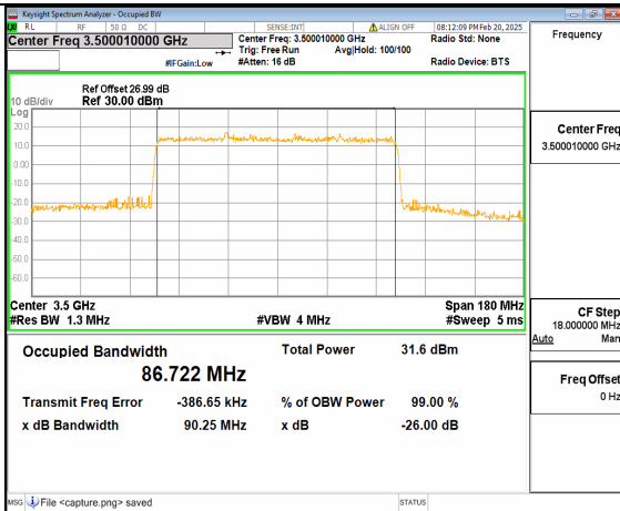
12A_n77(3450-3550MHz) 90M DFT-s-OFDM 16QAM Outer_Full Mid
