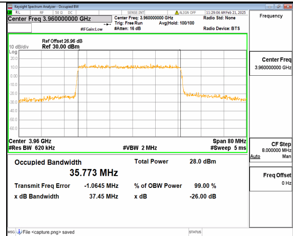
12A_n77(3700-3980MHz) 40M DFT-s-OFDM 64QAM Outer_Full High
