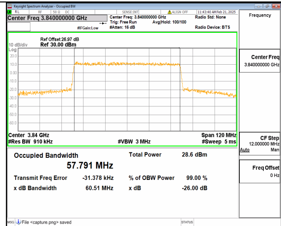
12A_n77(3700-3980MHz) 60M DFT-s-OFDM 64QAM Outer_Full Mid
