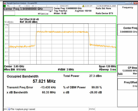
12A_n77(3700-3980MHz) 60M DFT-s-OFDM 64QAM Outer_Full High
