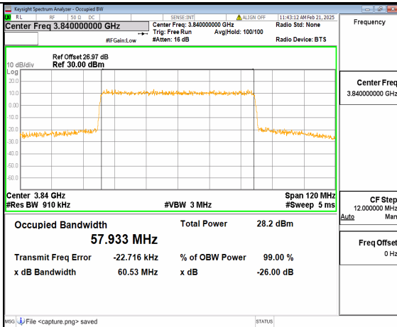
12A_n77(3700-3980MHz) 60M DFT-s-OFDM 16QAM Outer_Full Mid
