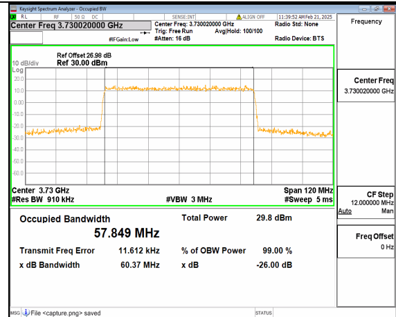
12A_n77(3700-3980MHz) 60M DFT-s-OFDM QPSK Outer_Full Low
