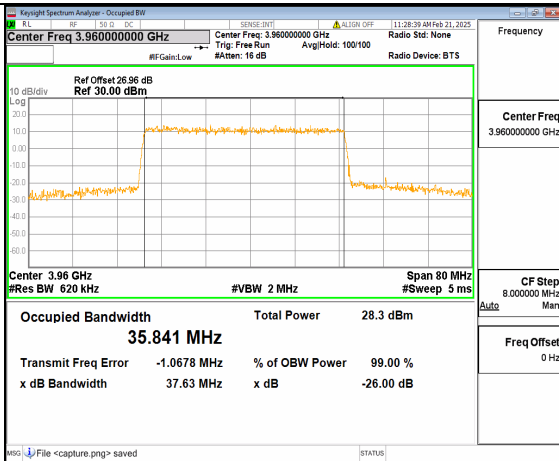
12A_n77(3700-3980MHz) 40M DFT-s-OFDM 16QAM Outer_Full High
