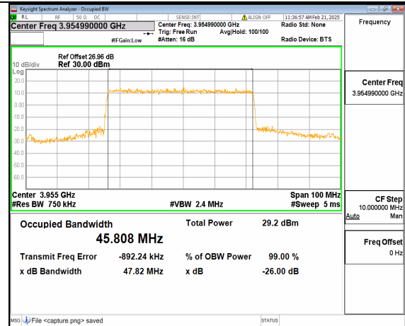
12A_n77(3700-3980MHz) 50M DFT-s-OFDM QPSK Outer_Full High
