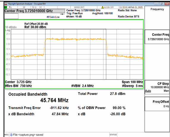
12A_n77(3700-3980MHz) 50M DFT-s-OFDM 64QAM Outer_Full Low
