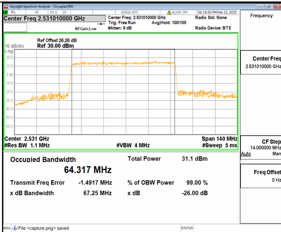
66A_n41 70M DFT-s-OFDM 16QAM Outer_Full Low
