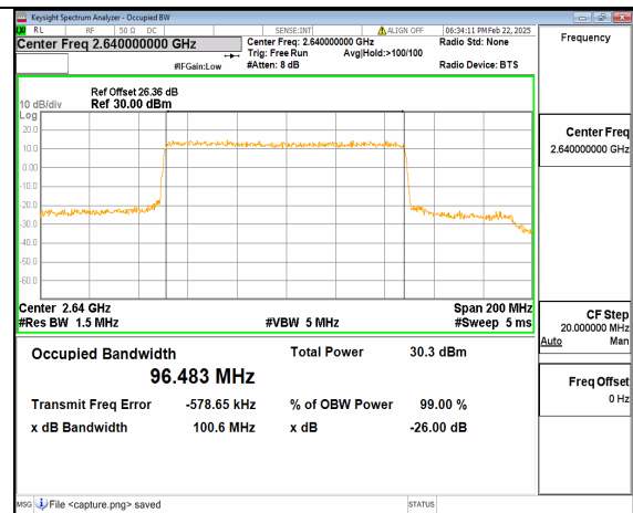
66A_n41 100M CP-OFDM QPSK Outer_Full High
