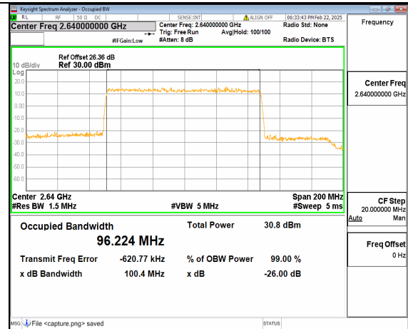
66A_n41 100M DFT-s-OFDM 64QAM Outer_Full High
