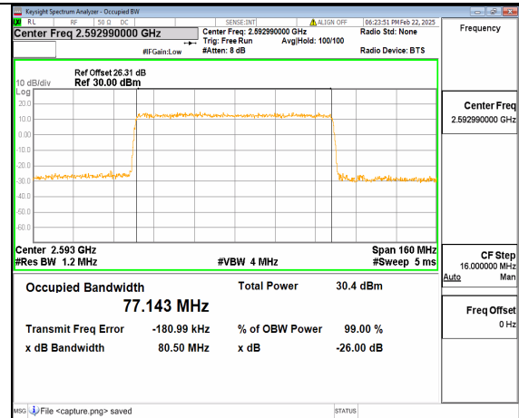
66A_n41 80M DFT-s-OFDM 64QAM Outer_Full Mid
