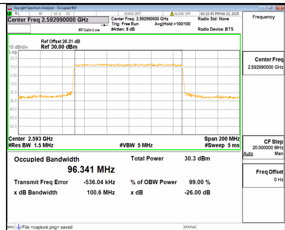
66A_n41 100M CP-OFDM QPSK Outer_Full Mid
