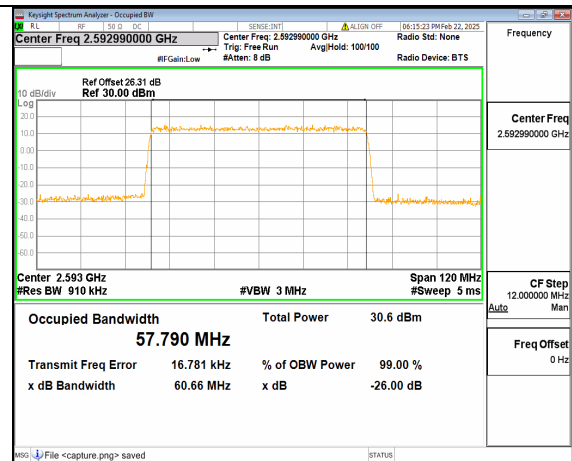
66A_n41 60M DFT-s-OFDM 64QAM Outer_Full Mid
