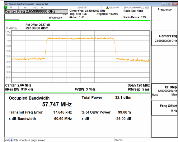
66A_n41 60M DFT-s-OFDM QPSK Outer_Full High
