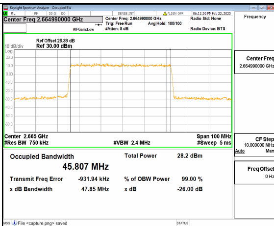
66A_n41 50M DFT-s-OFDM 256QAM Outer_Full High
