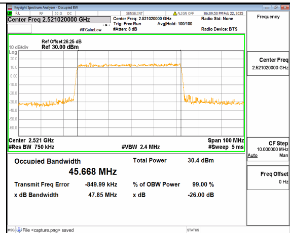
66A_n41 50M DFT-s-OFDM 64QAM Outer_Full Low
