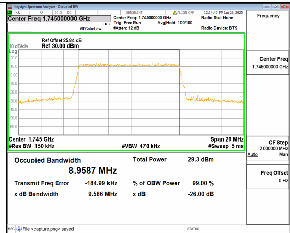
12A_n66 10M DFT-s-OFDM 64QAM Outer_Full Mid
