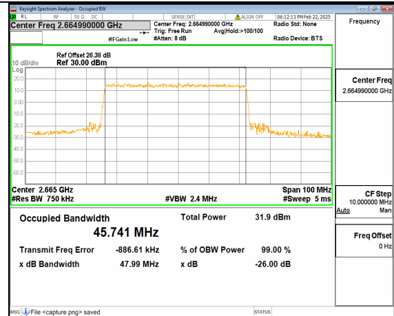
66A_n41 50M DFT-s-OFDM QPSK Outer_Full High
