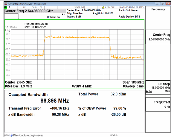
66A_n41 90M DFT-s-OFDM QPSK Outer_Full High
