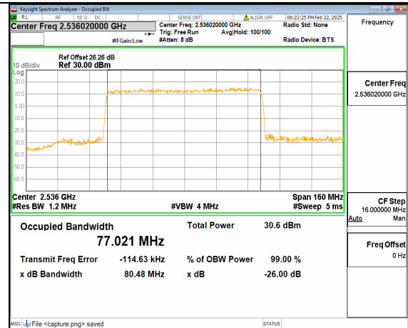
66A_n41 80M DFT-s-OFDM 64QAM Outer_Full Low
