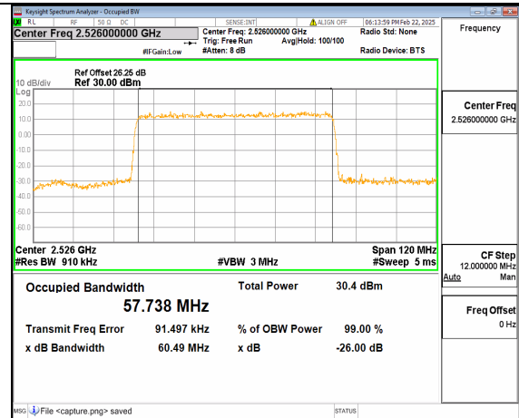
66A_n41 60M DFT-s-OFDM 64QAM Outer_Full Low
