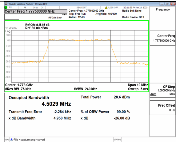
12A_n66 5M DFT-s-OFDM 64QAM Outer_Full High
