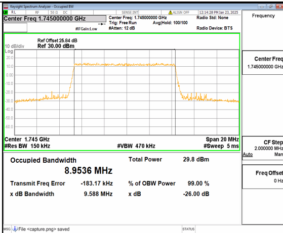
12A_n66 10M DFT-s-OFDM 16QAM Outer_Full Mid
