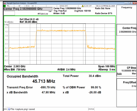
66A_n41 50M DFT-s-OFDM 64QAM Outer_Full Mid
