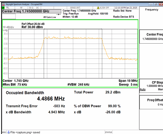
12A_n66 5M DFT-s-OFDM 16QAM Outer_Full Mid
