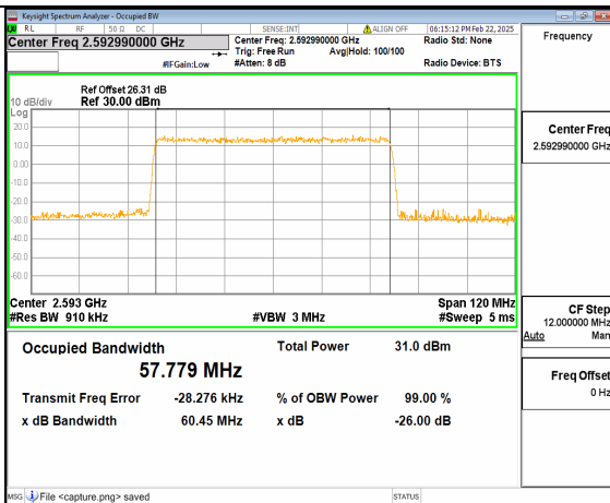
66A_n41 60M DFT-s-OFDM 16QAM Outer_Full Mid
