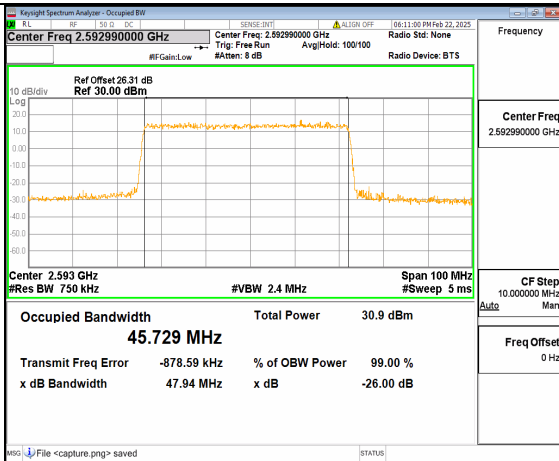
66A_n41 50M DFT-s-OFDM 16QAM Outer_Full Mid
