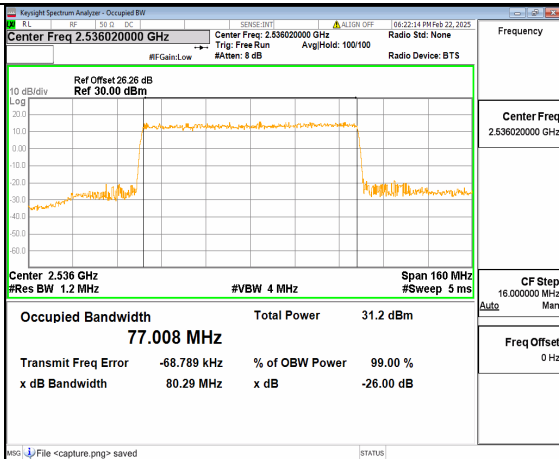
66A_n41 80M DFT-s-OFDM 16QAM Outer_Full Low
