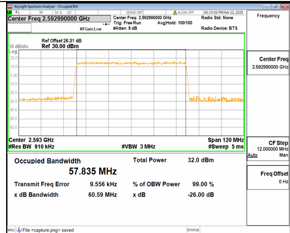
66A_n41 60M DFT-s-OFDM QPSK Outer_Full Mid
