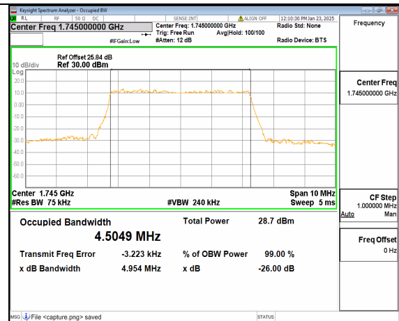
12A_n66 5M DFT-s-OFDM 64QAM Outer_Full Mid
