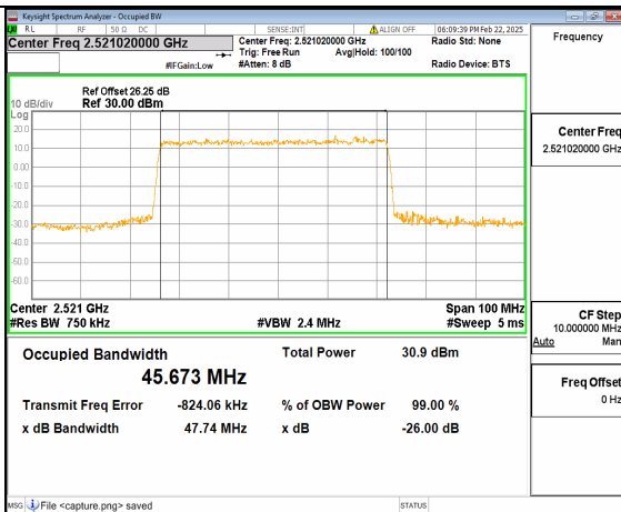
66A_n41 50M DFT-s-OFDM 16QAM Outer_Full Low
