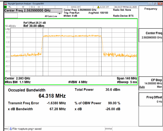
66A_n41 70M DFT-s-OFDM 64QAM Outer_Full Mid
