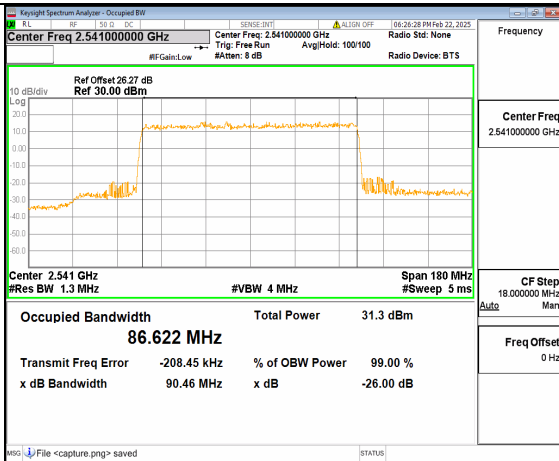
66A_n41 90M DFT-s-OFDM 16QAM Outer_Full Low
