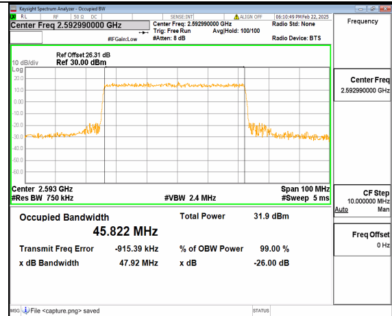
66A_n41 50M DFT-s-OFDM QPSK Outer_Full Mid
