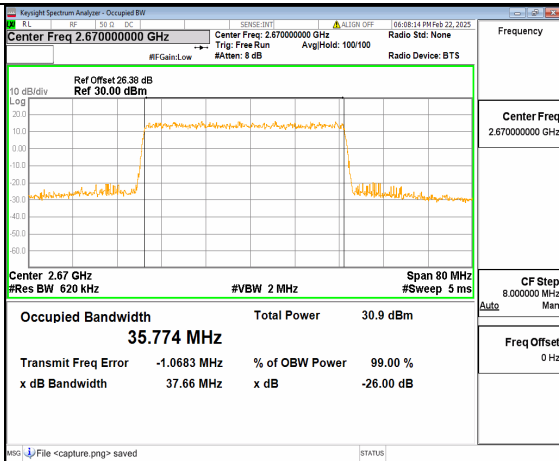
66A_n41 40M DFT-s-OFDM 16QAM Outer_Full High
