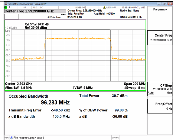
66A_n41 100M DFT-s-OFDM 64QAM Outer_Full Mid
