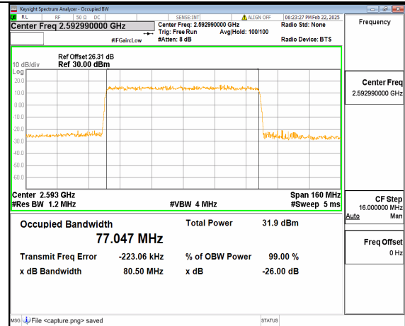
66A_n41 80M DFT-s-OFDM QPSK Outer_Full Mid
