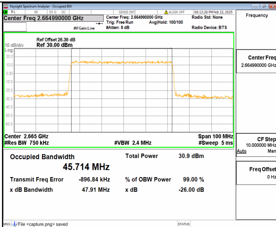
66A_n41 50M DFT-s-OFDM 16QAM Outer_Full High
