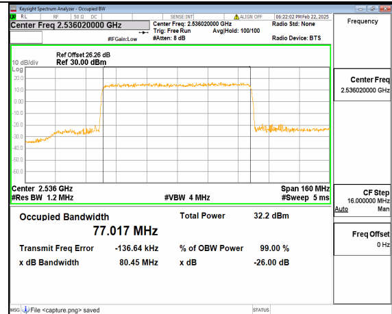
66A_n41 80M DFT-s-OFDM QPSK Outer_Full Low
