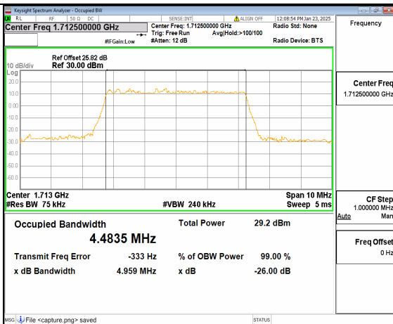
12A_n66 5M DFT-s-OFDM 16QAM Outer_Full Low
