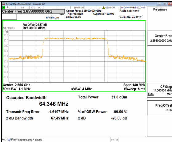
66A_n41 70M DFT-s-OFDM 16QAM Outer_Full High
