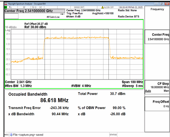
66A_n41 90M DFT-s-OFDM 64QAM Outer_Full Low
