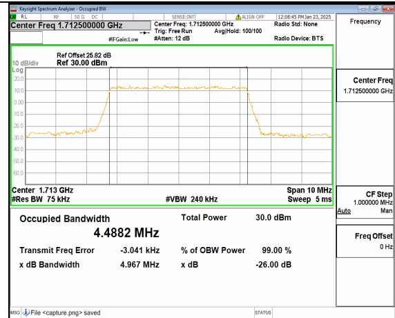
12A_n66 5M DFT-s-OFDM QPSK Outer_Full Low
