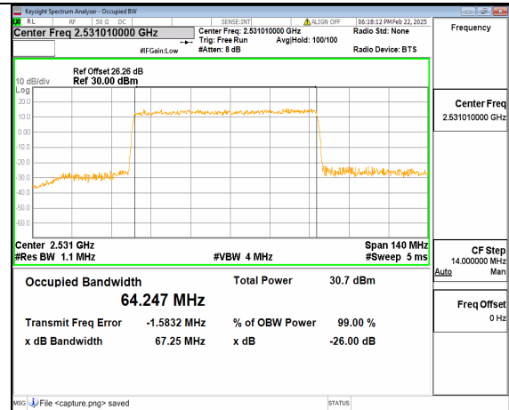
66A_n41 70M DFT-s-OFDM 64QAM Outer_Full Low
