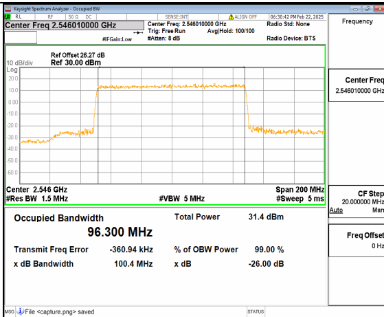
66A_n41 100M DFT-s-OFDM 16QAM Outer_Full Low
