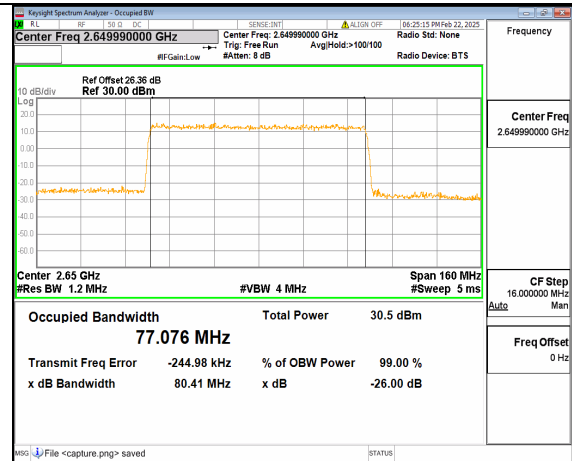
66A_n41 80M DFT-s-OFDM 64QAM Outer_Full High
