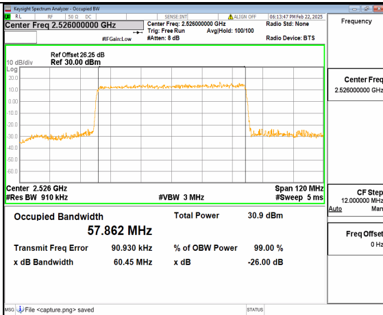
66A_n41 60M DFT-s-OFDM 16QAM Outer_Full Low
