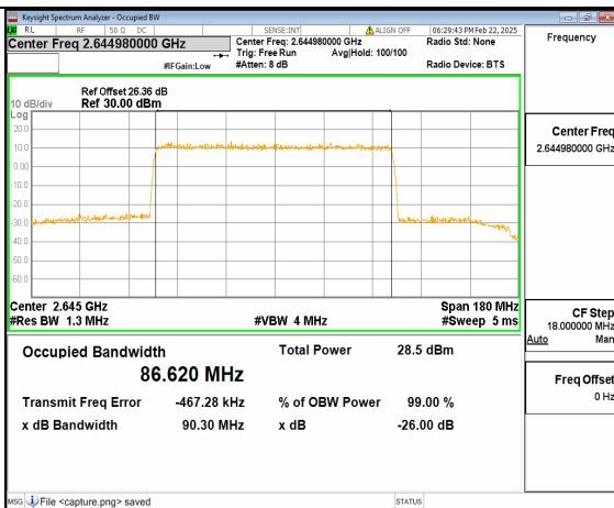
66A_n41 90M DFT-s-OFDM 256QAM Outer_Full High
