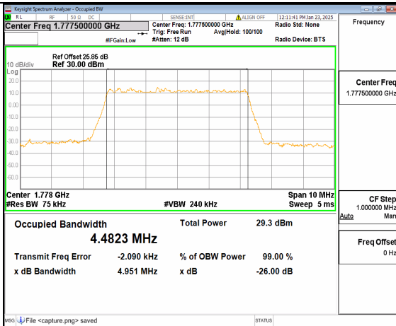
12A_n66 5M DFT-s-OFDM 16QAM Outer_Full High
