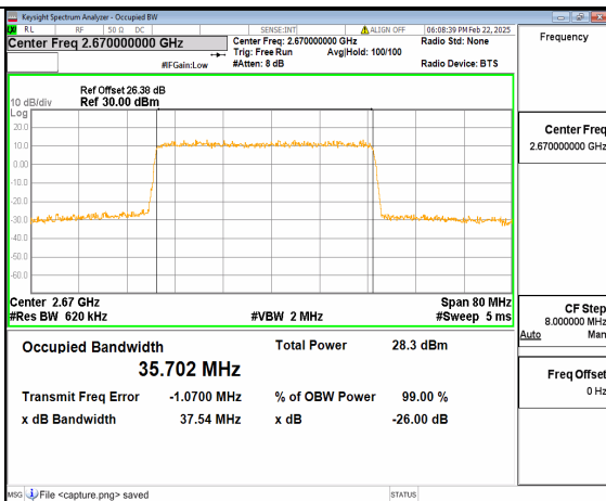
66A_n41 40M DFT-s-OFDM 256QAM Outer_Full High
