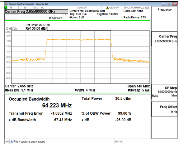
66A_n41 70M DFT-s-OFDM 64QAM Outer_Full High
