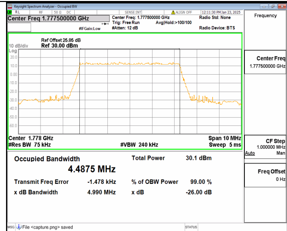
12A_n66 5M DFT-s-OFDM QPSK Outer_Full High
