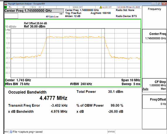
12A_n66 5M DFT-s-OFDM QPSK Outer_Full Mid
