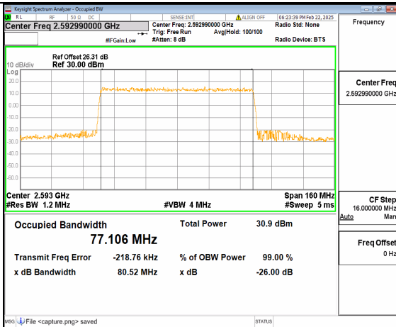
66A_n41 80M DFT-s-OFDM 16QAM Outer_Full Mid
