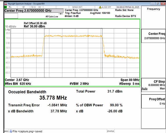
66A_n41 40M DFT-s-OFDM QPSK Outer_Full High
