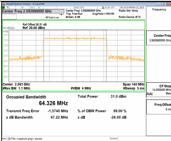
66A_n41 70M DFT-s-OFDM 16QAM Outer_Full Mid
