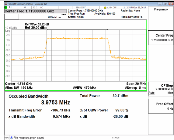
12A_n66 10M DFT-s-OFDM QPSK Outer_Full Low
