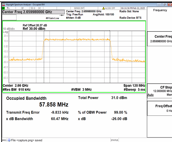
66A_n41 60M DFT-s-OFDM 16QAM Outer_Full High
