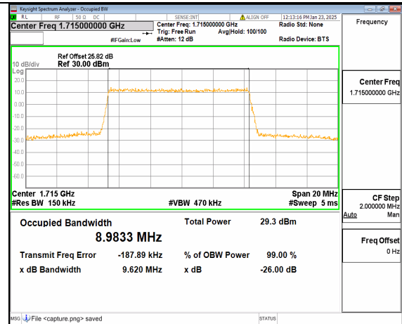
12A_n66 10M DFT-s-OFDM 64QAM Outer_Full Low
