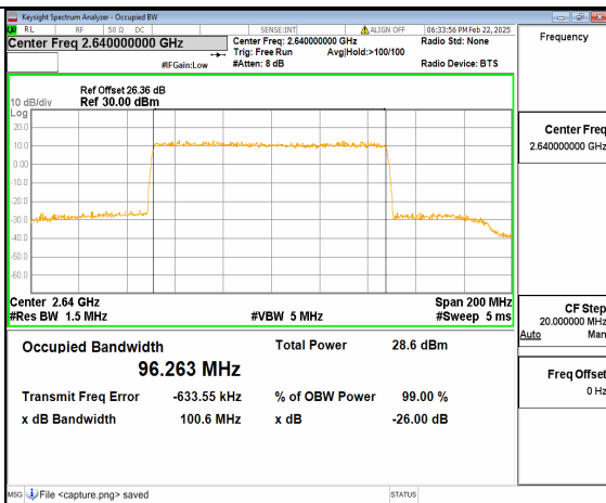
66A_n41 100M DFT-s-OFDM 256QAM Outer_Full High
