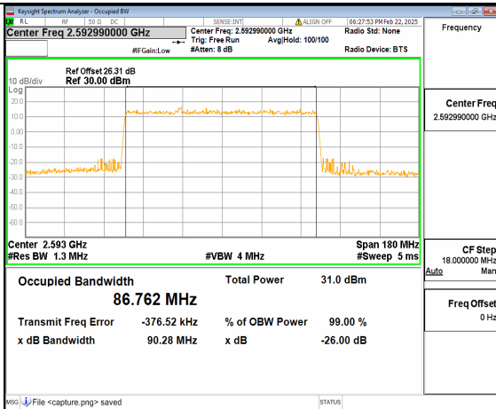
66A_n41 90M DFT-s-OFDM 16QAM Outer_Full Mid
