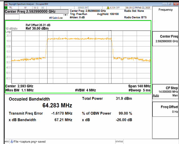
66A_n41 70M DFT-s-OFDM QPSK Outer_Full Mid
