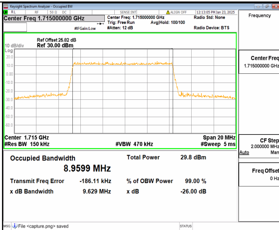
12A_n66 10M DFT-s-OFDM 16QAM Outer_Full Low
