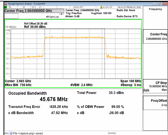
66A_n41 50M DFT-s-OFDM 64QAM Outer_Full High
