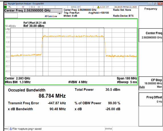
66A_n41 90M DFT-s-OFDM 64QAM Outer_Full Mid
