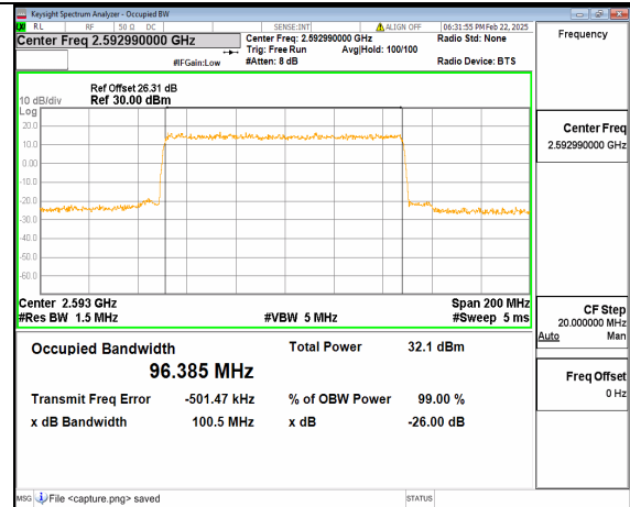
66A_n41 100M DFT-s-OFDM QPSK Outer_Full Mid
