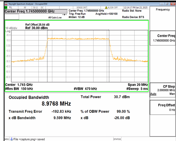
12A_n66 10M DFT-s-OFDM QPSK Outer_Full Mid
