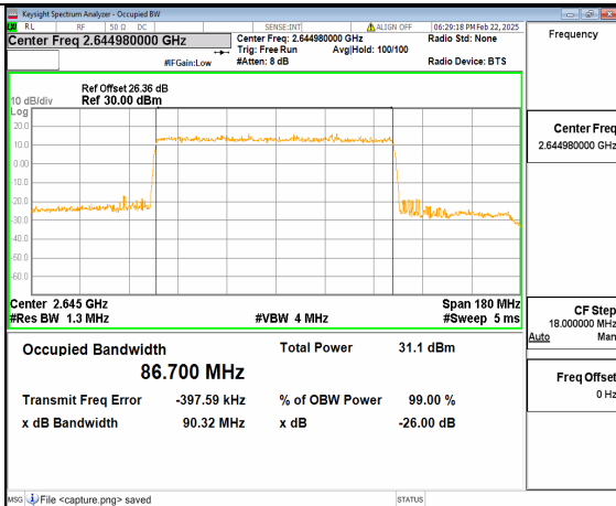
66A_n41 90M DFT-s-OFDM 16QAM Outer_Full High
