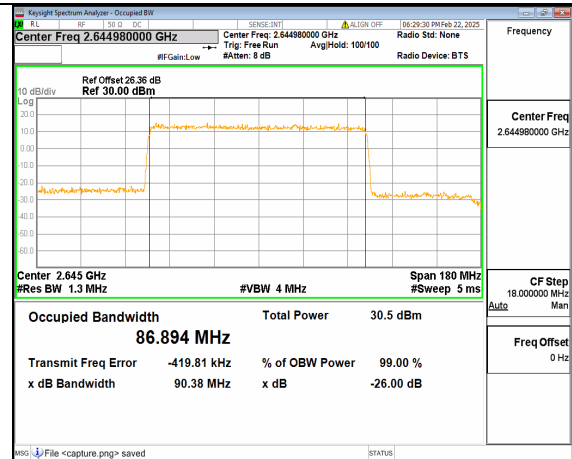
66A_n41 90M DFT-s-OFDM 64QAM Outer_Full High
