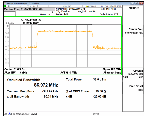
66A_n41 90M DFT-s-OFDM QPSK Outer_Full Mid
