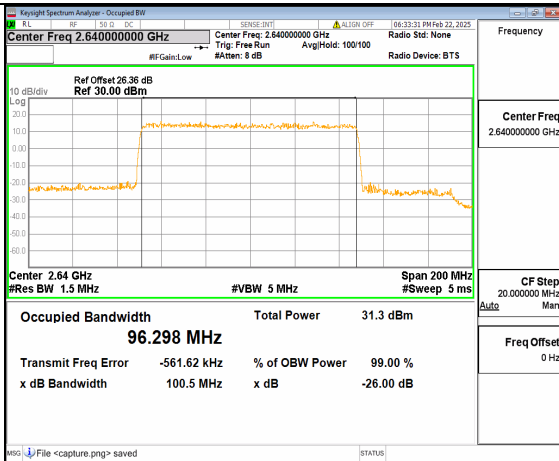
66A_n41 100M DFT-s-OFDM 16QAM Outer_Full High
