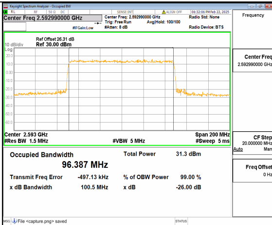
66A_n41 100M DFT-s-OFDM 16QAM Outer_Full Mid
