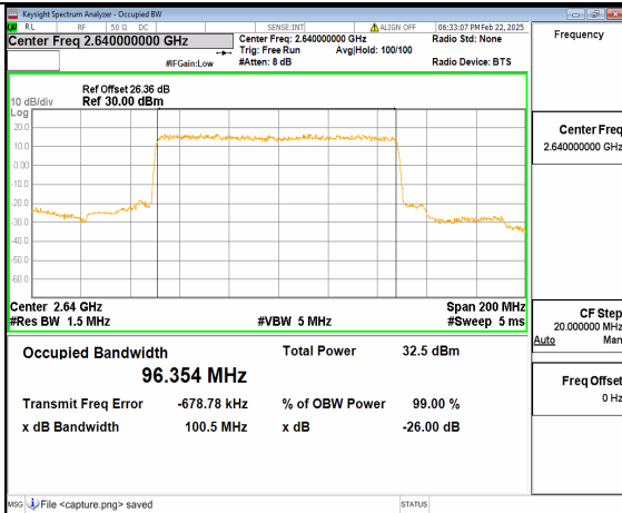
66A_n41 100M DFT-s-OFDM BPSK Outer_Full High
