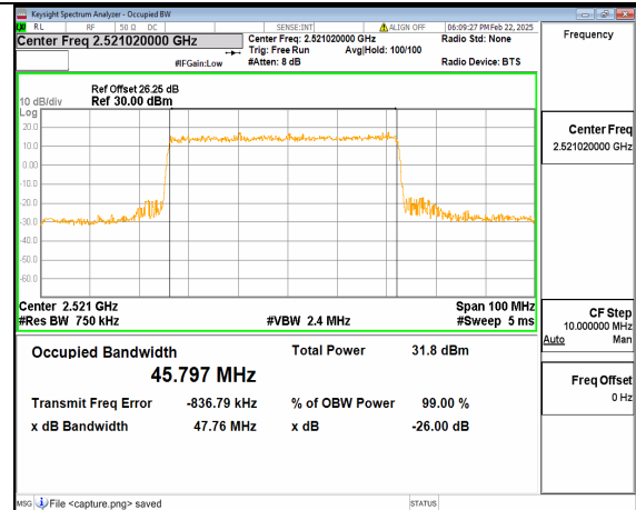
66A_n41 50M DFT-s-OFDM QPSK Outer_Full Low
