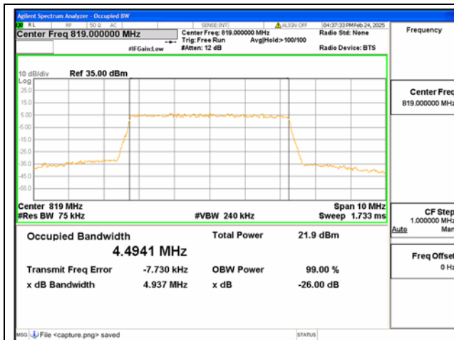
B26 Part90 / 5MHz / 64QAM/ Mid CH
