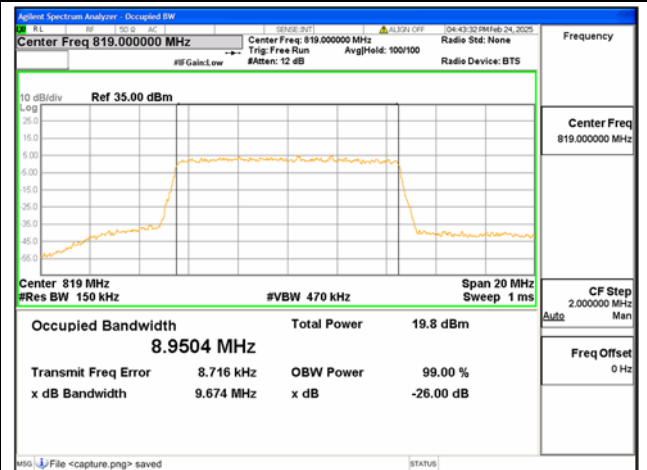
B26 Part90 / 10MHz / 256QAM/ High CH
