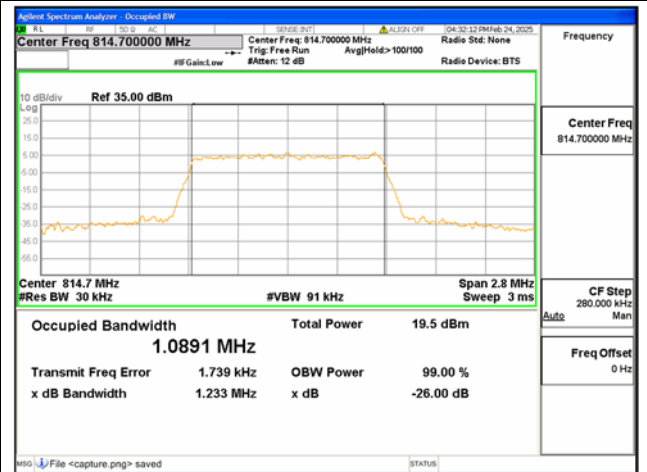
B26 Part90 / 1.4MHz / 256QAM/ Low CH
