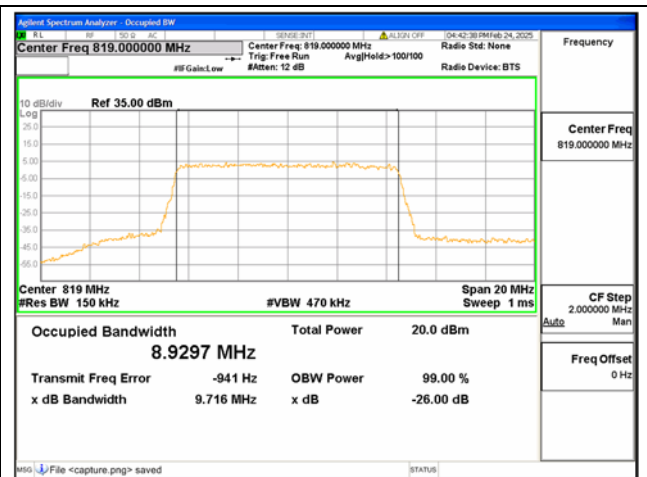
B26 Part90 / 10MHz / 256QAM/ Mid CH
