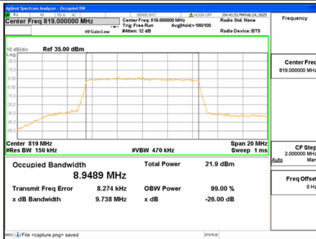
B26 Part90 / 10MHz / 64QAM/ Low CH
