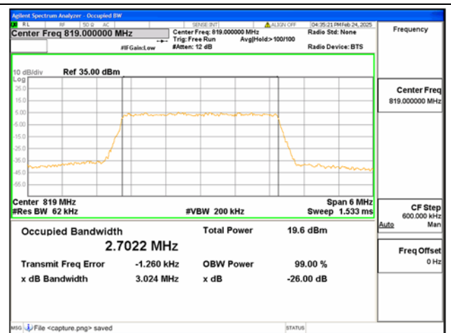
B26 Part90 / 3MHz / 256QAM/ Mid CH
