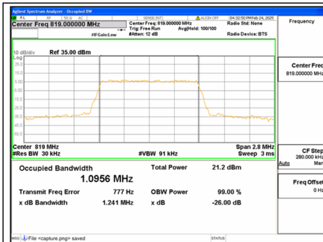
B26 Part90 / 1.4MHz / 64QAM/ Mid CH
