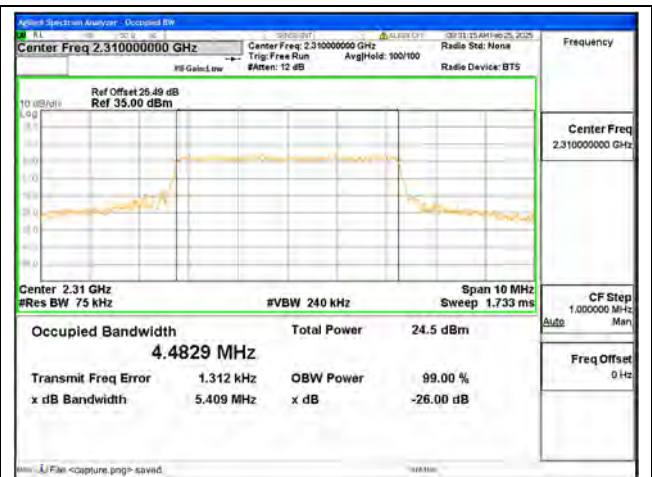
B40-1 / 5MHz / 256QAM/ Mid CH
