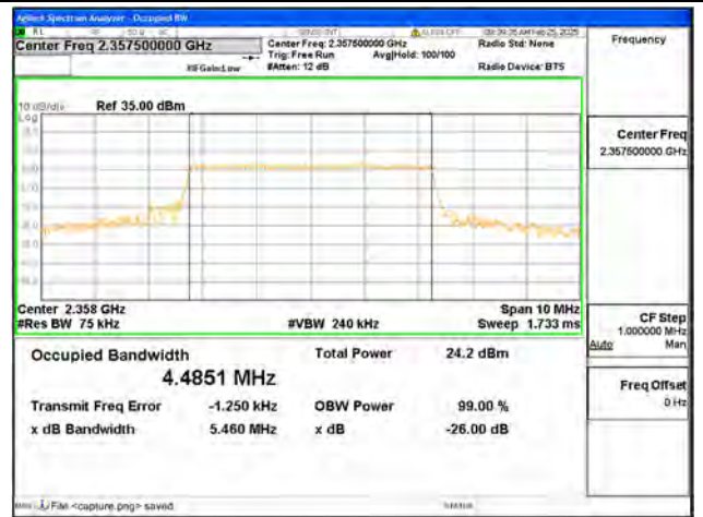
B40-2 / 5MHz / 256QAM/ High CH
