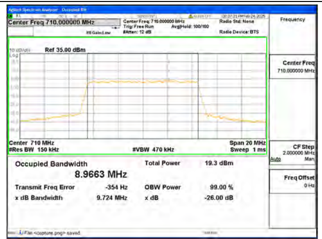
B17 / 10MHz / 256QAM/ Mid CH
