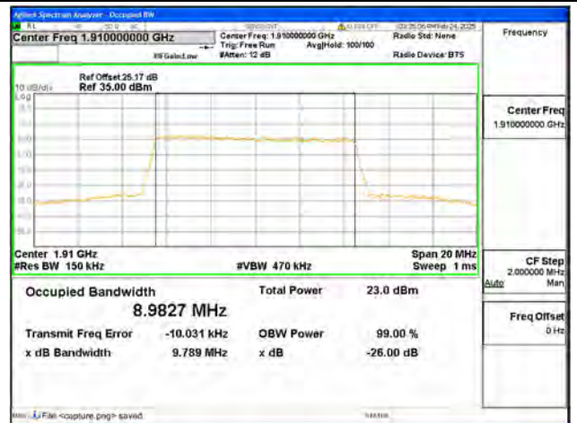
B25 / 10MHz / 256QAM/ High CH
