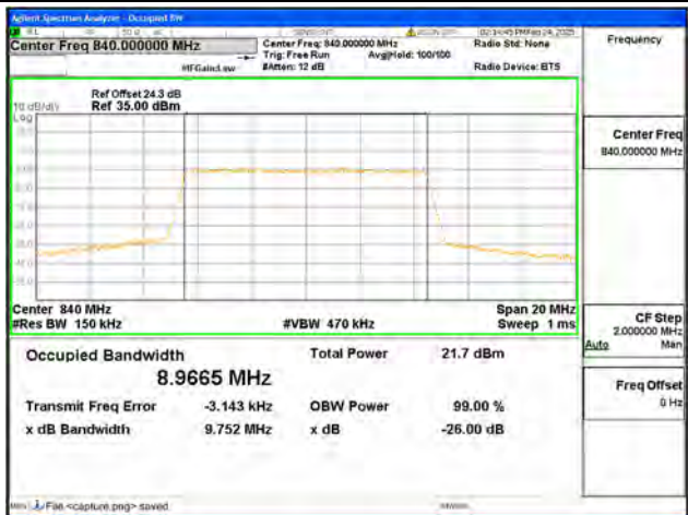
B19 / 10MHz / 64QAM/ High CH
