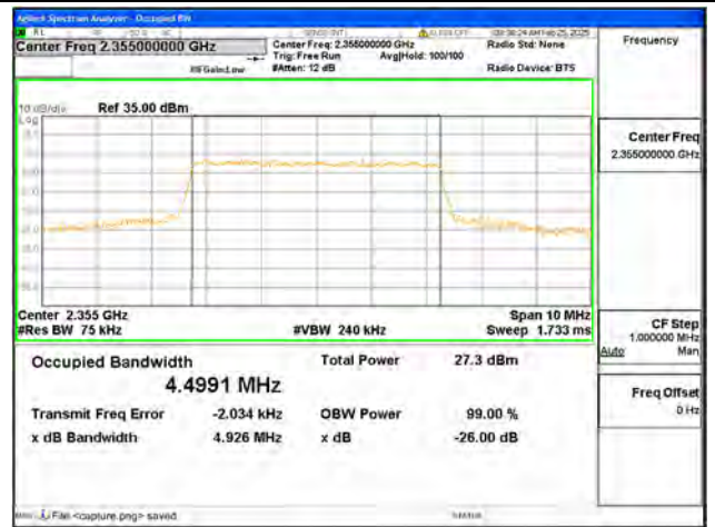
B40-2 / 5MHz / 16QAM/ Mid CH
