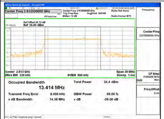
B38 / 15MHz / 256QAM/ High CH
