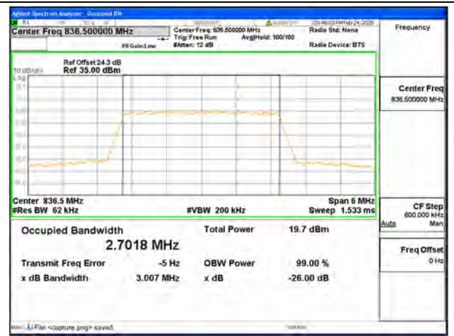
B26 / 3MHz / 256QAM/ Mid CH
