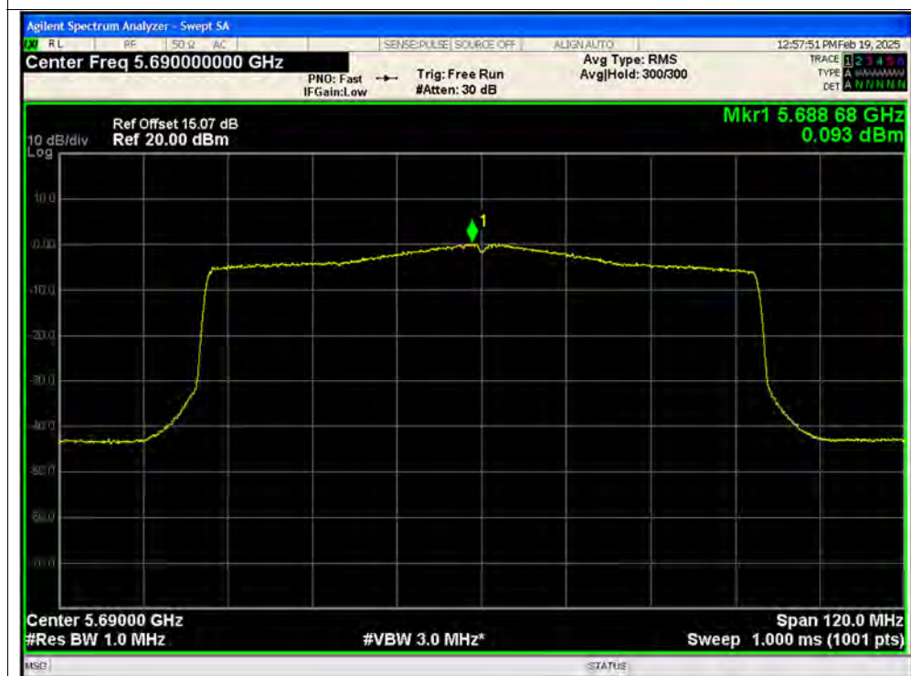
PSD NVNT ax80 5690MHz Ant1 SISO
