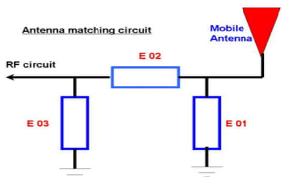
匹配电路图(没修改)/ Matching circuit diagram (not modified)
