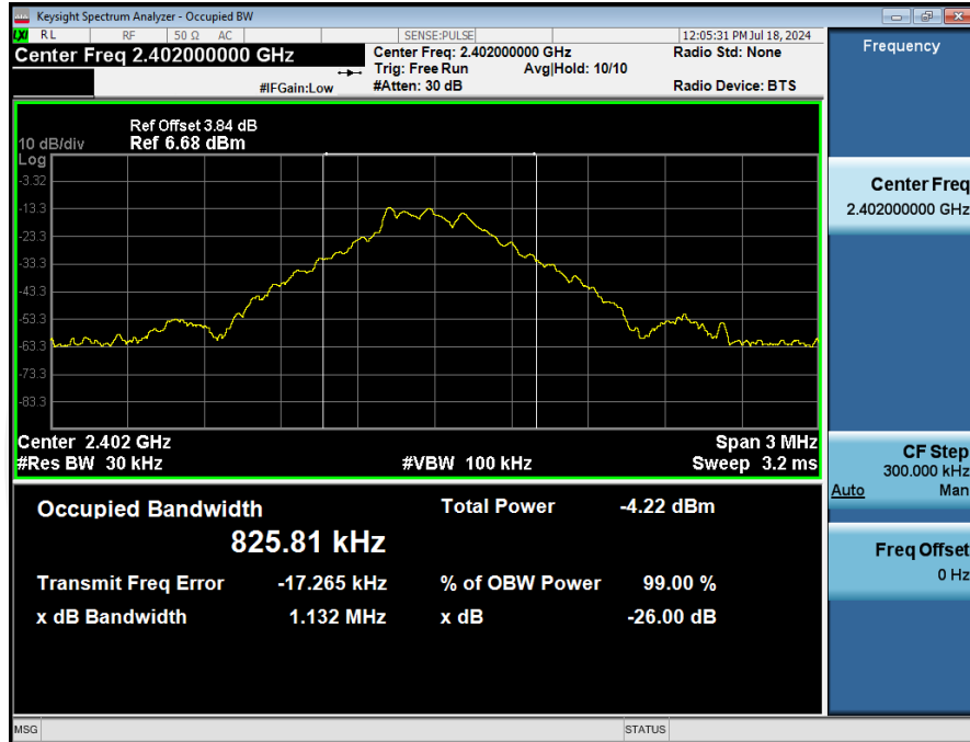
99%_Occupied_Bandwidth_NVNT_ANT1_1-DH1_2402
