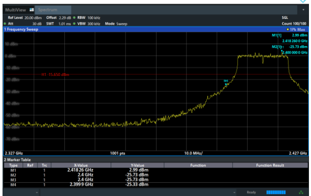
802.11g: Band Edge, Left Side
