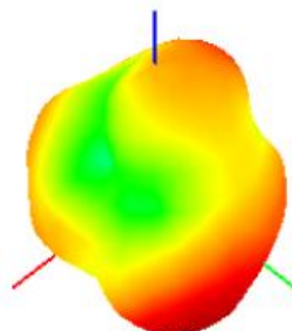
2460.00MHz@T45P45
