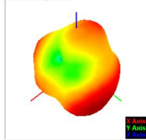
2440.00MHz@T45P45
