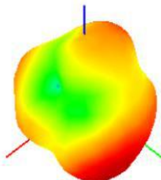
2450.00MHz@T45P45
