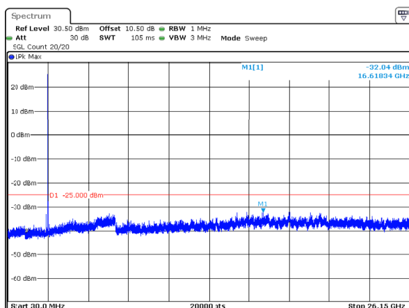
10MHz_High_QPSK_1@0 -32.04dBm
