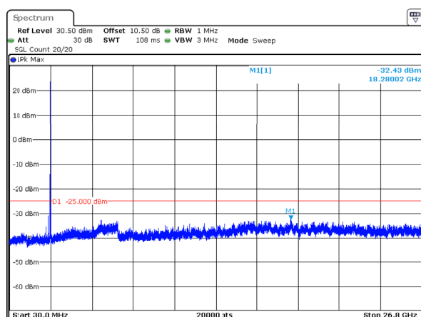
20MHz_High_QPSK_1@0 -32.43dBm
