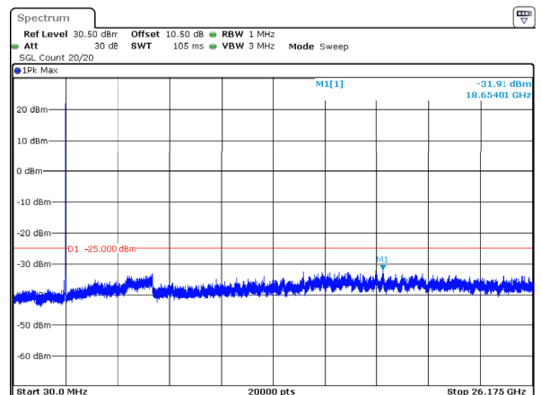
5MHz_High_QPSK_25@0 -31.91dBm
