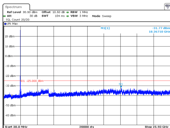
20MHz_Middle_QPSK_1@0 -31.77dBm
