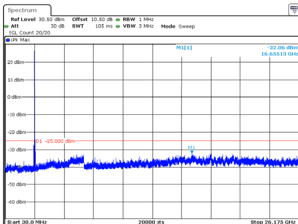
5MHz_High_QPSK_1@0 -32.06dBm
