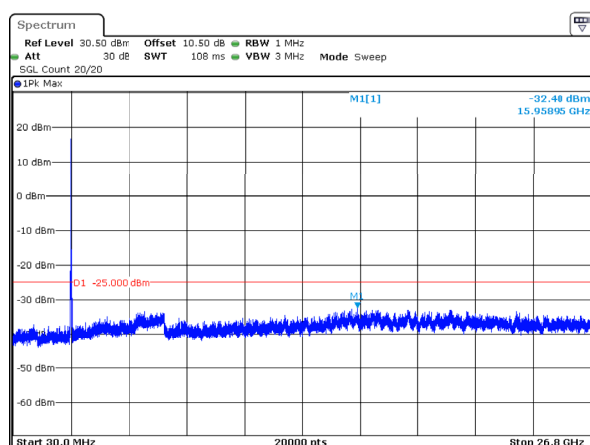
20MHz_High_QPSK_100@0 -32.40dBm
