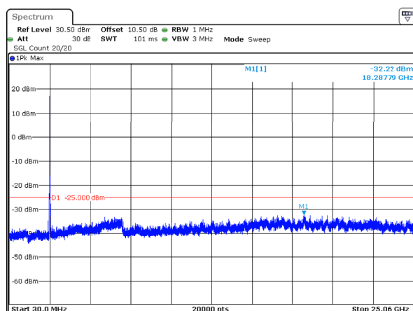
20MHz_Low_QPSK_100@0 -32.22dBm
