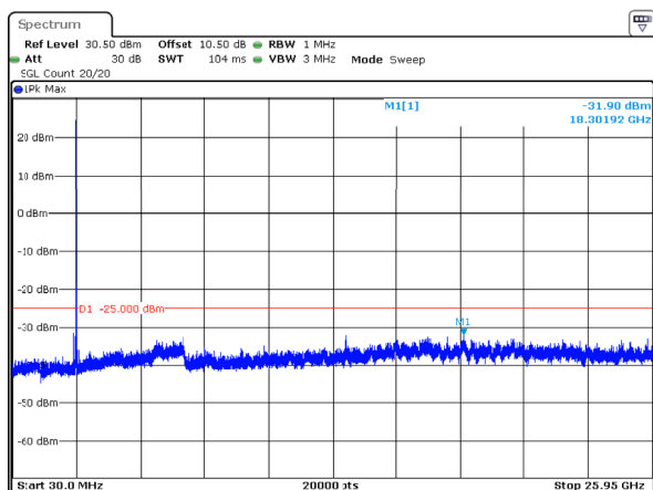
20MHz_Middle_QPSK_1@0 -31.90dBm
