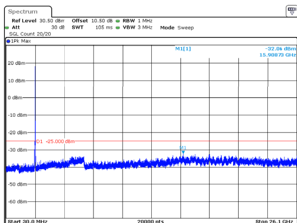
20MHz_High_QPSK_100@0 -32.06dBm
