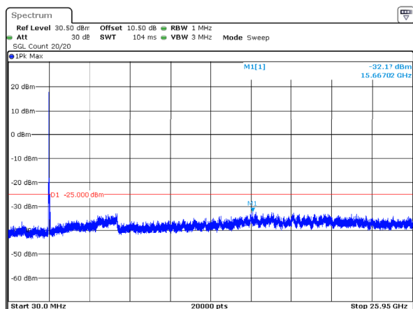
20MHz_Middle_QPSK_100@0 -32.17dBm
