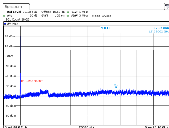
10MHz_High_QPSK_50@0 -32.07dBm
