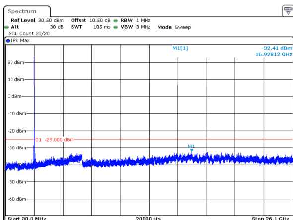
20MHz_High_QPSK_1@0 -32.41dBm
