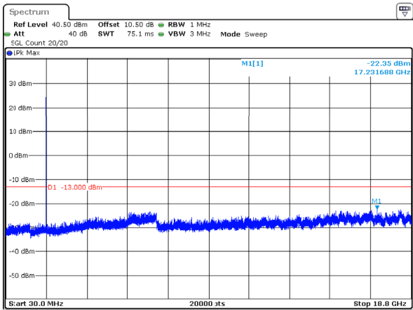
1.4MHz_Middle_QPSK_1@0
