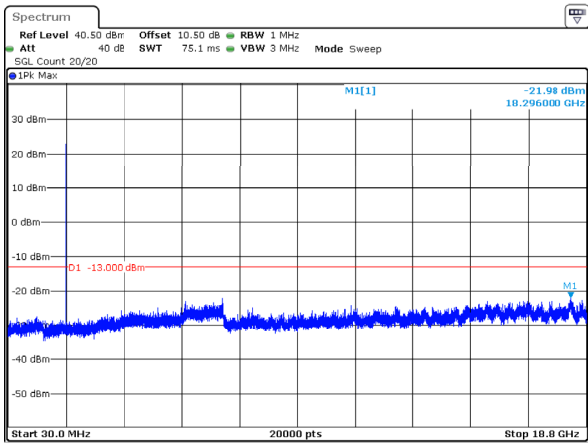
1.4MHz_Middle_QPSK_6@0
