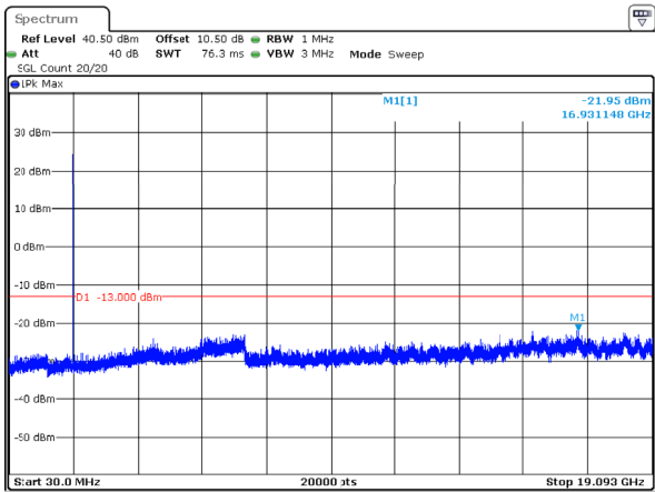
1.4MHz_High_QPSK_1@0
