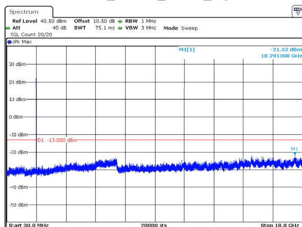
3MHz_Middle_QPSK_1@0
