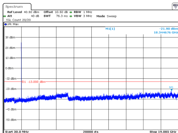
3MHz_High_QPSK_1@0
