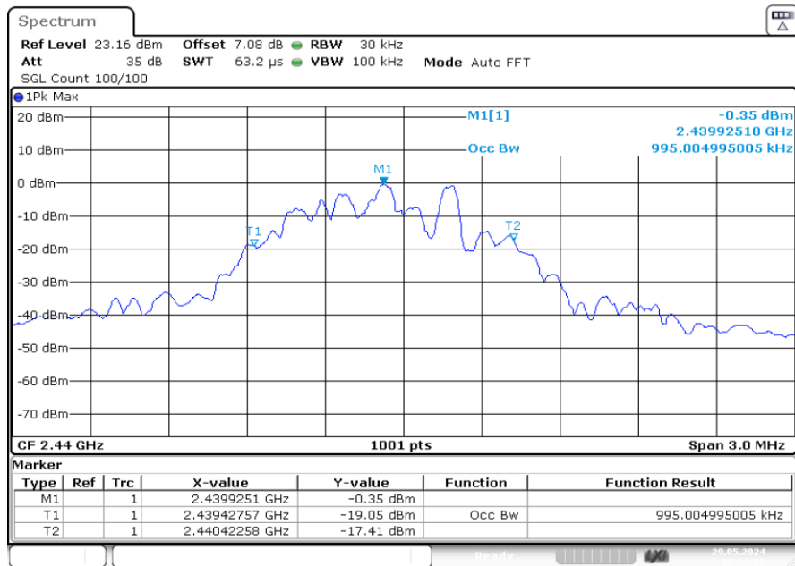
99%_Occupied_Bandwidth_NVNT_ANT1_GFSK_2440
