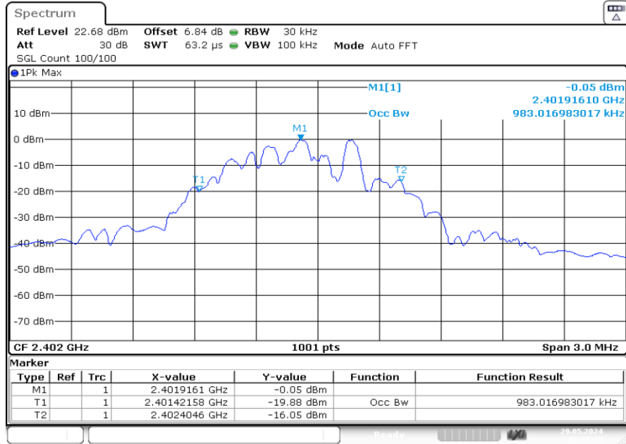
99%_Occupied_Bandwidth_NVNT_ANT1_GFSK_2402
