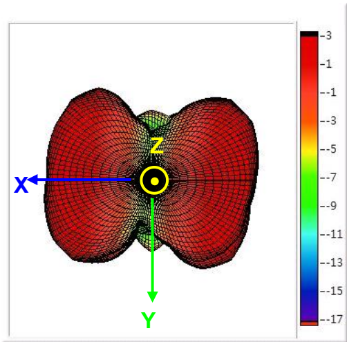
7-2-2. 3D Gain Pattern @ 5550 MHz (unit: dBi)
