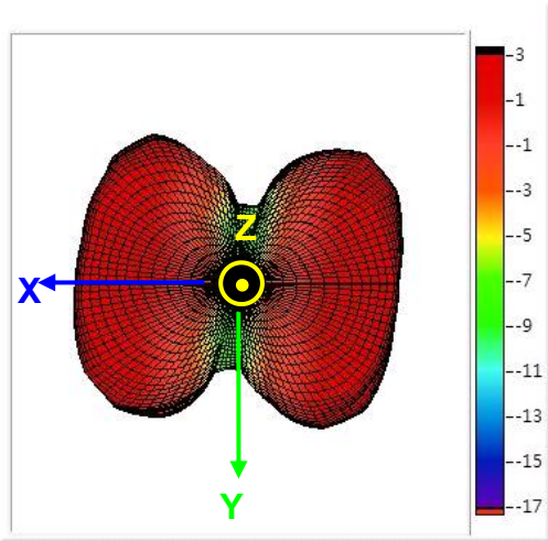
7-2-3. 3D Gain Pattern @ 5850 MHz (unit: dBi)
