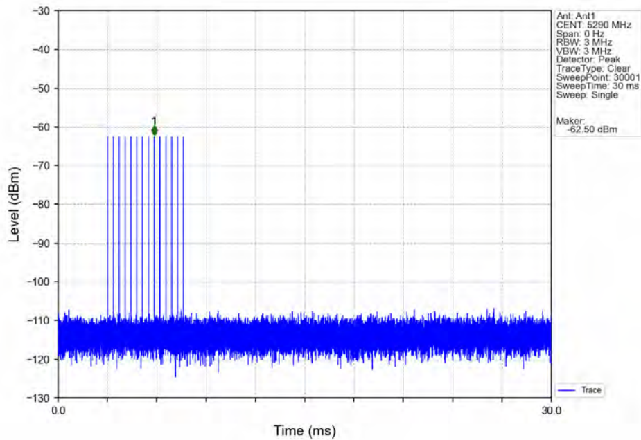
Signal Calibration_802.11ax(HEW80)_2A_5290MHz_RadarType5_Trial0
