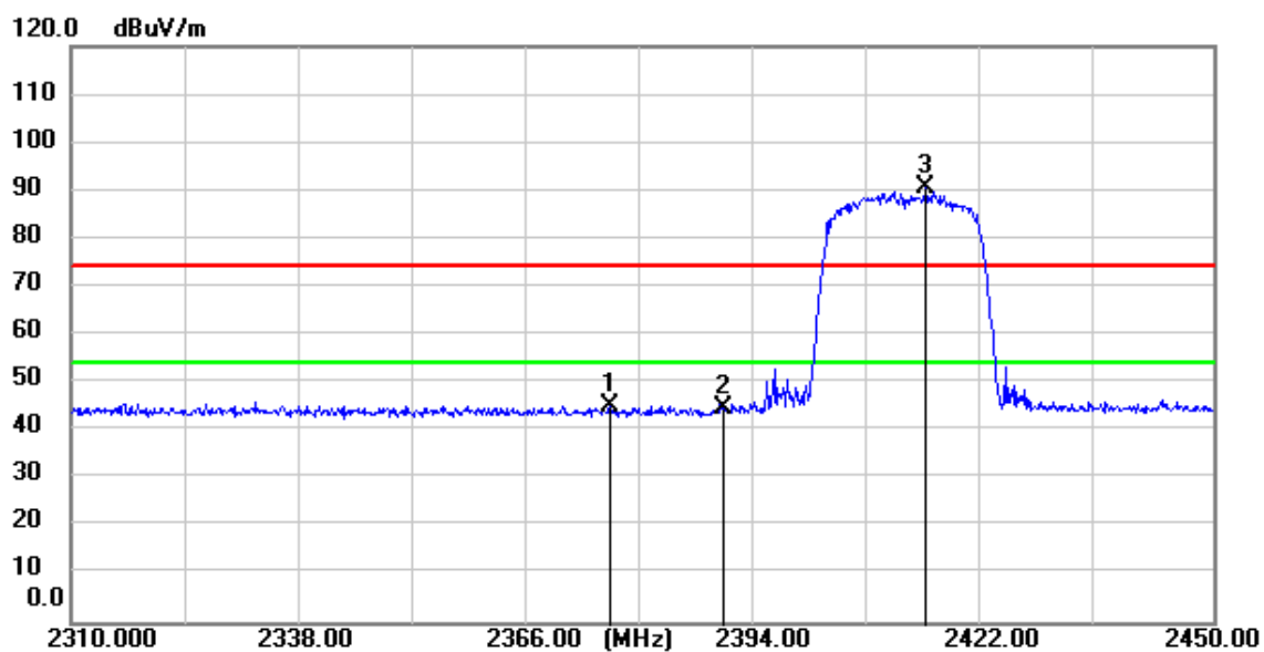
11ax(HE20)_TX_CH_01_Horizontal_Peak
