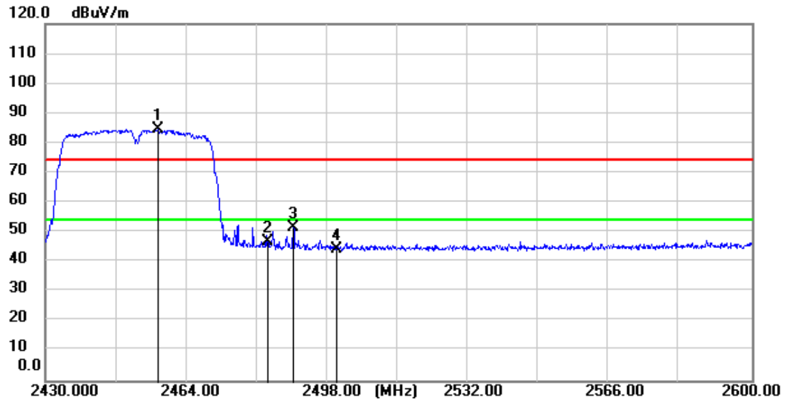
11n(HT40)_TX_CH_09_Horizontal_Peak
