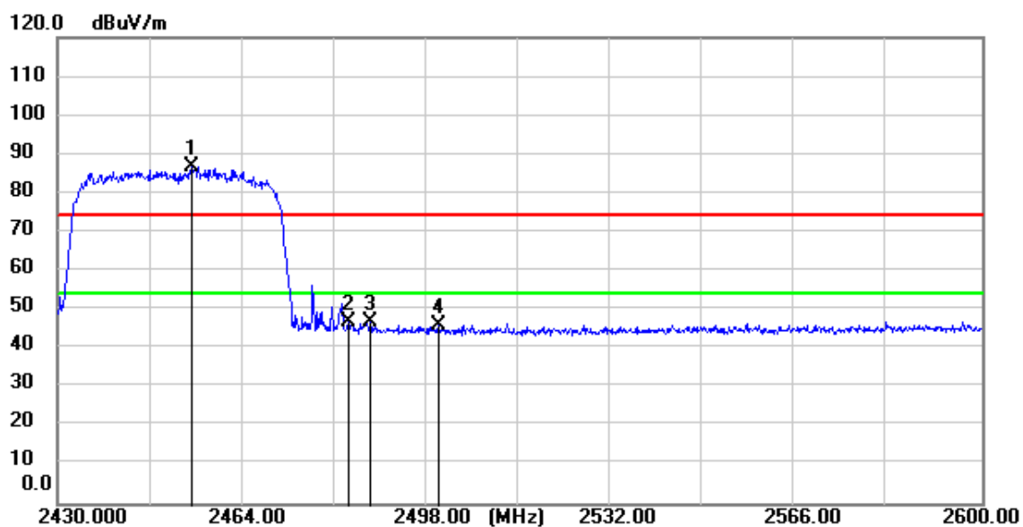
11ax(HE40)_TX_CH_09_Horizontal_Peak
