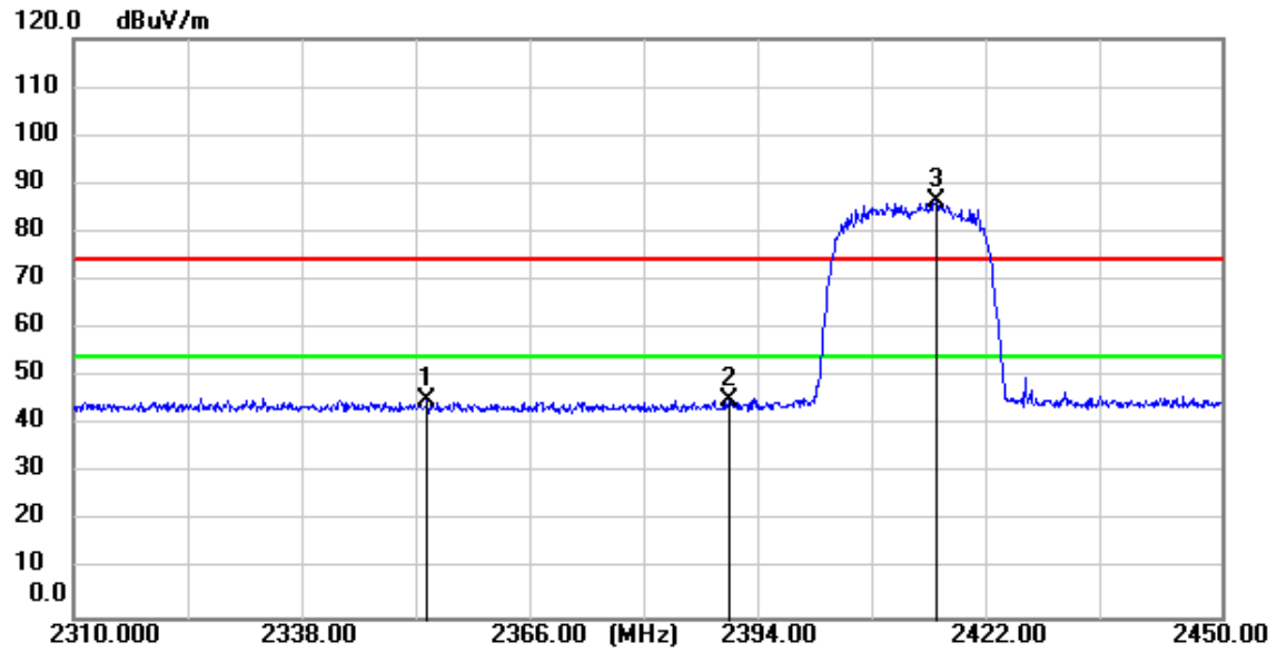
11ax(HE20)_TX_CH_01_Vertical_Peak
