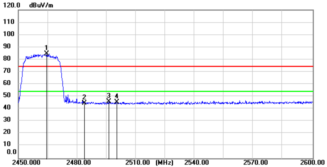
11ax(HE20)_TX_CH_11_Vertical_Peak
