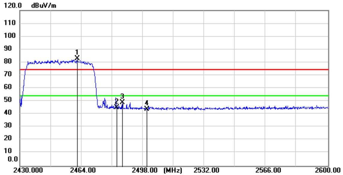
11ax(HE40)_TX_CH_09_Vertical_Peak
