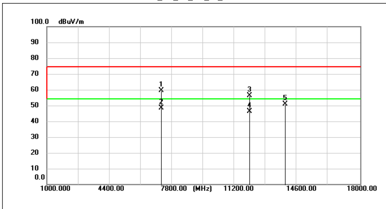
BLE_1M_TX_CH_19_Verical
