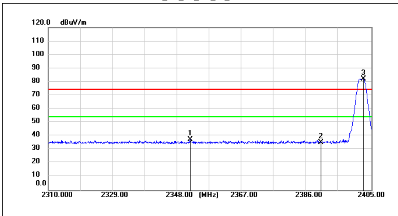
BLE_2M_TX_CH_00_Verical
