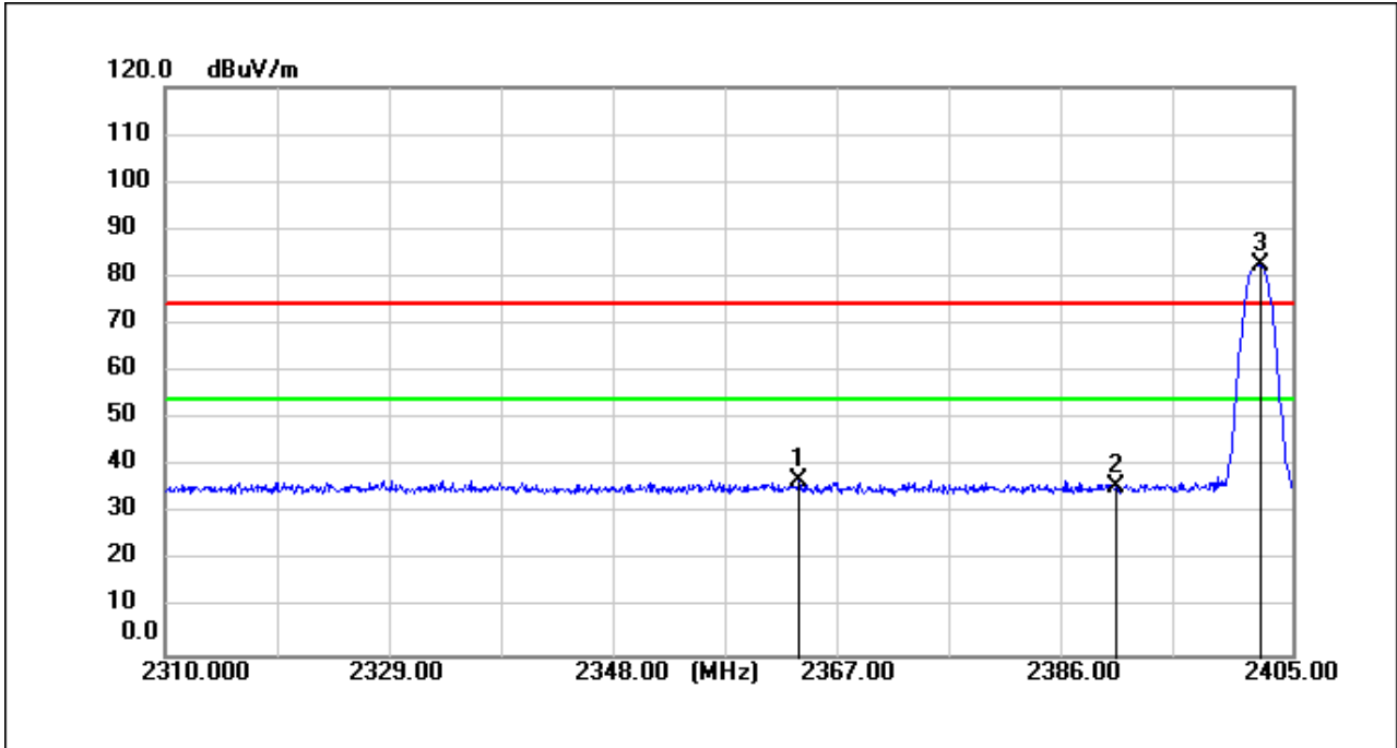
BLE_1M_TX_CH_00_Vertical_Peak
