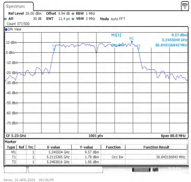
11N40SISO-Ant1-5230
