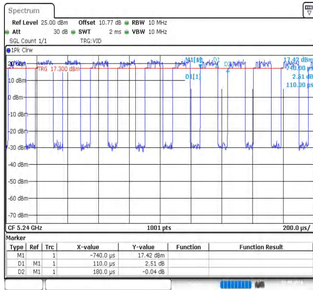
NTNV-11N20SISO-Ant1-5240
