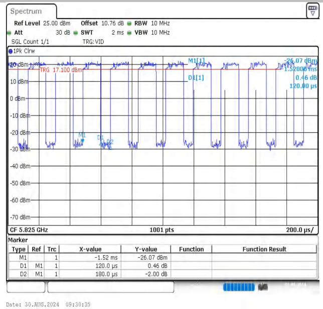
NTNV-11N20SISO-Ant1-5825
