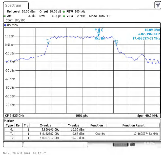
11A-Ant1-5825
