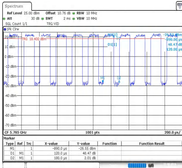
NTNV-11A-Ant1-5785
