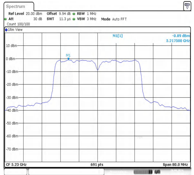
11N40SISO-Ant1-5230-PASS
