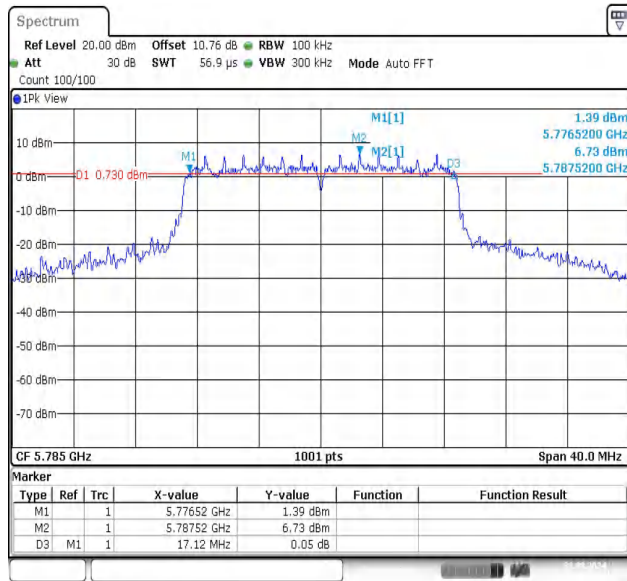
11N20SISO-Ant1-5785-PASS
