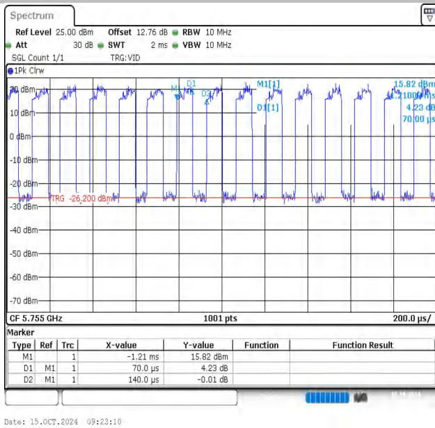
NTNV-11N40SISO-Ant1-5755
