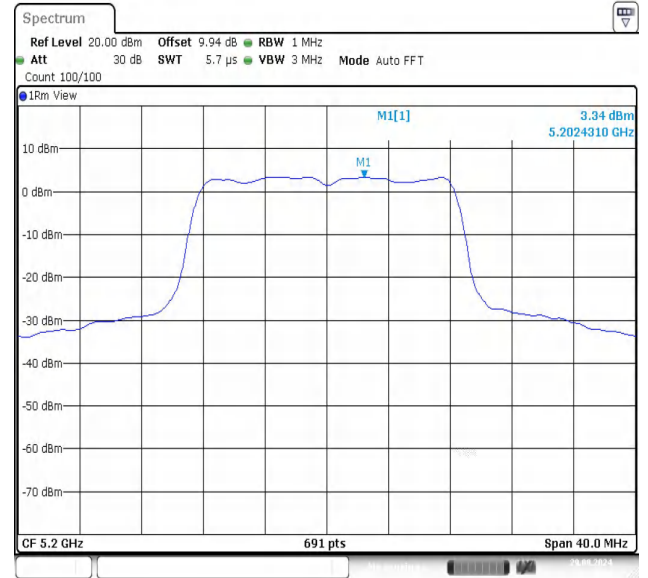
11A-Ant1-5200-PASS
