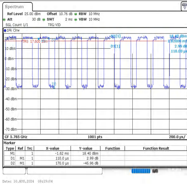
NTNV-11N20SISO-Ant1-5785
