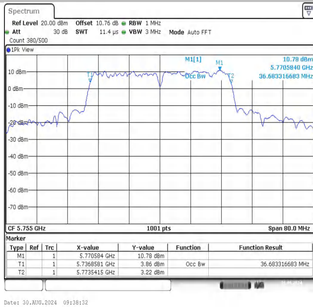
11N40SISO-Ant1-5755
