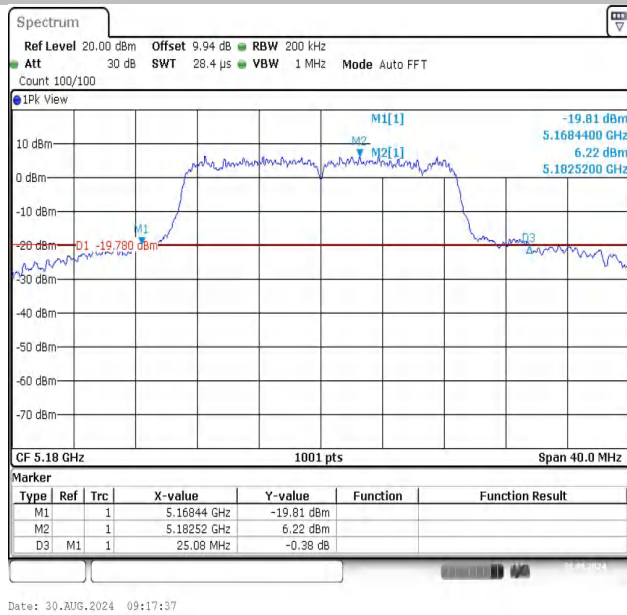
11N20SISO-Ant1-5180
