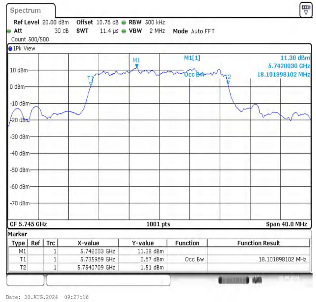
11N20SISO-Ant1-5745
