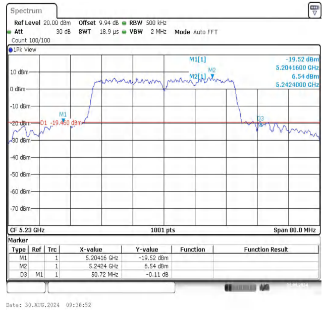
11N40SISO-Ant1-5230
