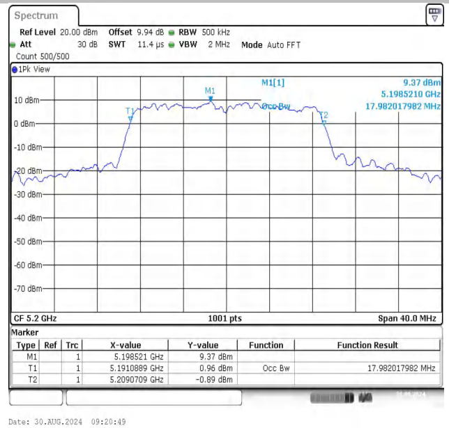
11N20SISO-Ant1-5200
