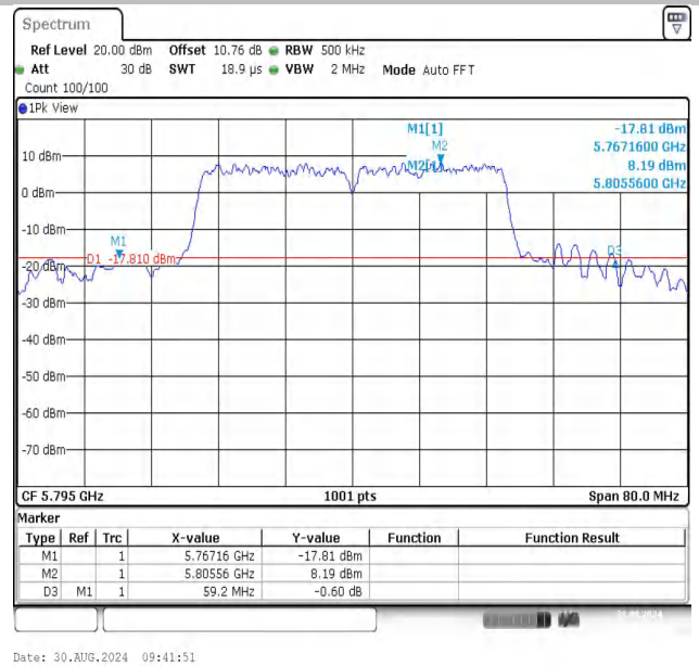
11N40SISO-Ant1-5795
