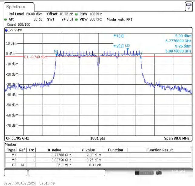
11N40SISO-Ant1-5795-PASS
