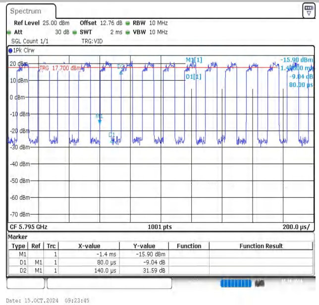
NTNV-11N40SISO-Ant1-5795
