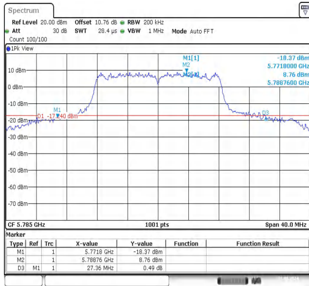
11A-Ant1-5785
