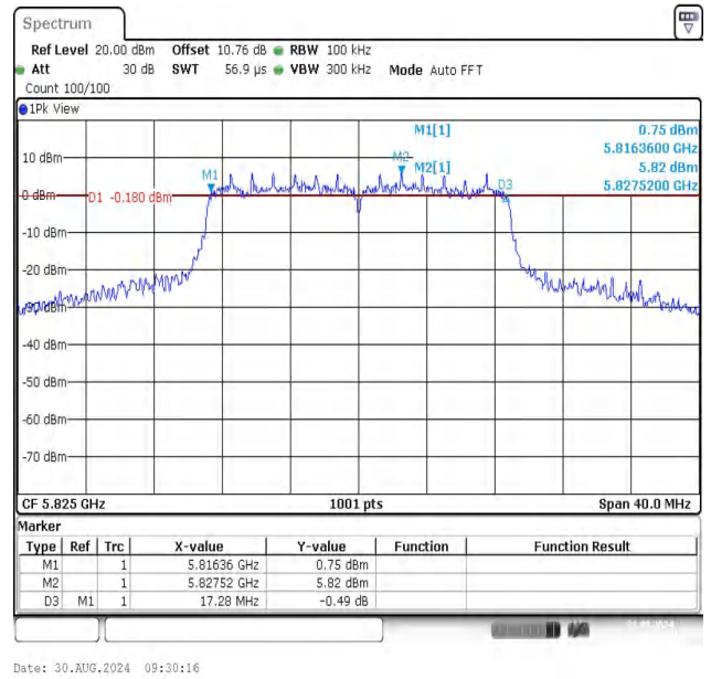
11N20SISO-Ant1-5825-PASS
