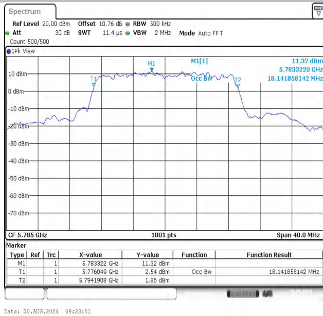
11N20SISO-Ant1-5785
