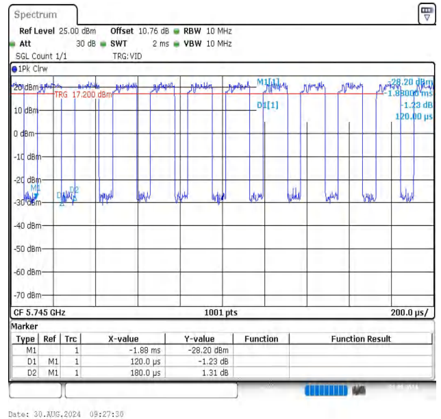
NTNV-11N20SISO-Ant1-5745
