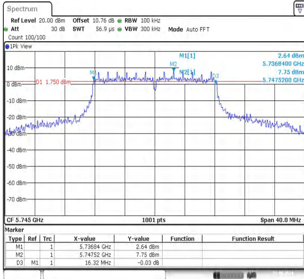
11A-Ant1-5745-PASS
