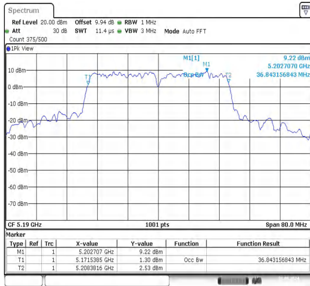
11N40SISO-Ant1-5190
