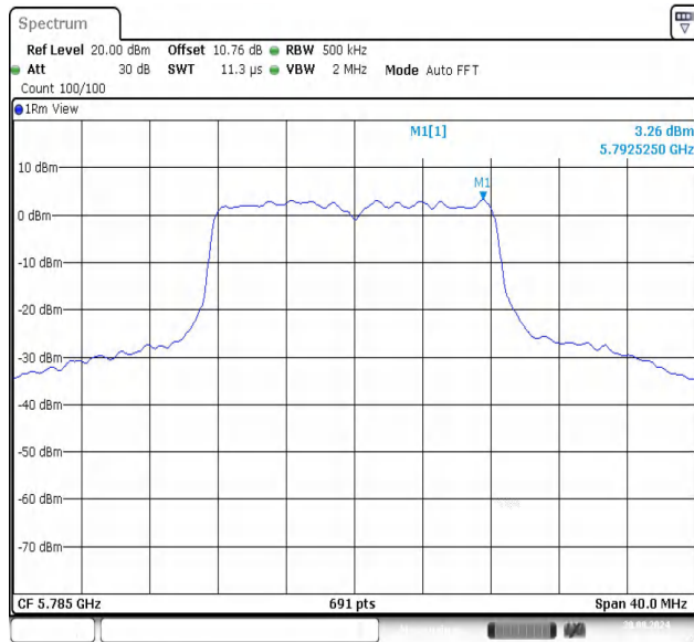
11A-Ant1-5785-PASS
