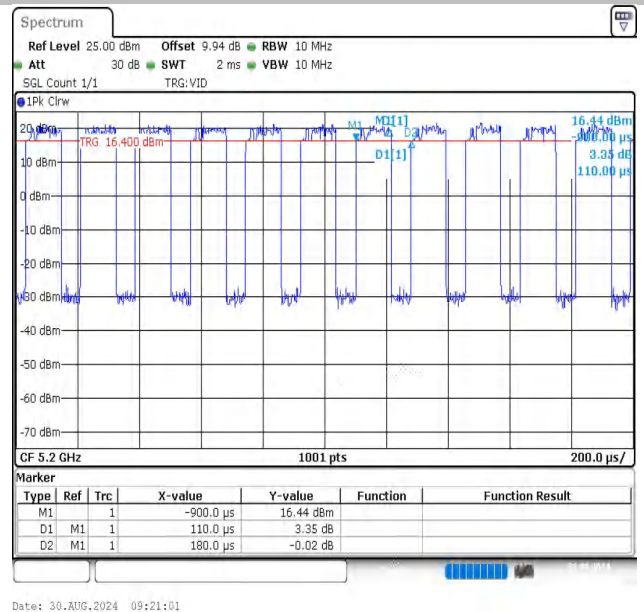
NTNV-11N20SISO-Ant1-5200
