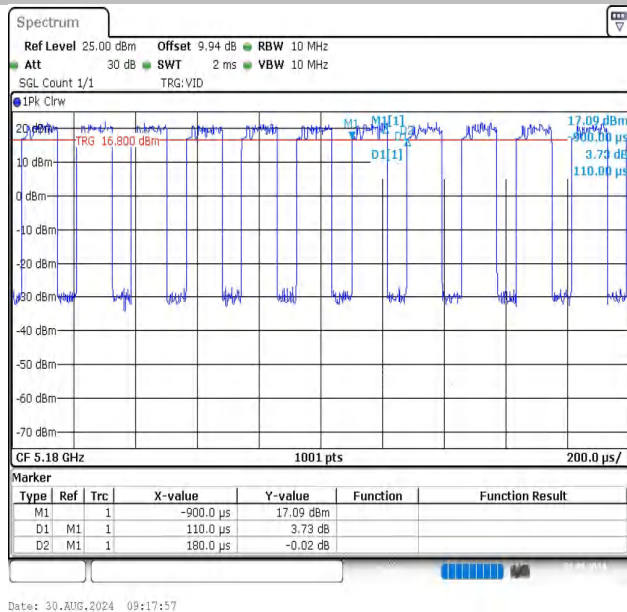
NTNV-11N20SISO-Ant1-5180
