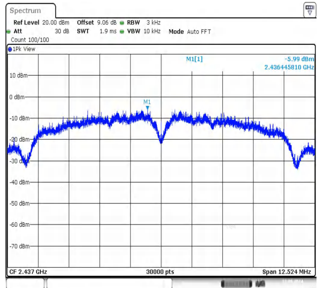
11B-Ant1-2437-PASS
