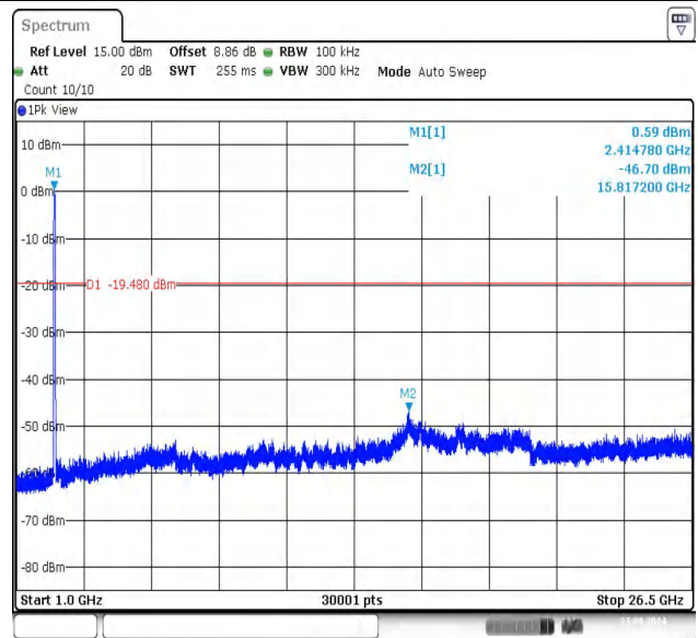
11N40SISO-Ant1-2422-1000~26500-PASS
