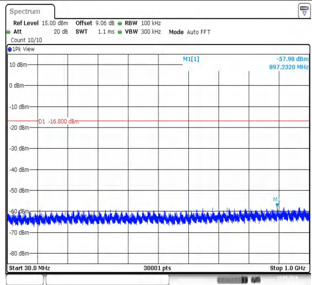
11N20SISO-Ant1-2462-30~1000-PASS
