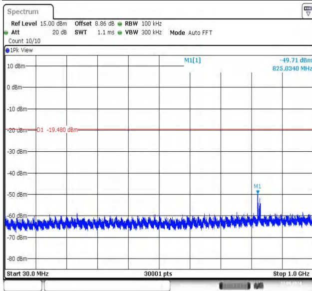
11N40SISO-Ant1-2422-30~1000-PASS
