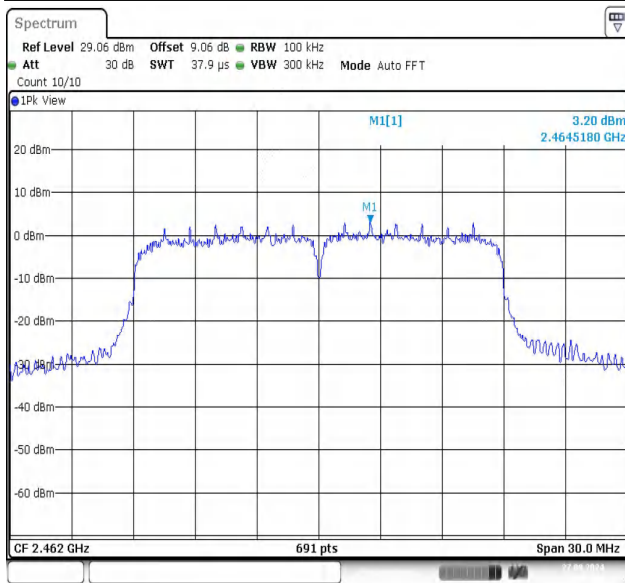
11N20SISO-Ant1-2462-0~Reference-PASS
