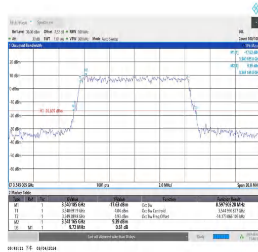
NTNV_N77-3450-3550_PC3_30_10_H_TID3_Ant
