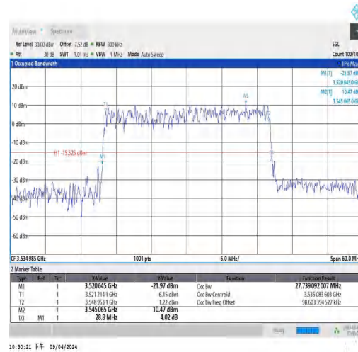
NTNV_N77-3450-3550_PC3_30_30_H_TID3_Ant
