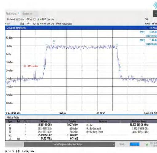
NTNV_N77-3450-3550_PC3_30_15_H_TID5_Ant
