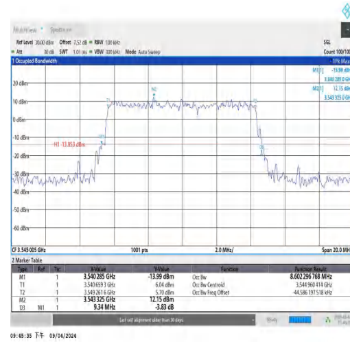
NTNV_N77-3450-3550_PC3_30_10_H_TID1_Ant
