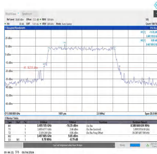
NTNV_N77-3450-3550_PC3_30_10_M_TID5_Ant
