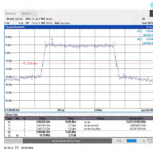
NTNV_N77-3450-3550_PC3_30_15_M_TID3_Ant
