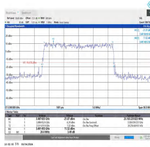
NTNV_N77-3450-3550_PC3_30_25_M_TID5_Ant
