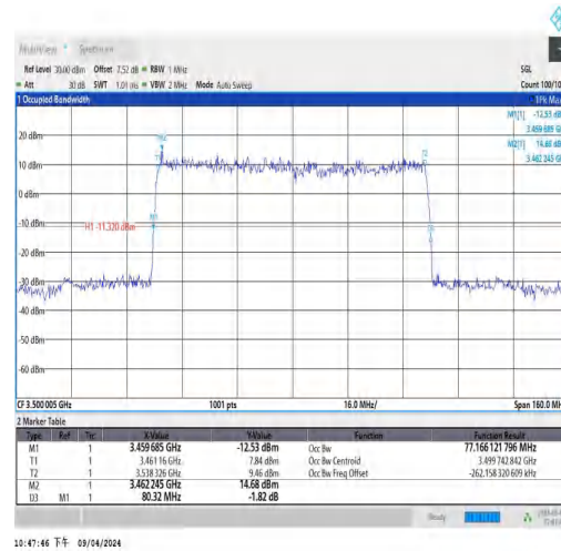
NTNV_N77-3450-3550_PC3_30_80_M_TID1_Ant
