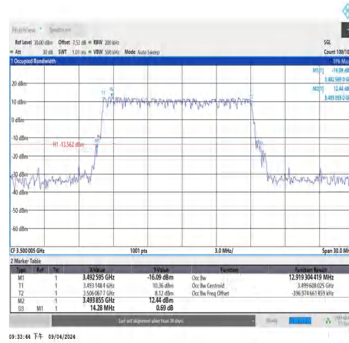
NTNV_N77-3450-3550_PC3_30_15_M_TID1_Ant
