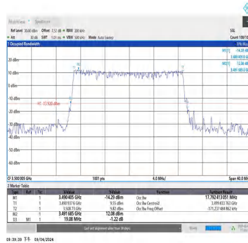
NTNV_N77-3450-3550_PC3_30_20_M_TID1_Ant
