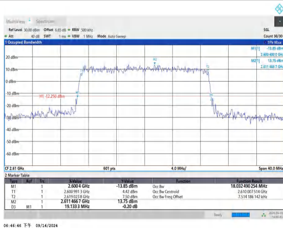
Band38-20MHz-QPSK-38150-100RB#0-PASS
