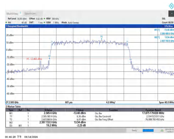
Band38-20MHz-QPSK-38000-100RB#0-PASS
