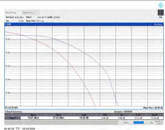
Band38-15MHz-QPSK-38175-75RB#0-PASS
