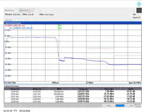
Band38_10MHz_QPSK_38200_50RB#0
