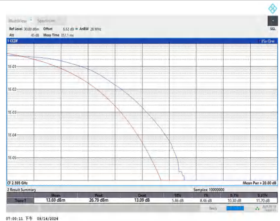
Band38-20MHz-16QAM-38000-100RB#0-PASS
