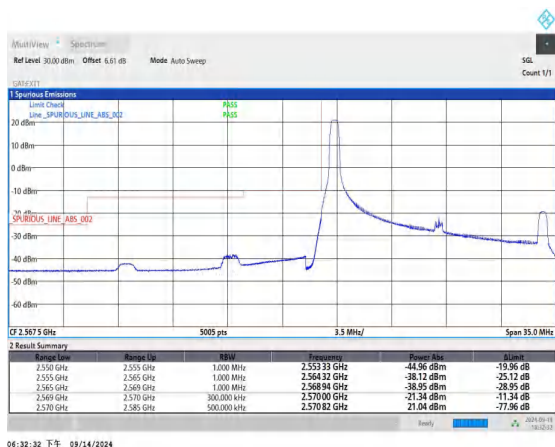
Band38_15MHz_QPSK_37825_1RB#0
