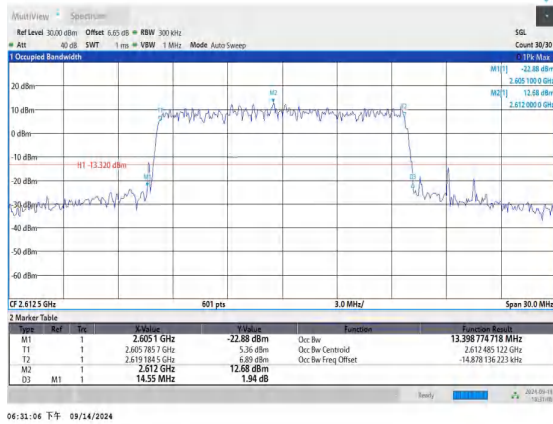
Band38-15MHz-QPSK-38175-75RB#0-PASS
