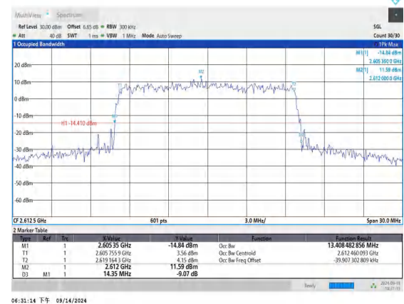
Band38-15MHz-16QAM-38175-75RB#0-PASS
