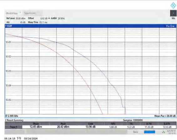
Band38-5MHz-16QAM-38000-25RB#0-PASS
