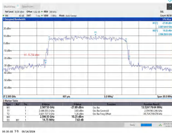
Band38-15MHz-16QAM-38000-75RB#0-PASS
