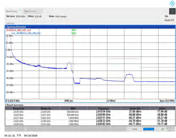
Band38_10MHz_QPSK_38200_1RB#0
