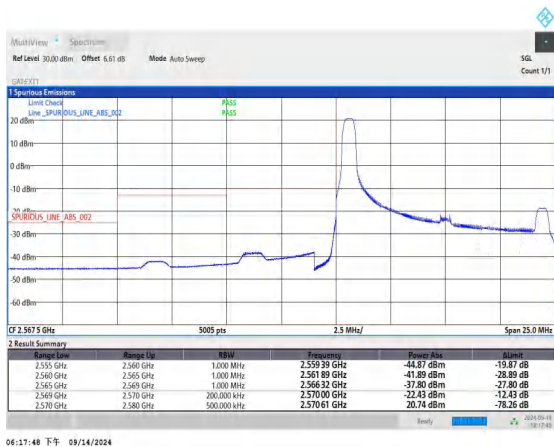
Band38_10MHz_QPSK_37800_1RB#0
