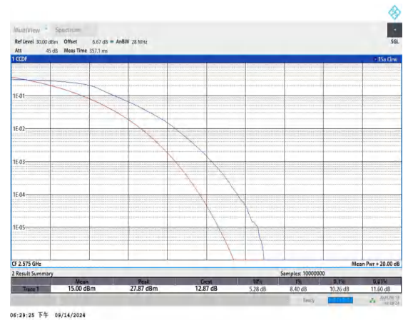
Band38-10MHz-QPSK-37800-50RB#0-PASS
