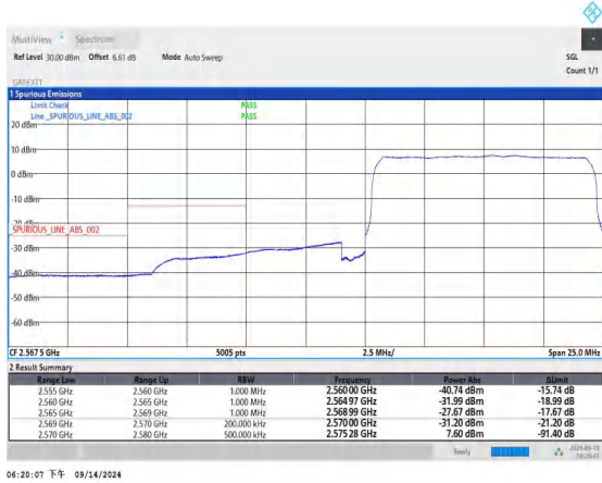
Band38_10MHz_QPSK_37800_50RB#0
