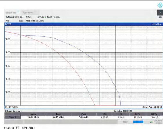
Band38-5MHz-QPSK-38225-25RB#0-PASS
