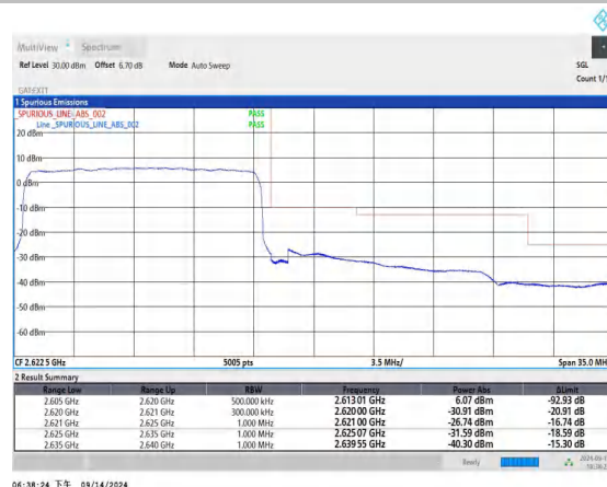
Band38_15MHz_QPSK_38175_75RB#0
