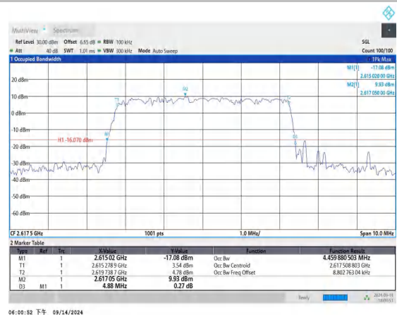
Band38-5MHz-16QAM-38225-25RB#0-PASS
