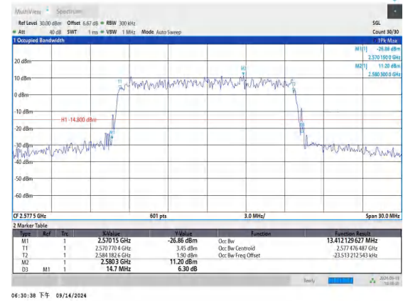
Band38-15MHz-16QAM-37825-75RB#0-PASS
