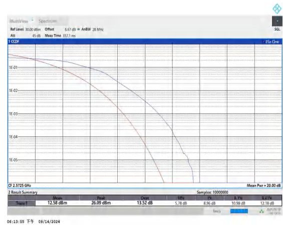
Band38-5MHz-16QAM-37775-25RB#0-PASS
