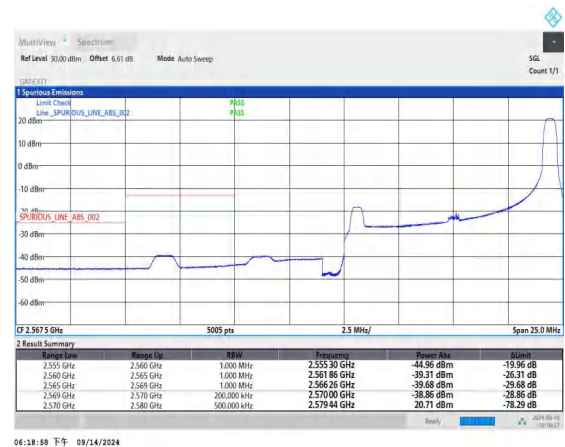
Band38_10MHz_QPSK_37800_1RB#49
