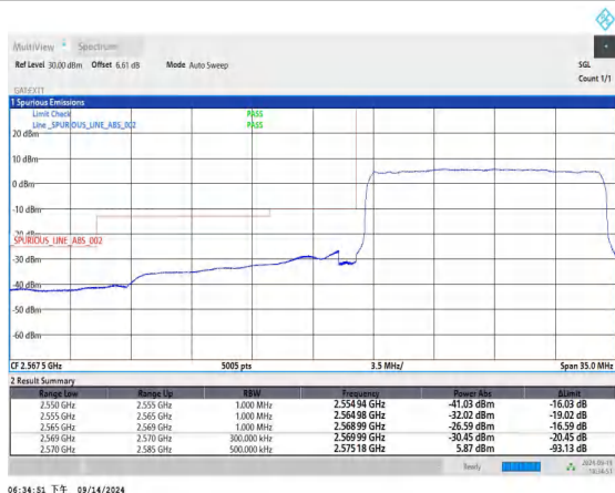
Band38_15MHz_QPSK_37825_75RB#0
