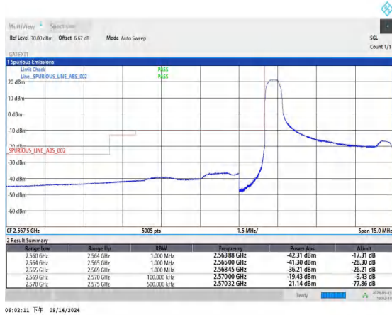
Band38_5MHz_QPSK_37775_1RB#0
