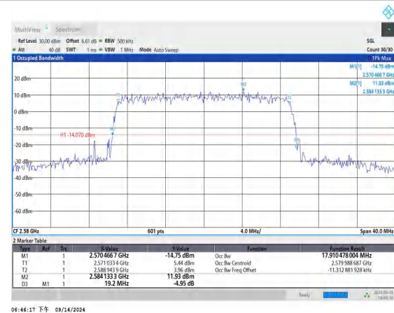
Band38-20MHz-16QAM-37850-100RB#0-PASS
