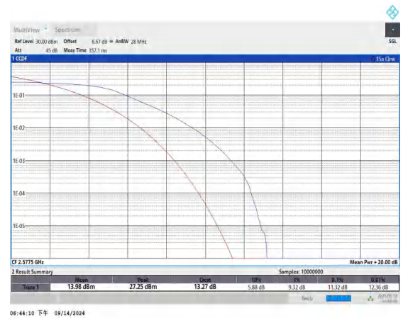
Band38-15MHz-QPSK-37825-75RB#0-PASS
