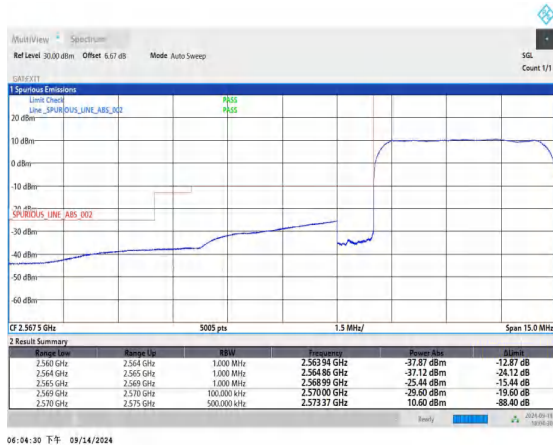
Band38_5MHz_QPSK_37775_25RB#0
