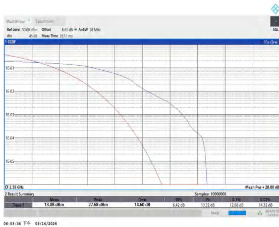
Band38-20MHz-16QAM-37850-1RB#0-PASS
