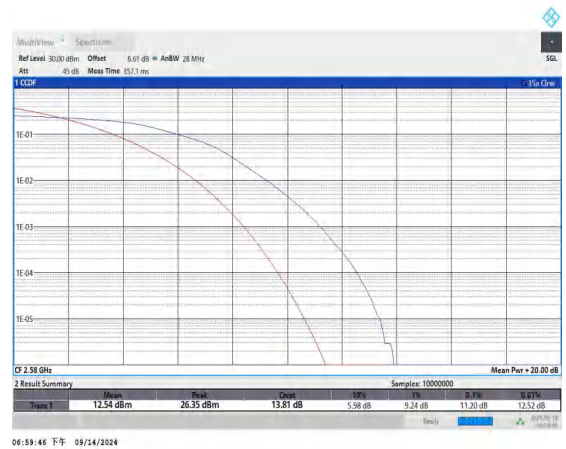
Band38-20MHz-16QAM-37850-100RB#0-PASS
