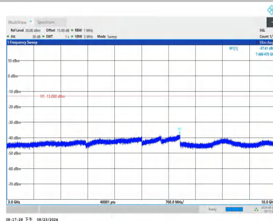
Band26_3MHz_QPSK_27025_1RB#0_3000~10000_3000~1000
