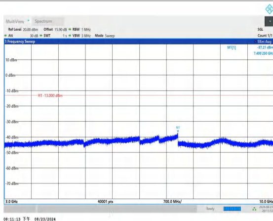
Band26_1.4MHz_QPSK_26797_1RB#0_3000~10000_3000~10000
