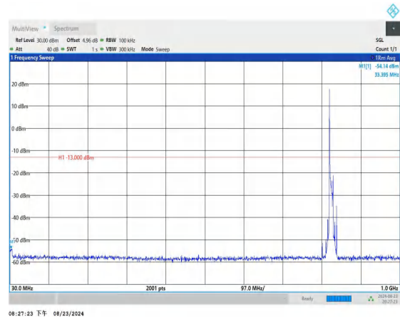
Band26_10MHz_QPSK_26840_1RB#0_30~1000_30~1000
