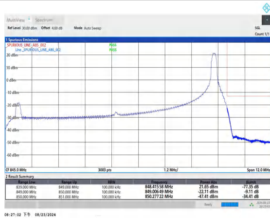
Band26_10MHz_QPSK_26990_1RB#49
