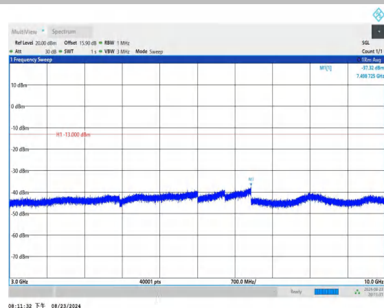
Band26_1.4MHz_QPSK_26915_1RB#0_3000~10000_3000~10000
