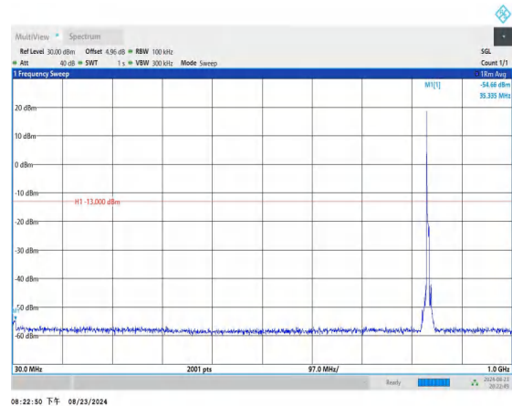
Band26_5MHz_QPSK_26915_1RB#0_30~1000_30~1000
