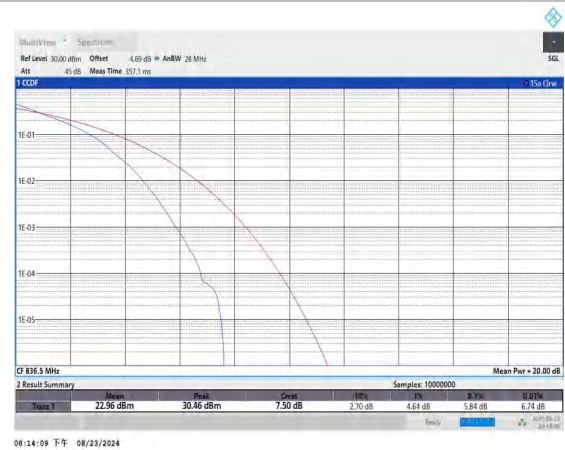
26(824-849)-1.4MHz-QPSK-26915-6RB#0-PASS
