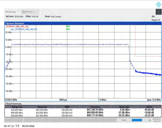
Band26_10MHz_QPSK_26990_50RB#0
