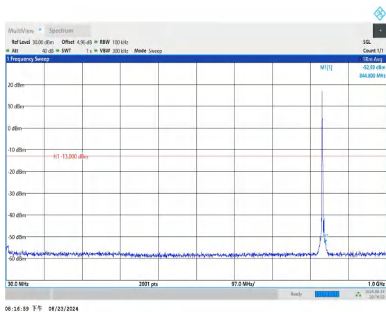
Band26_3MHz_QPSK_26915_1RB#0_30~1000_30~1000
