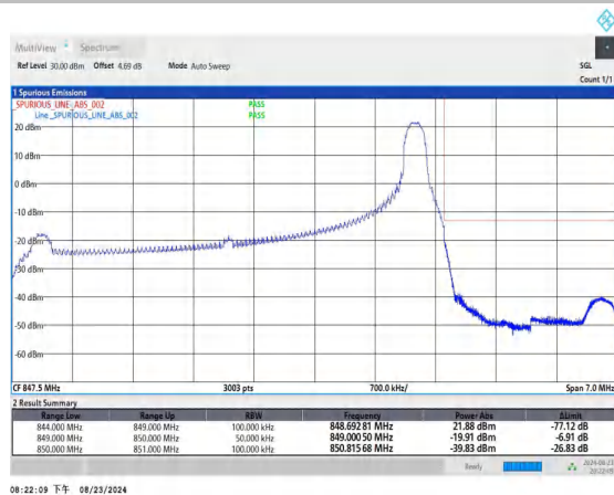
Band26_5MHz_QPSK_27015_1RB#24
