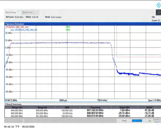
Band26_5MHz_QPSK_27015_25RB#0
