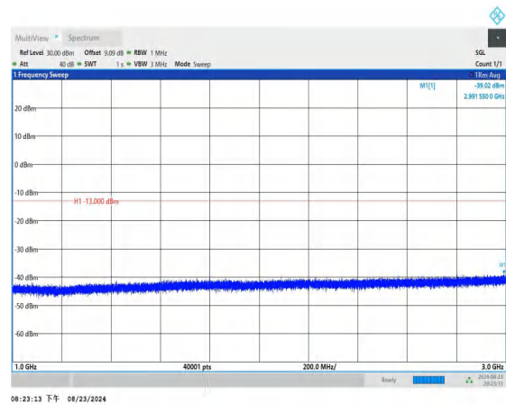
Band26_5MHz_QPSK_27015_1RB#0_1000~3000_1000~3000
