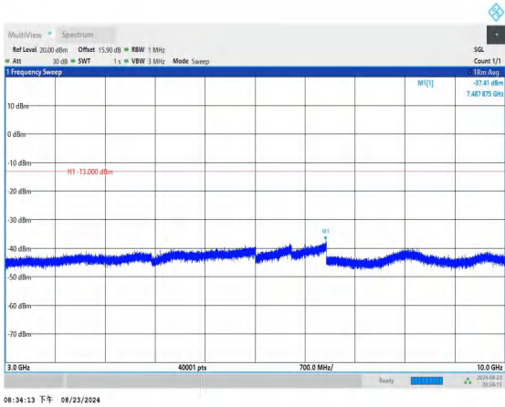
Band26_15MHz_QPSK_26965_1RB#0_3000~10000_3000~100
