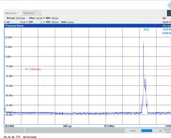
Band26_15MHz_QPSK_26915_1RB#0_30~1000_30~1000
