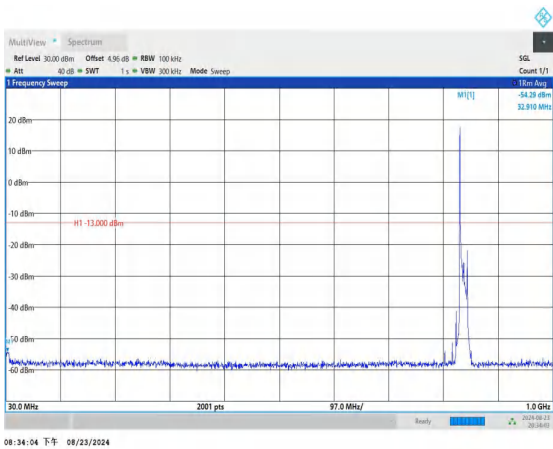
Band26_15MHz_QPSK_26965_1RB#0_30~1000_30~1000
