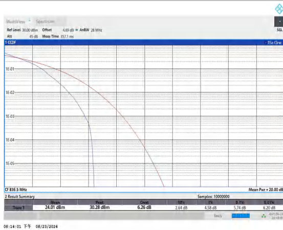
26(824-849)-1.4MHz-QPSK-26915-1RB#0-PASS
