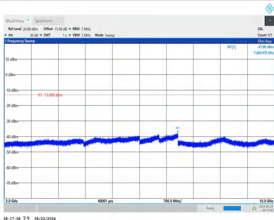
Band26_3MHz_QPSK_26915_1RB#0_3000~10000_3000~1000
