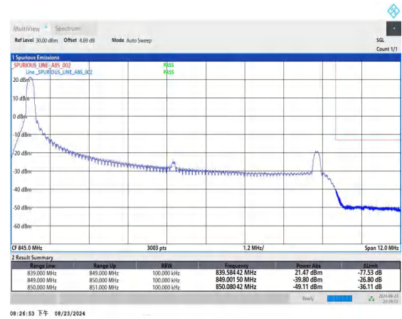
Band26_10MHz_QPSK_26990_1RB#0
