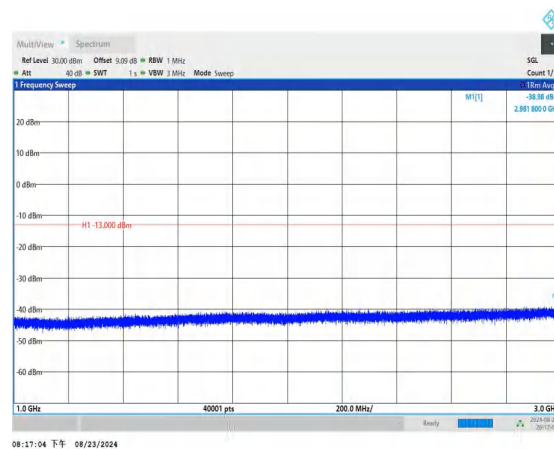
Band26_3MHz_QPSK_26915_1RB#0_1000~3000_1000~3000
