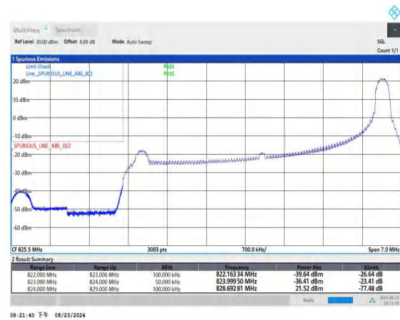
Band26_5MHz_QPSK_26815_1RB#24
