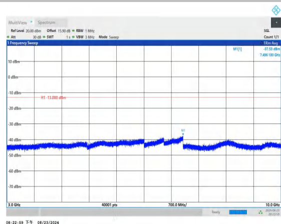
Band26_5MHz_QPSK_26915_1RB#0_3000~10000_3000~1000
