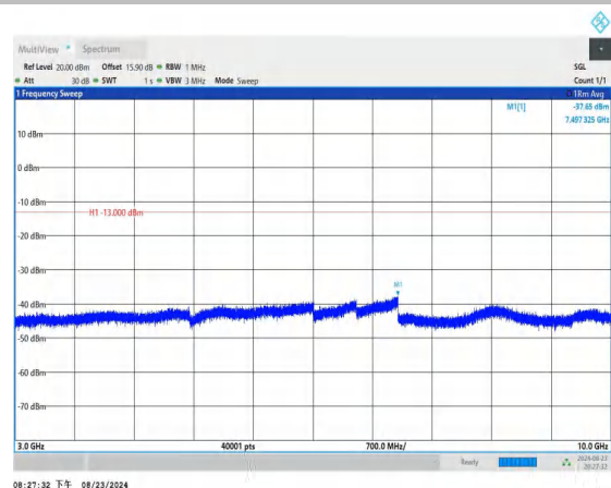
Band26_10MHz_QPSK_26840_1RB#0_3000~10000_3000~1000
