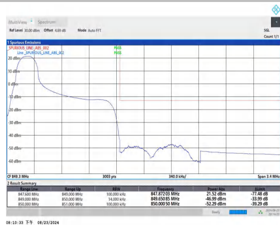
Band26_1.4MHz_QPSK_27033_1RB#0
