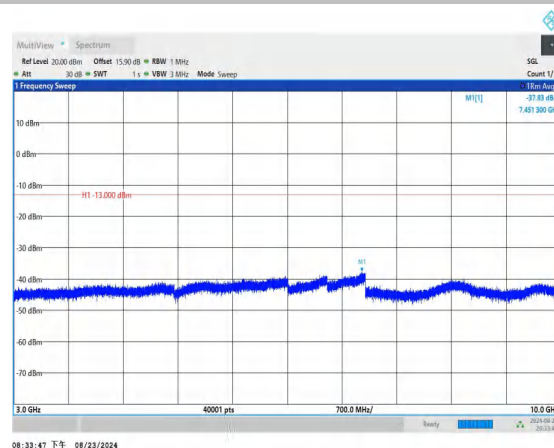
Band26_15MHz_QPSK_26915_1RB#0_3000~10000_3000~10000
