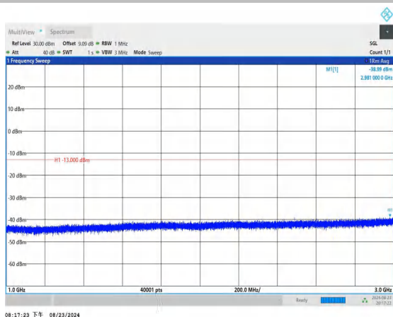
Band26_3MHz_QPSK_27025_1RB#0_1000~3000_1000~3000
