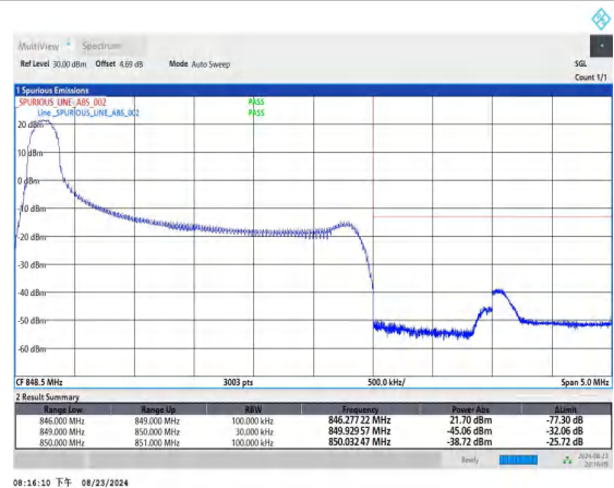
Band26_3MHz_QPSK_27025_1RB#0
