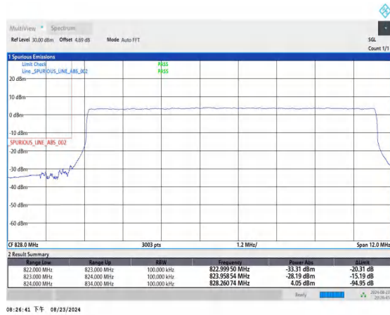
Band26_10MHz_QPSK_26840_50RB#0
