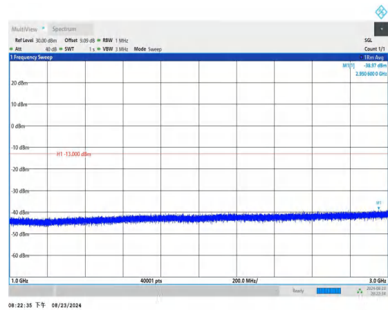
Band26_5MHz_QPSK_26815_1RB#0_1000~3000_1000~3000
