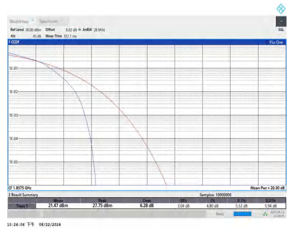
Band25-15MHz-16QAM-26115-75RB#0-PASS
