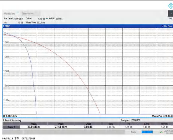
Band25-3MHz-QPSK-26675-1RB#0-PASS
