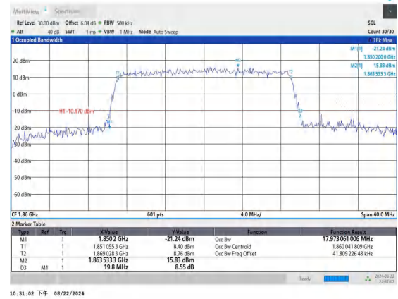
Band25-20MHz-16QAM-26140-100RB#0-PASS
