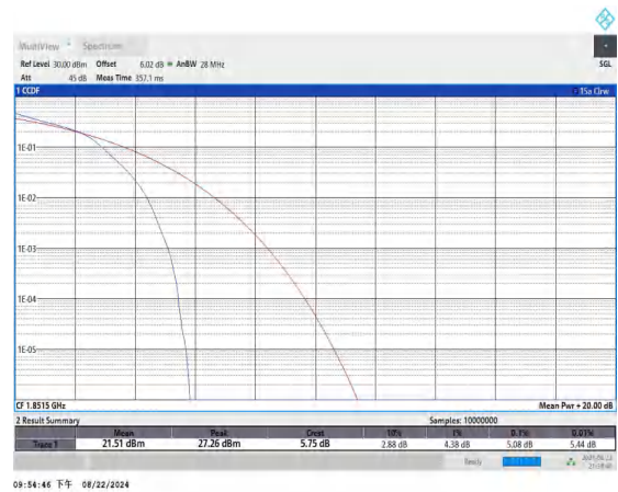
Band25-3MHz-16QAM-26055-15RB#0-PASS
