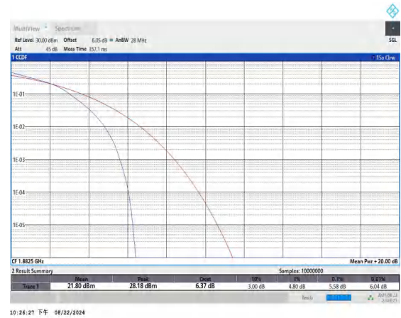
Band25-15MHz-16QAM-26365-75RB#0-PASS
