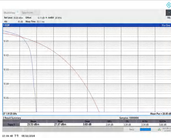
Band25-5MHz-16QAM-26665-1RB#0-PASS
