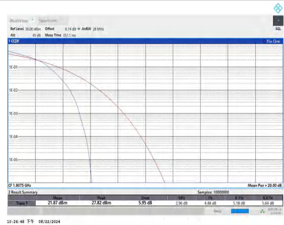
Band25-15MHz-16QAM-26615-75RB#0-PASS
