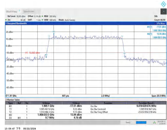
Band25-10MHz-16QAM-26640-50RB#0-PASS
