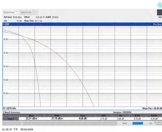
Band25-15MHz-16QAM-26115-1RB#0-PASS
