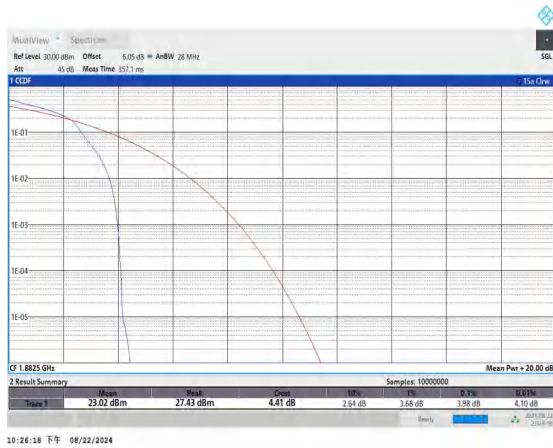
Band25-15MHz-16QAM-26365-1RB#0-PASS
