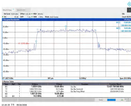
Band25-15MHz-QPSK-26115-75RB#0-PASS
