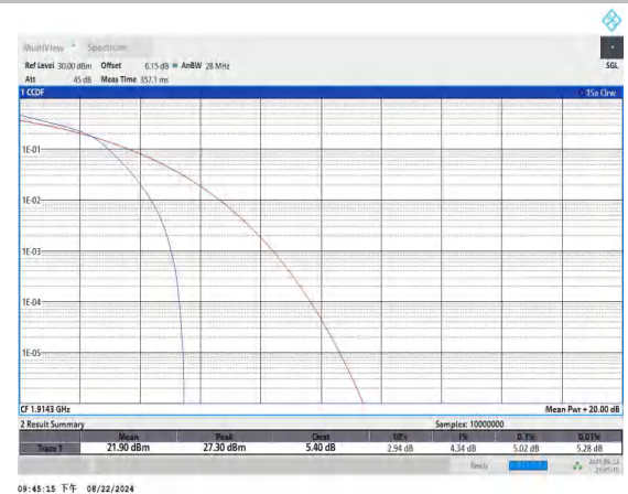
Band25-1.4MHz-16QAM-26683-6RB#0-PASS
