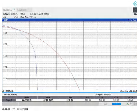
Band25-5MHz-16QAM-26365-1RB#0-PASS
