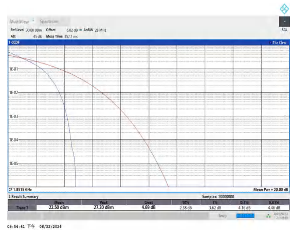
Band25-3MHz-QPSK-26055-15RB#0-PASS
