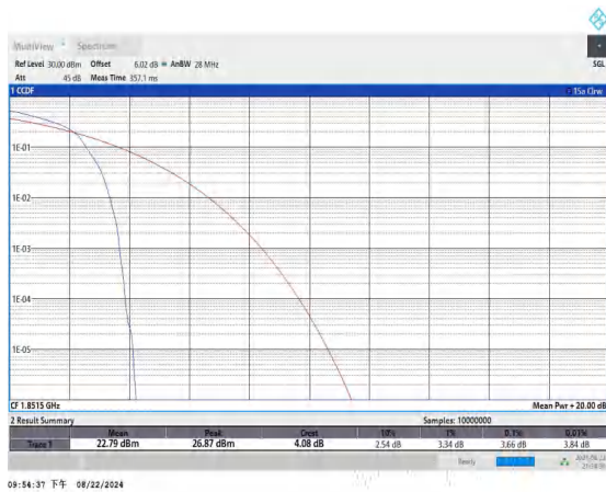
Band25-3MHz-16QAM-26055-1RB#0-PASS
