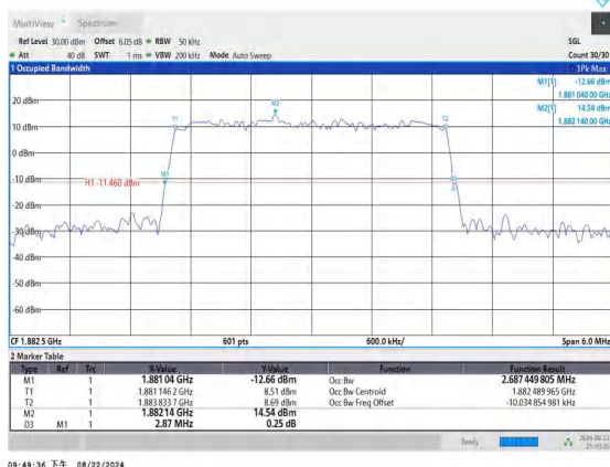
Band25-3MHz-16QAM-26365-15RB#0-PASS
