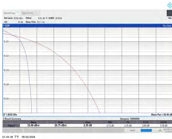
Band25-5MHz-QPSK-26065-1RB#0-PASS
