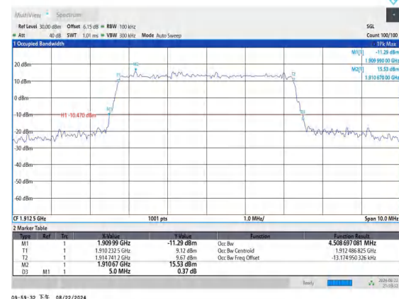
Band25-5MHz-16QAM-26665-25RB#0-PASS
