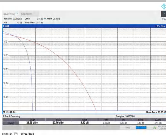
Band25-1.4MHz-QPSK-26683-1RB#0-PASS
