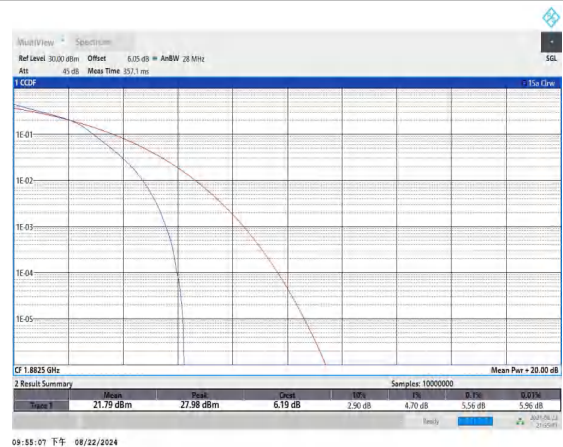
Band25-3MHz-16QAM-26365-15RB#0-PASS
