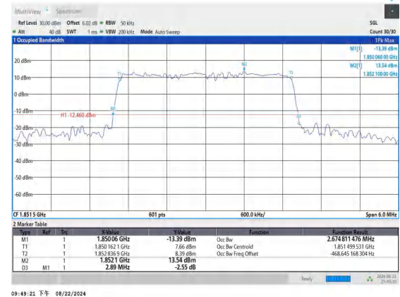
Band25-3MHz-16QAM-26055-15RB#0-PASS
