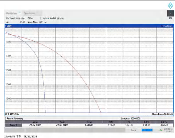
Band25-5MHz-QPSK-26665-25RB#0-PASS
