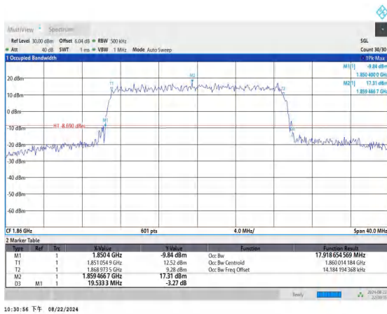
Band25-20MHz-QPSK-26140-100RB#0-PASS
