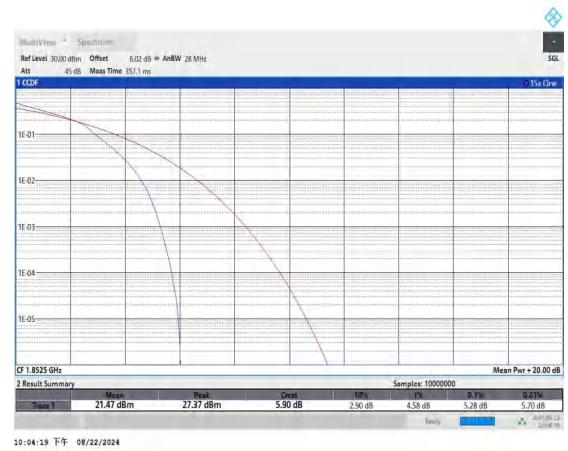
Band25-5MHz-16QAM-26065-25RB#0-PASS
