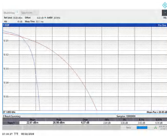
Band25-10MHz-16QAM-26090-1RB#0-PASS
