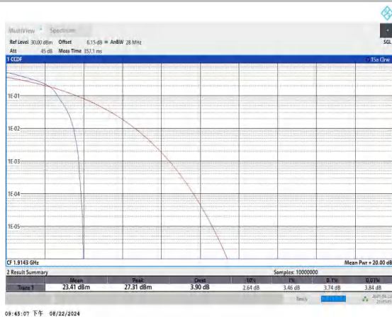
Band25-1.4MHz-16QAM-26683-1RB#0-PASS
