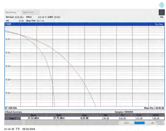
Band25-10MHz-16QAM-26090-50RB#0-PASS
