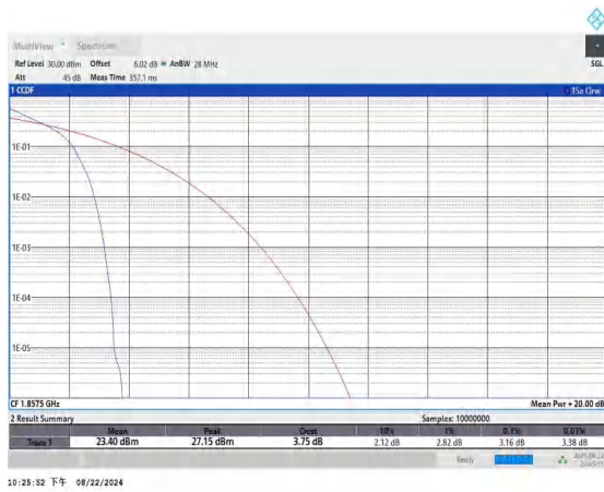
Band25-15MHz-QPSK-26115-1RB#0-PASS
