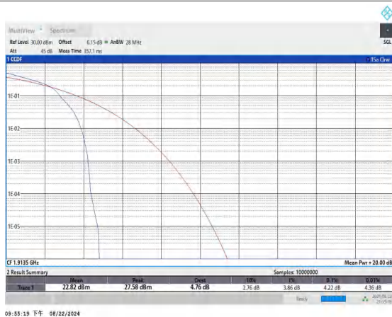
Band25-3MHz-16QAM-26675-1RB#0-PASS
