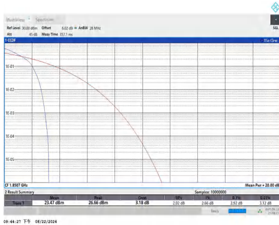
Band25-1.4MHz-QPSK-26047-1RB#0-PASS
