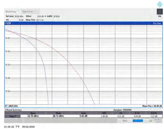
Band25-15MHz-QPSK-26365-75RB#0-PASS
