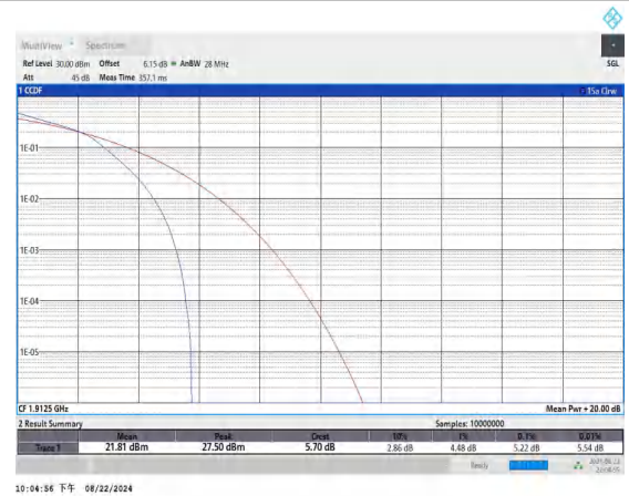
Band25-5MHz-16QAM-26665-25RB#0-PASS
