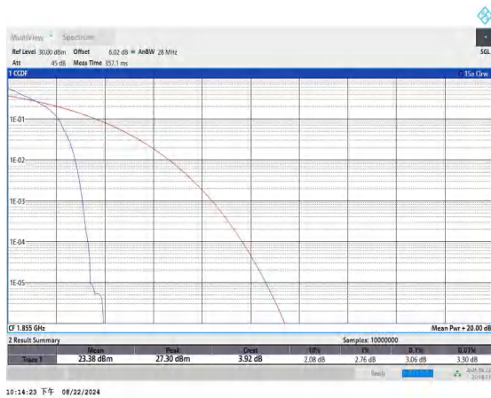
Band25-10MHz-QPSK-26090-1RB#0-PASS
