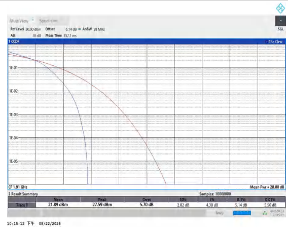
Band25-10MHz-16QAM-26640-50RB#0-PASS
