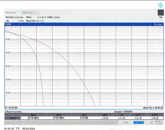
Band25-3MHz-QPSK-26675-15RB#0-PASS
