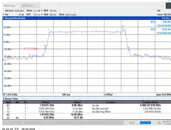
Band25-5MHz-QPSK-26665-25RB#0-PASS
