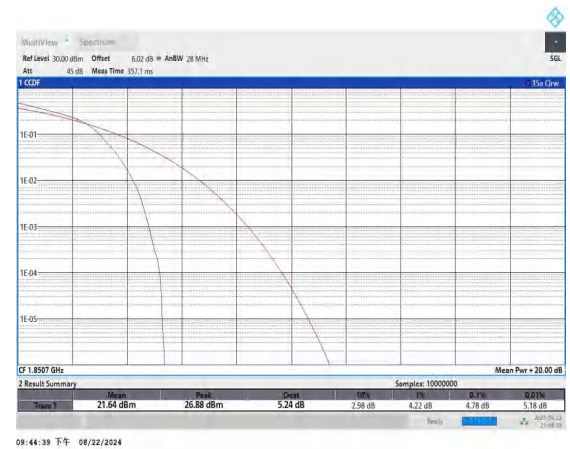
Band25-1.4MHz-16QAM-26047-6RB#0-PASS
