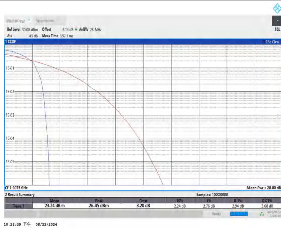
Band25-15MHz-16QAM-26615-1RB#0-PASS
