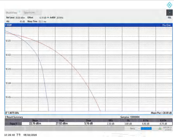
Band25-15MHz-QPSK-26615-75RB#0-PASS
