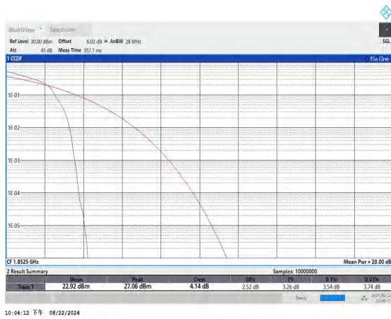
Band25-5MHz-16QAM-26065-1RB#0-PASS
