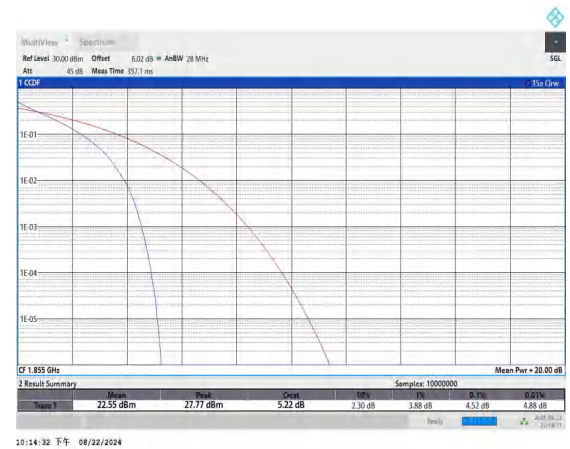
Band25-10MHz-QPSK-26090-50RB#0-PASS
