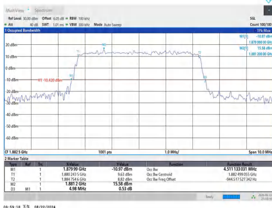
Band25-5MHz-16QAM-26365-25RB#0-PASS
