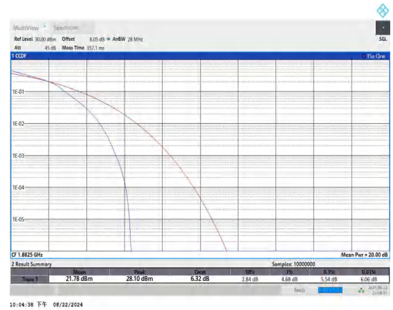
Band25-5MHz-16QAM-26365-25RB#0-PASS
