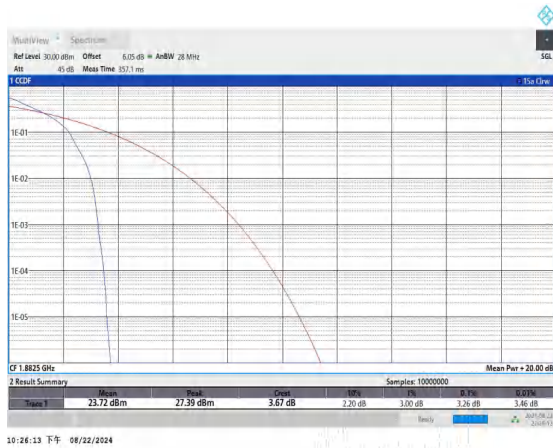
Band25-15MHz-QPSK-26365-1RB#0-PASS
