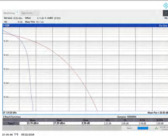
Band25-5MHz-QPSK-26665-1RB#0-PASS
