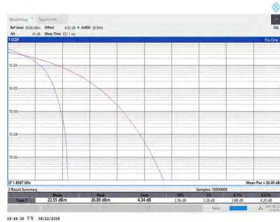
Band25-1.4MHz-QPSK-26047-6RB#0-PASS
