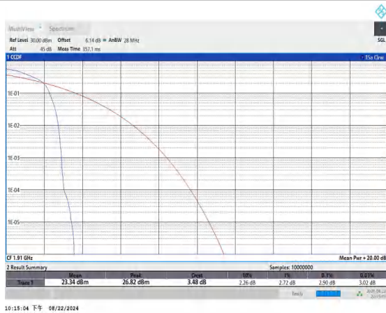
Band25-10MHz-16QAM-26640-1RB#0-PASS
