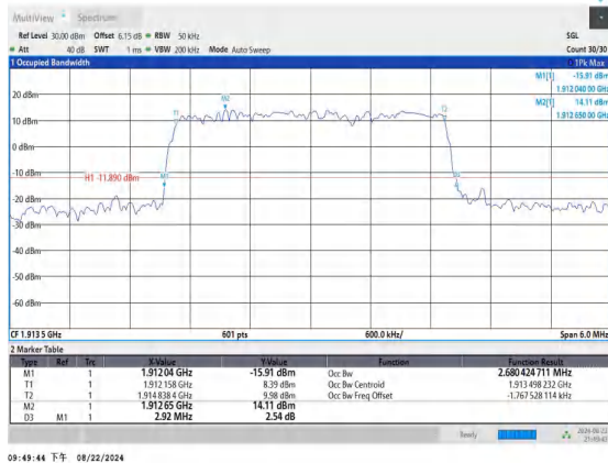
Band25-3MHz-QPSK-26675-15RB#0-PASS
