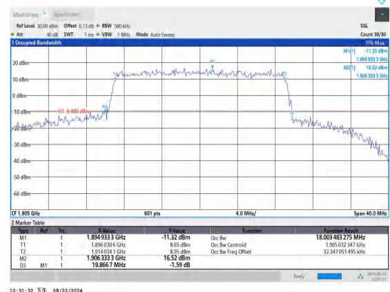
Band25-20MHz-16QAM-26590-100RB#0-PASS
