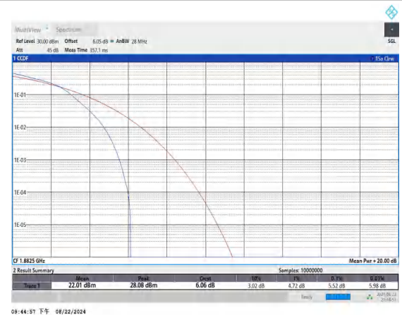
Band25-1.4MHz-16QAM-26365-6RB#0-PASS
