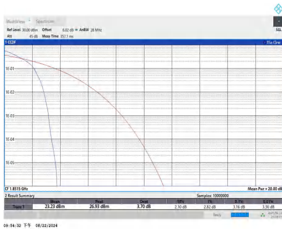
Band25-3MHz-QPSK-26055-1RB#0-PASS
