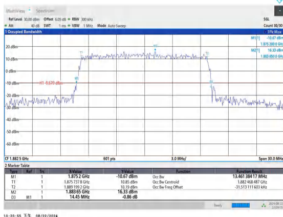
Band25-15MHz-16QAM-26365-75RB#0-PASS
