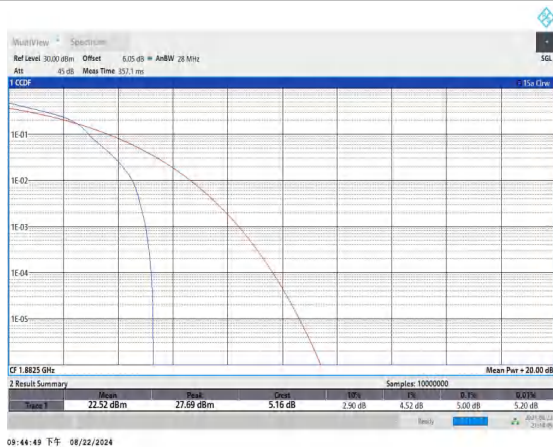
Band25-1.4MHz-16QAM-26365-1RB#0-PASS
