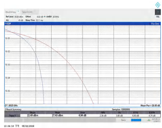
Band25-5MHz-QPSK-26065-25RB#0-PASS
