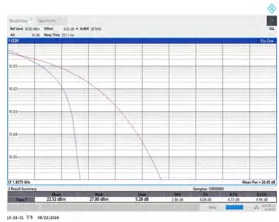
Band25-15MHz-QPSK-26115-75RB#0-PASS
