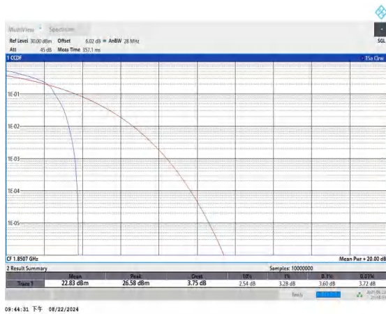
Band25-1.4MHz-16QAM-26047-1RB#0-PASS
