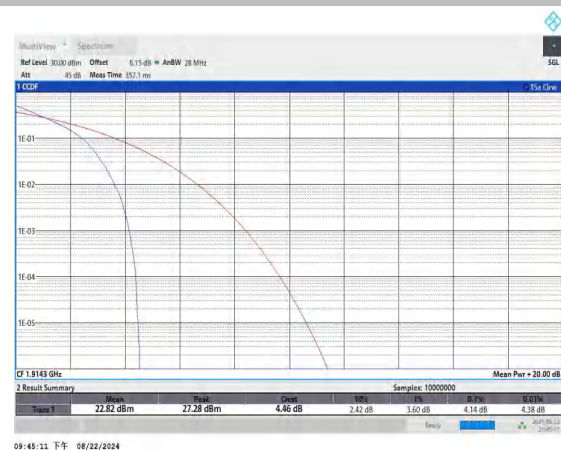
Band25-1.4MHz-QPSK-26683-6RB#0-PASS
