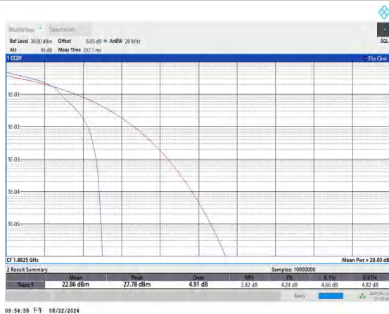
Band25-3MHz-16QAM-26365-1RB#0-PASS
