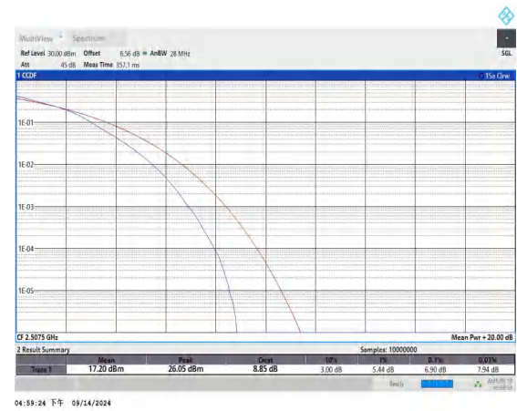
Band7-15MHz-16QAM-20825-75RB#0-PASS
