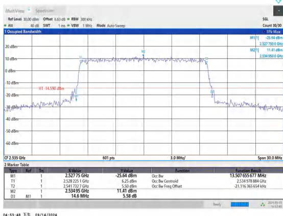
Band7-15MHz-16QAM-21100-75RB#0-PASS
