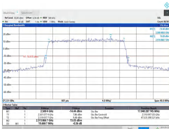
Band7-20MHz-QPSK-20850-100RB#0-PASS
