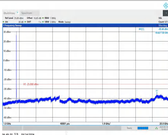
Band7_10MHz_QPSK_21400_1RB#0_1000~20000_1000~2000
