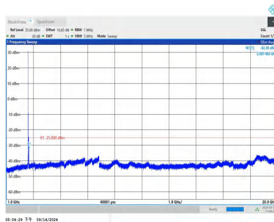
Band7_20MHz_QPSK_21100_1RB#0_1000~20000_1000~2000
