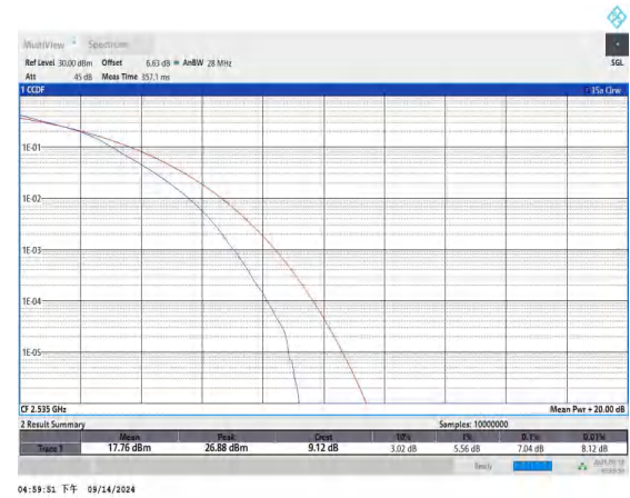
Band7-15MHz-16QAM-21100-75RB#0-PASS
