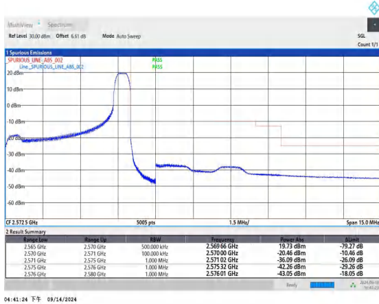
Band7_5MHz_16QAM_21425_1RB#24
