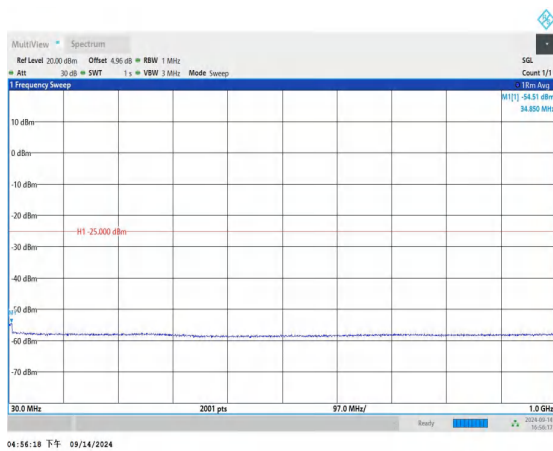
Band7_15MHz_QPSK_20825_1RB#0_30~1000_30~1000
