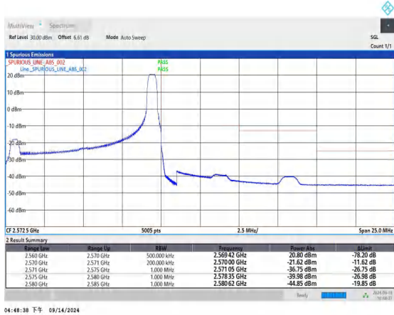
Band7_10MHz_QPSK_21400_1RB#49
