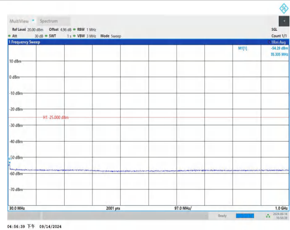
Band7_15MHz_QPSK_21100_1RB#0_30~1000_30~1000
