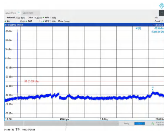
Band7_10MHz_QPSK_21100_1RB#0_1000~20000_1000~2000
