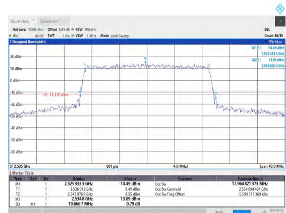
Band7-20MHz-QPSK-21100-100RB#0-PASS
