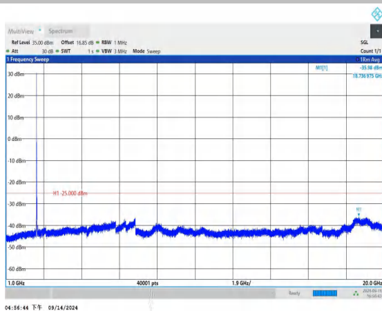
Band7_15MHz_QPSK_21100_1RB#0_1000~20000_1000~2000
