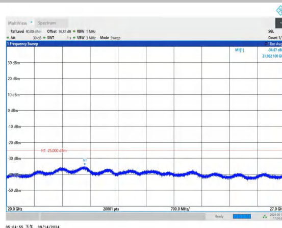
Band7_20MHz_QPSK_21350_1RB#0_20000~27000_20000~27000
