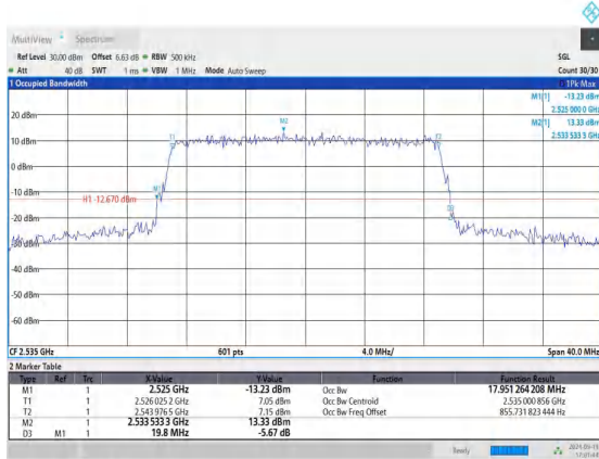
Band7-20MHz-16QAM-21100-100RB#0-PASS
