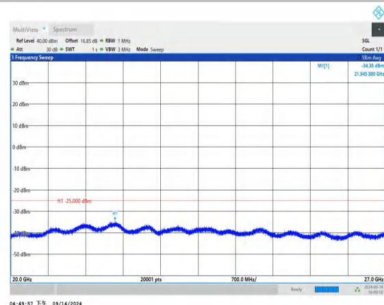
Band7_10MHz_QPSK_21400_1RB#0_20000~27000_20000~27000
