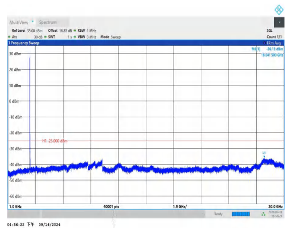
Band7_15MHz_QPSK_20825_1RB#0_1000~20000_1000~2000
