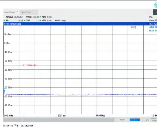
Band7_20MHz_QPSK_21350_1RB#0_30~1000_30~1000
