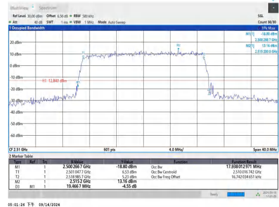
Band7-20MHz-16QAM-20850-100RB#0-PASS
