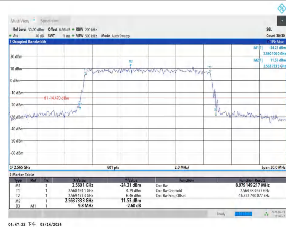
Band7-10MHz-16QAM-21400-50RB#0-PASS
