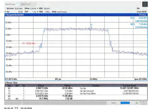
Band7-15MHz-16QAM-20825-75RB#0-PASS
