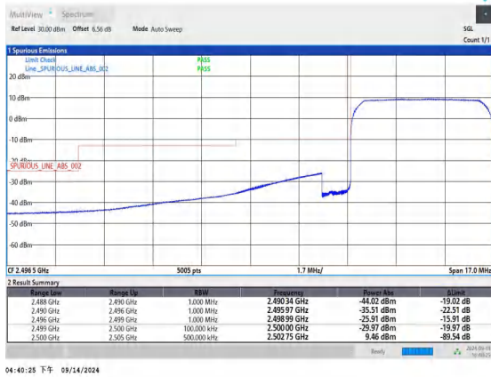
Band7_5MHz_16QAM_20775_25RB#0
