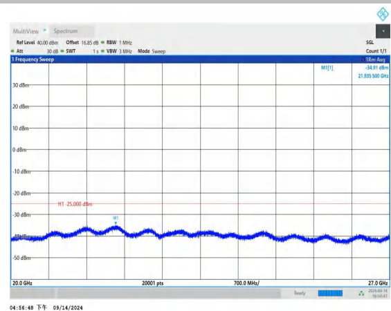
Band7_15MHz_QPSK_21100_1RB#0_20000~27000_20000~27
