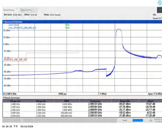
Band7_5MHz_QPSK_20775_1RB#0
