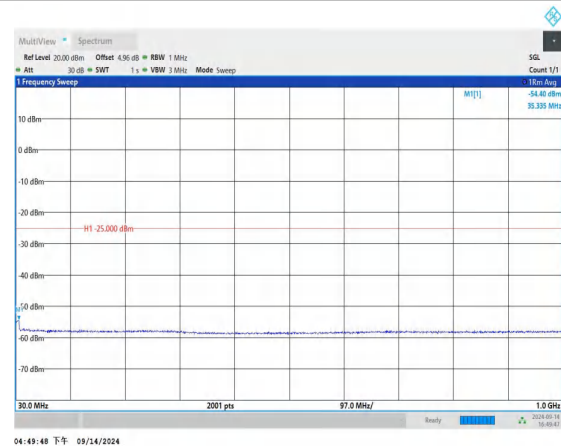
Band7_10MHz_QPSK_21400_1RB#0_30~1000_30~1000
