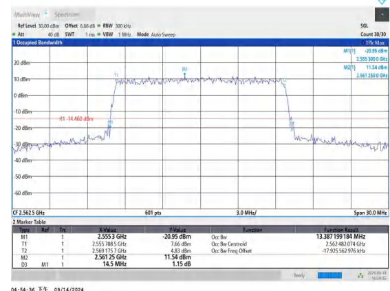
Band7-15MHz-16QAM-21375-75RB#0-PASS
