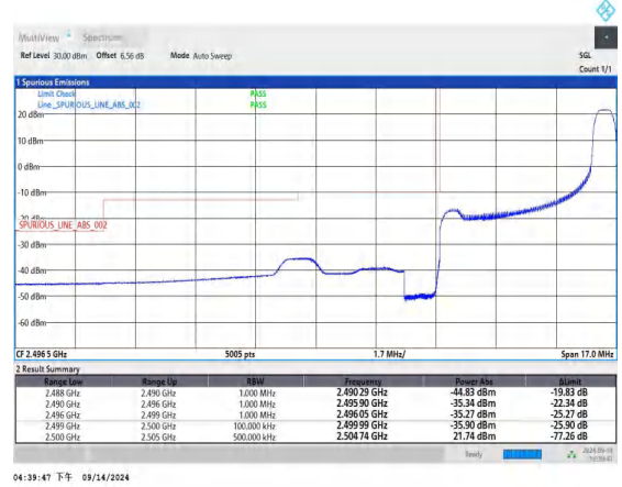
Band7_5MHz_QPSK_20775_1RB#24
