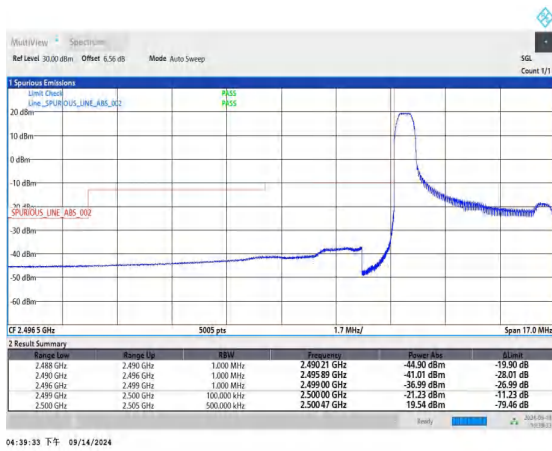
Band7_5MHz_16QAM_20775_1RB#0
