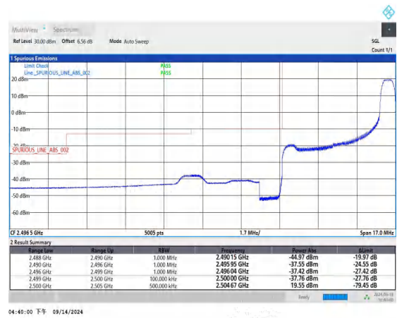
Band7_5MHz_16QAM_20775_1RB#24
