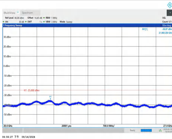
Band7_15MHz_QPSK_20825_1RB#0_20000~27000_20000~27
