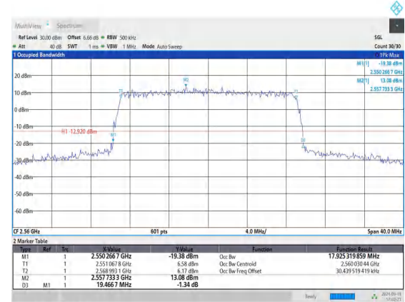
Band7-20MHz-16QAM-21350-100RB#0-PASS
