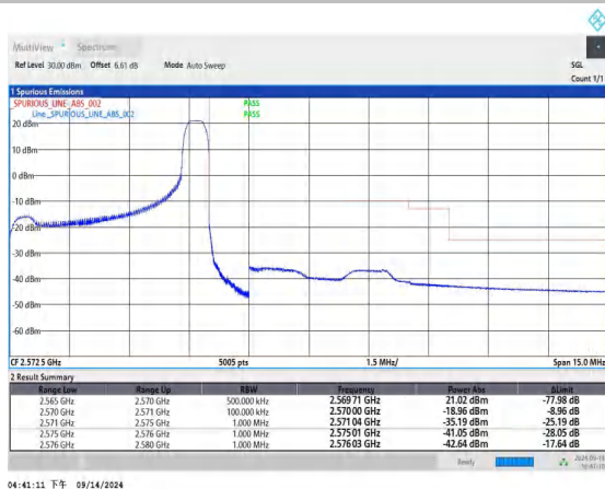
Band7_5MHz_QPSK_21425_1RB#24
